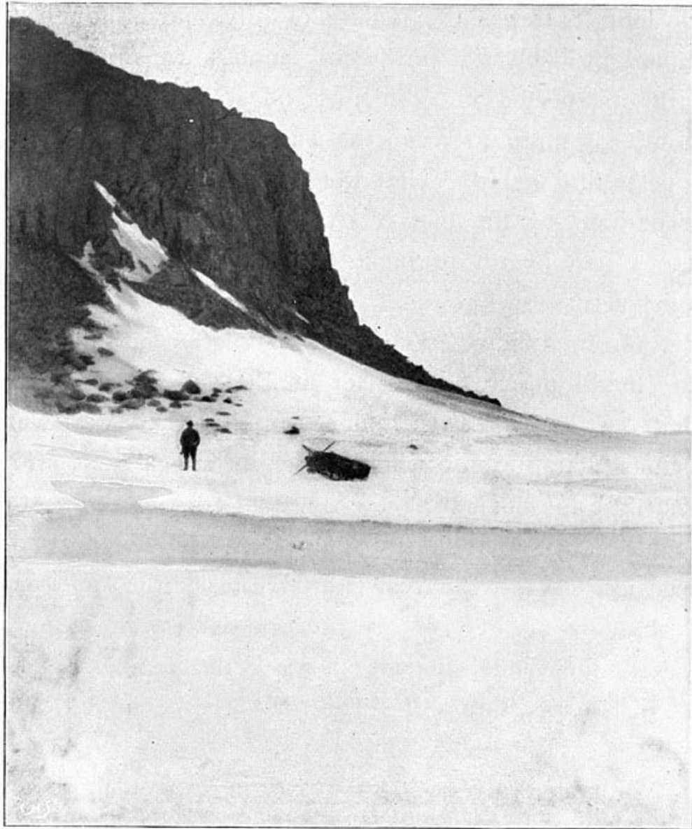
Basaltic Cliffs
