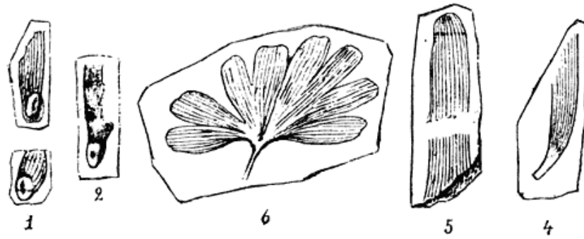
Plant Fossils
