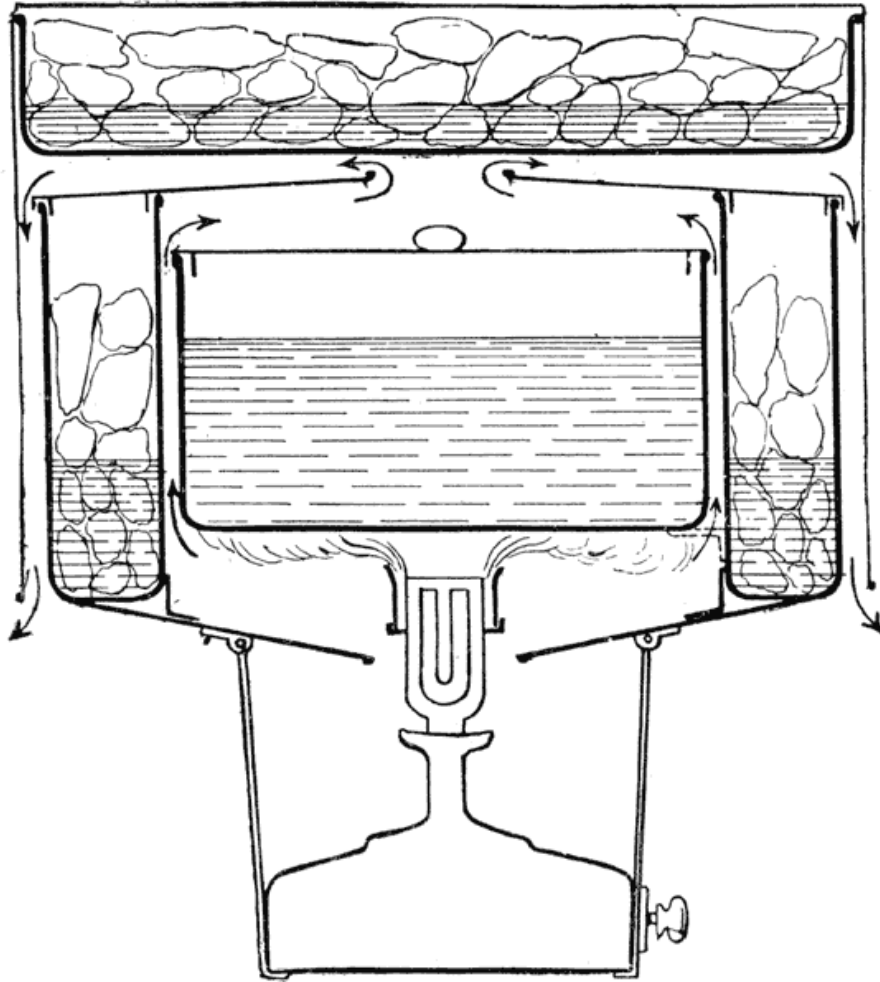
The Cooking Apparatus
