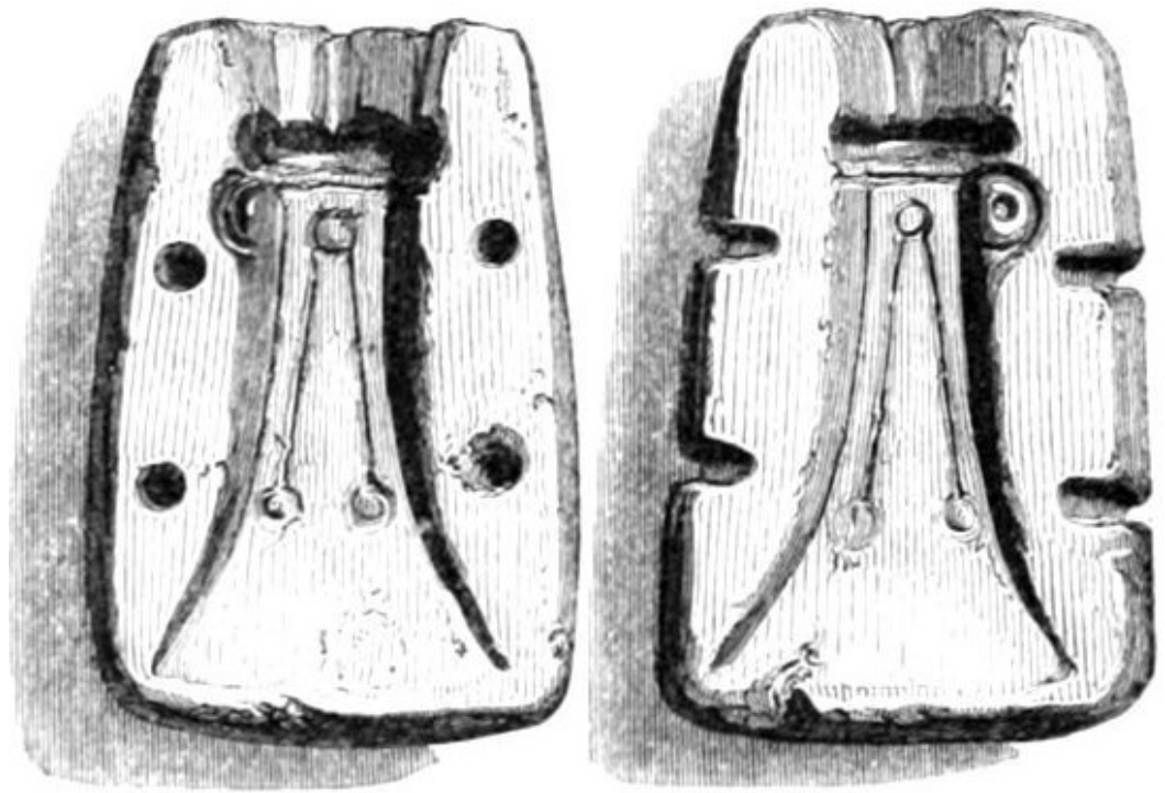
Celt-Moulds, Ross-shire.
