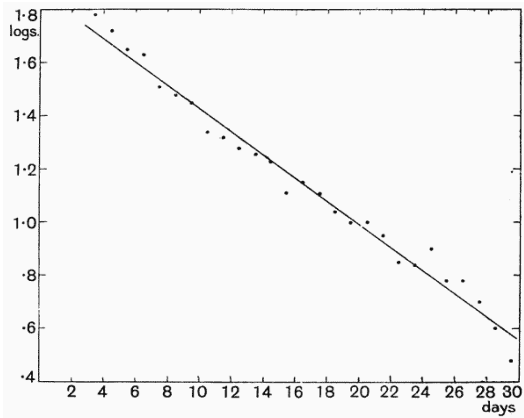
Fig. 37. Logarithms of values shewn in Fig. 36 .
