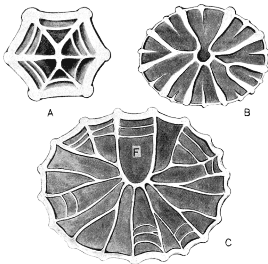
Fig. 174. Heterophyllia sp. (After Martin Duncan.)
