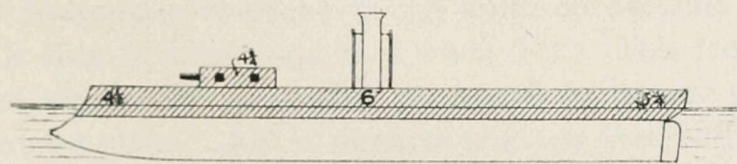
FRENCH RAM TAUREAU (1865)
