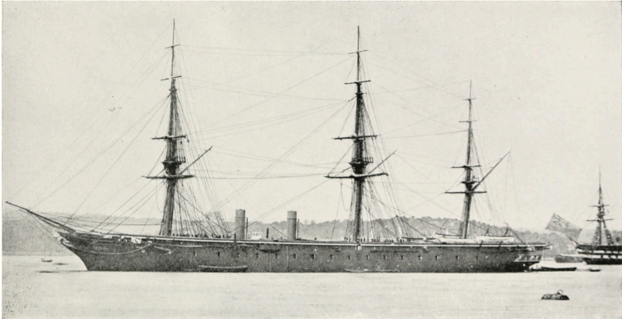
THE WARRIOR, AS COMPLETED, 1861.
