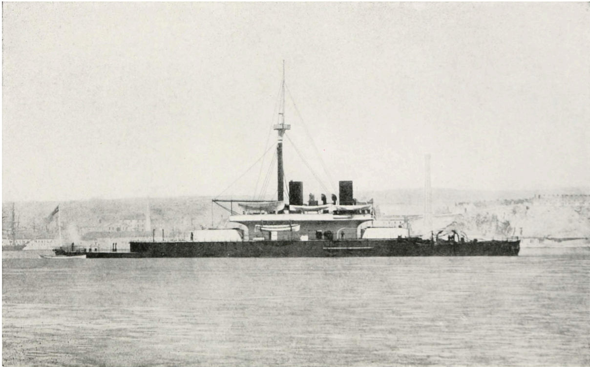
THE DEVASTATION , AS COMPLETED, 1873.
