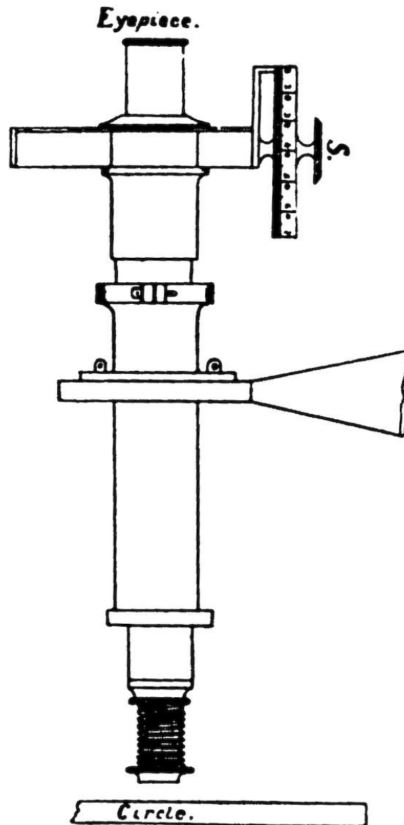
FIG. 48.— The Reading Microscope.
