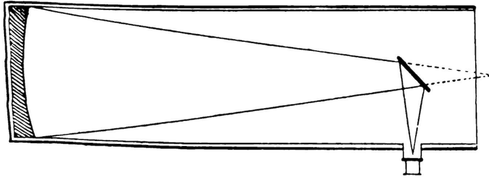
FIG. 50.— The Newtonian Reflector.
