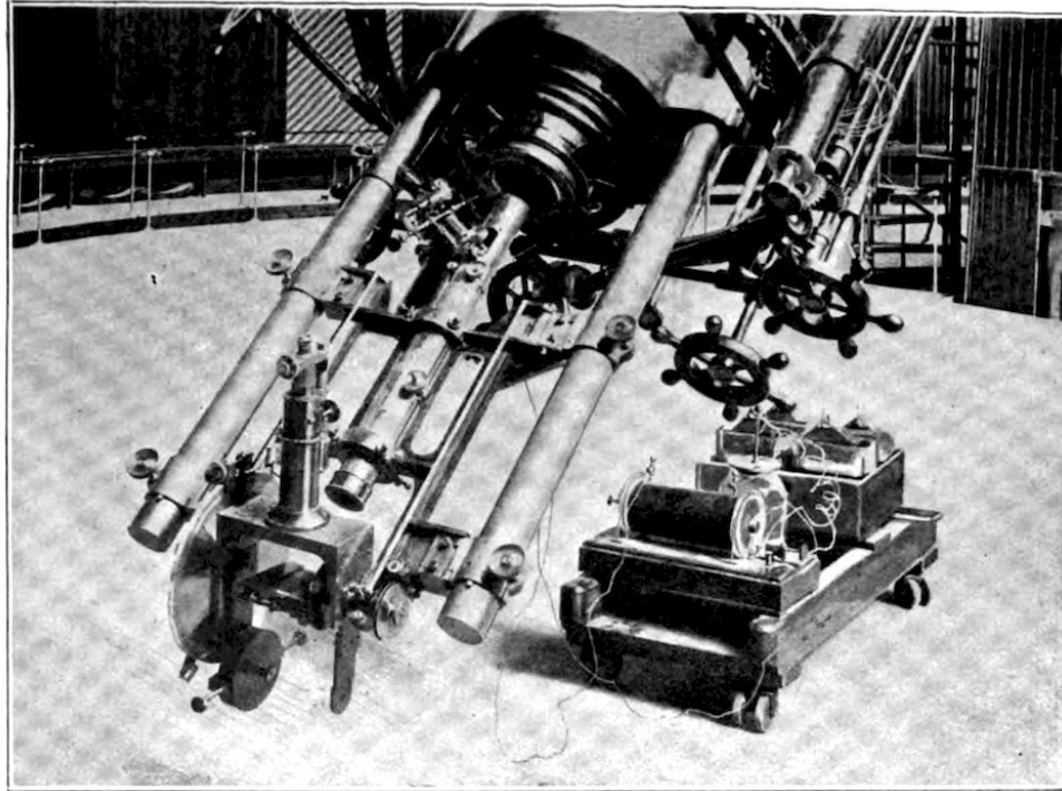
FIG. 55.—The Spectroscope adapted to the Eye End of the Lick Telescope.
