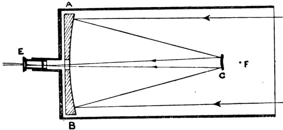
FIG. 51.— The Cassegrain Reflector.
