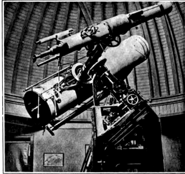
FIG. 52.— The Photographic Telescope employed by Dr. Isaac Roberts.
