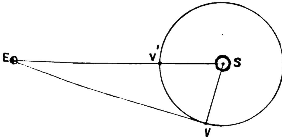
FIG. 41.— Relative Distance of Venus.
