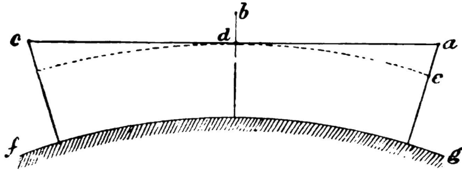
FIG. 1.— Rough Measurement of Earth's Diameter.
