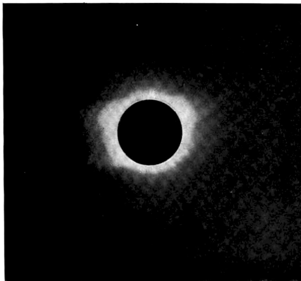
FIG. 7.— The Corona of January 1, 1889, photographed by Professor E. E. Barnard.
