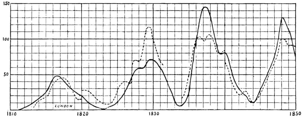
FIG. 2.— Sun-spots and Magnetic Variations. (From Langley's "New Astronomy.")
