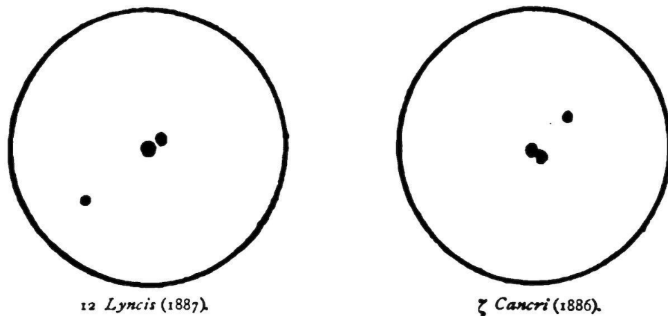
FIG. 7.—Triple Stars.
