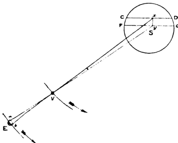
FIG. 43.— The Transit of Venus.
