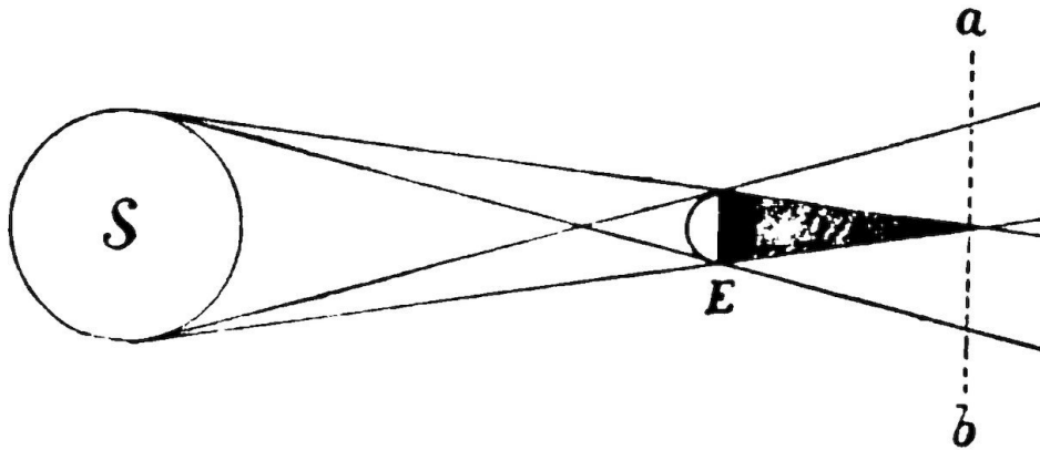
FIG. 29.— The Earth's Shadow.
