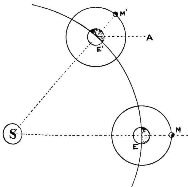
FIG. 19.—The Lunar Month.
