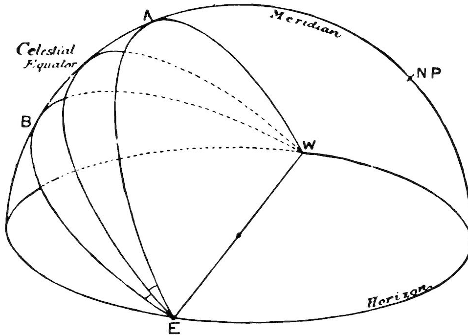
FIG. 22.—Position of Ecliptic at Sunset at Vernal Equinox (E A W) and Autumnal Equinox (E B W).
