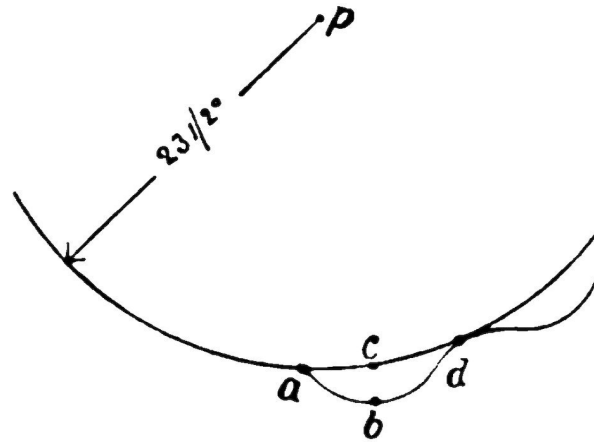
FIG. 46.—Nutation.
