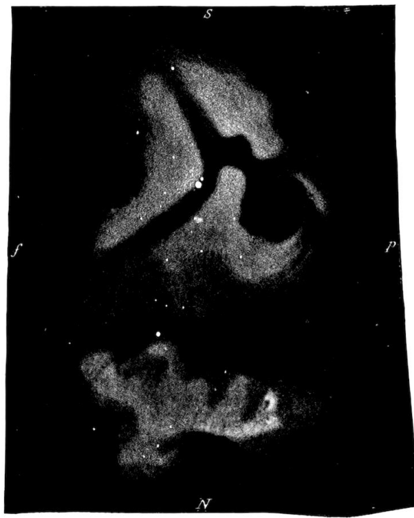
FIG. 16.— The Trifid Nebula, Sagittarius.
