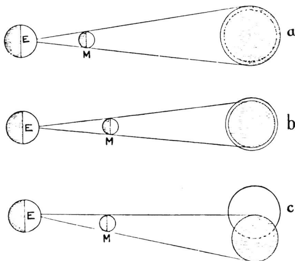
FIG. 31.—Eclipses of the Sun. (a) Total Eclipse, (b) Annular Eclipse, (c) Partial Eclipse.
