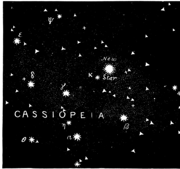
FIG. 8.— The Temporary Star of 1572.
