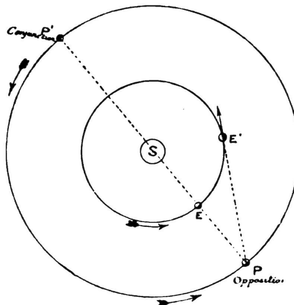
FIG. 25.— Movement of an Exterior Planet.
