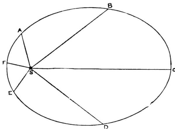
FIG. 13.— Elliptic Form of Earth's Orbit.
