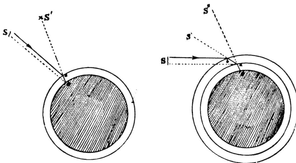
FIG. 5.—Atmospheric Refraction.
