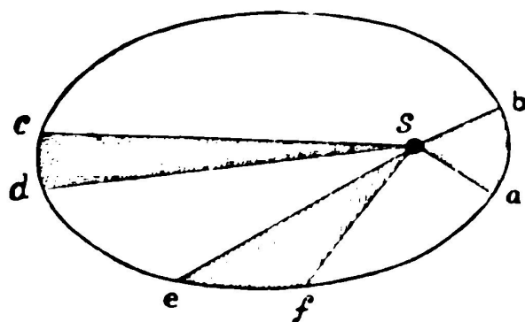
FIG. 16.— Illustrating Kepler's Second Law.
