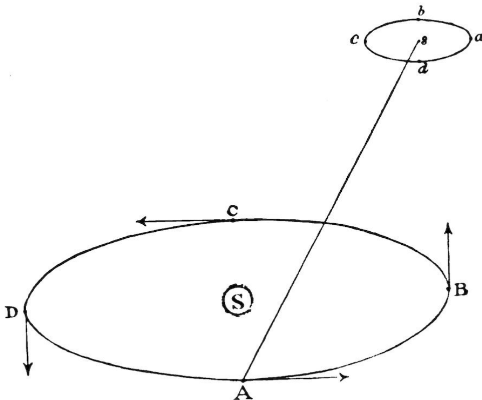
FIG. 7.— Aberrational Orbit of a Star.
