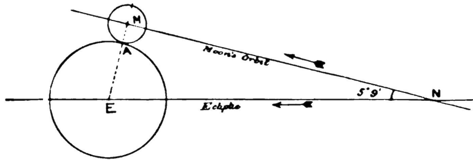
FIG. 30.—The Lunar Ecliptic Limit.
