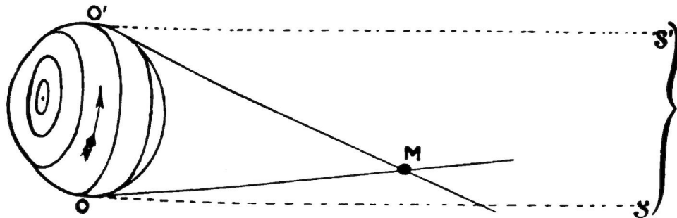
FIG. 42.— The Parallax of Mars.
