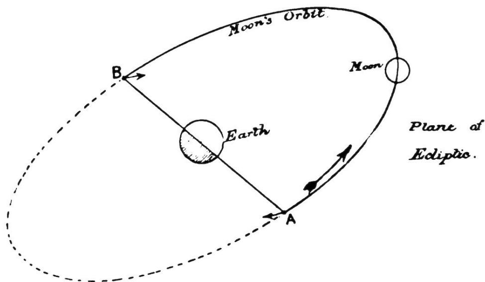
FIG. 21.—The Moon's Nodes.
