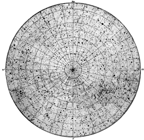
FIG. 1.— Stars visible in the Northern Hemisphere.
