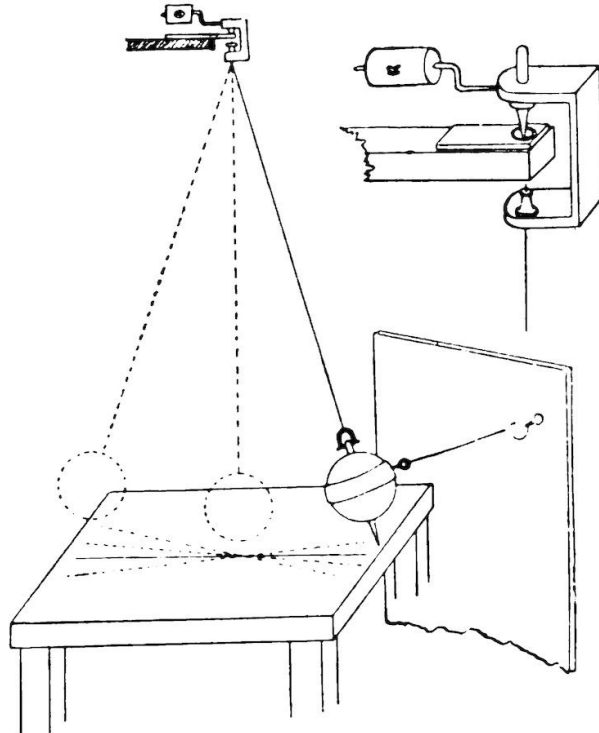
FIG. 3.—Foucault's Pendulum Experiment.
