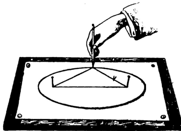
FIG. 15.—How to draw an Ellipse.
