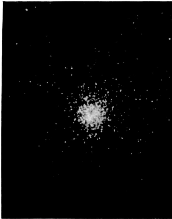
FIG. 12.— Star Cluster in Hercules.
