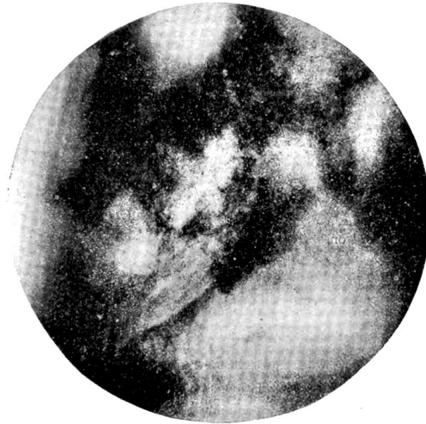
FIG. 19.— Photograph of Milky Way, Sagittarius.
