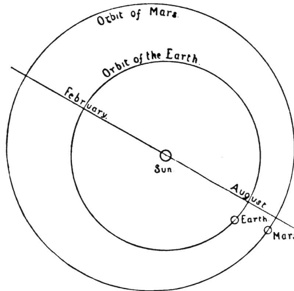
FIG. 27.— Opposition of Mars.
