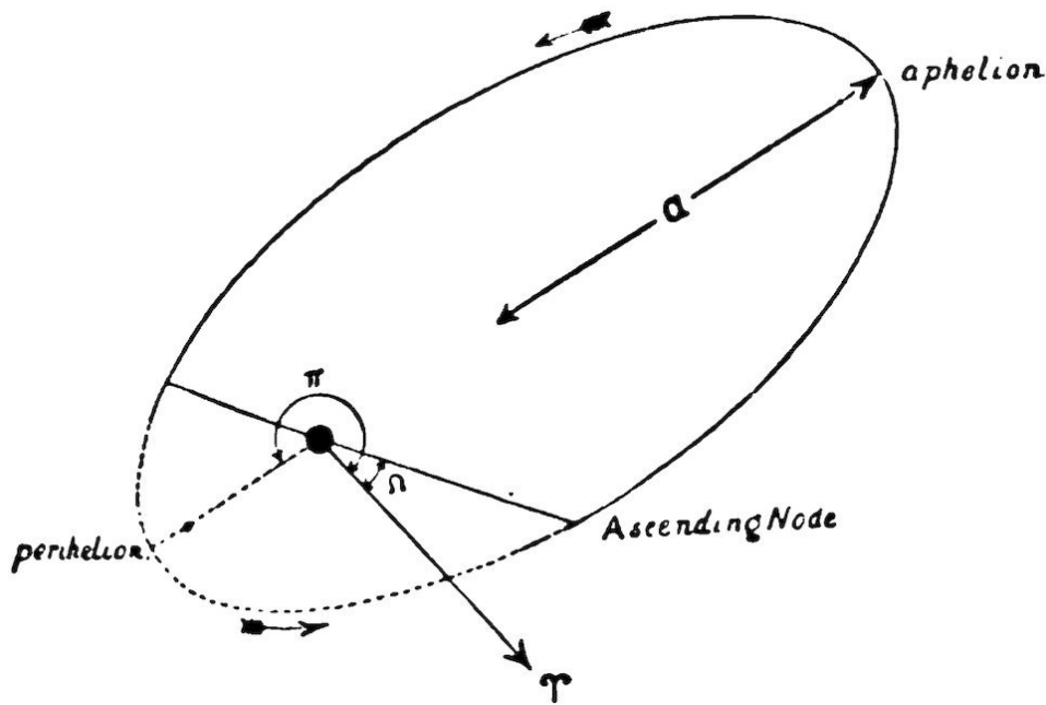
FIG. 28.—Elements of an Elliptic Orbit.
