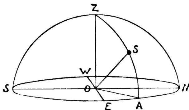
FIG. 11.—Altitude and Azimuth.
