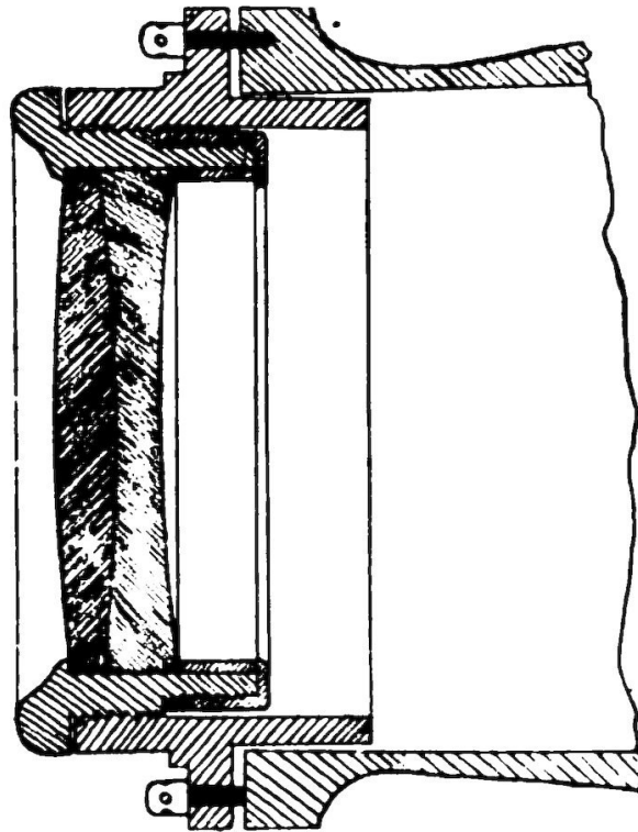
FIG. 49.— The Achromatic Object-Glass.
