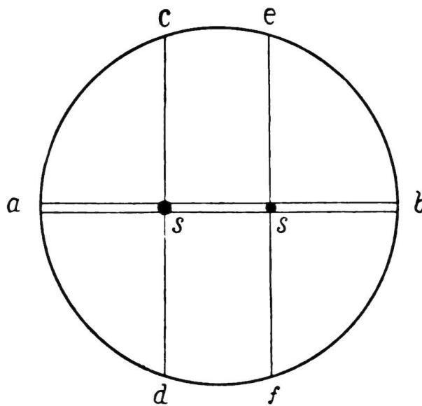
FIG. 54.— The Micrometer applied to a Binary Star: a b, Fixed Threads; c d, e f, Movable Threads; s s, Components of Binary Star.
