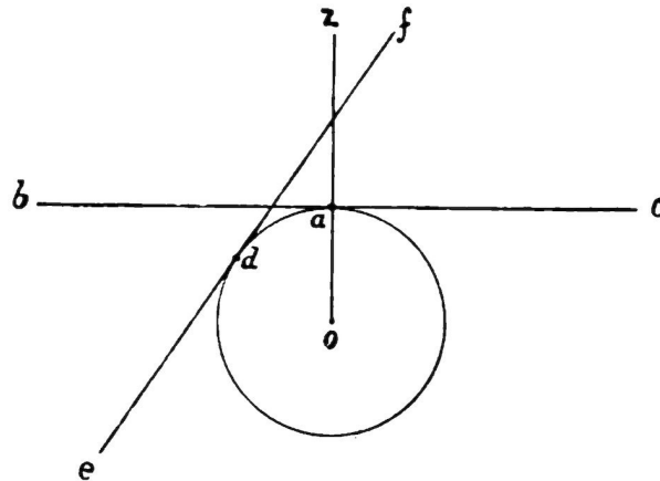
FIG. 2.—Horizons at Two Places on the Earth.
