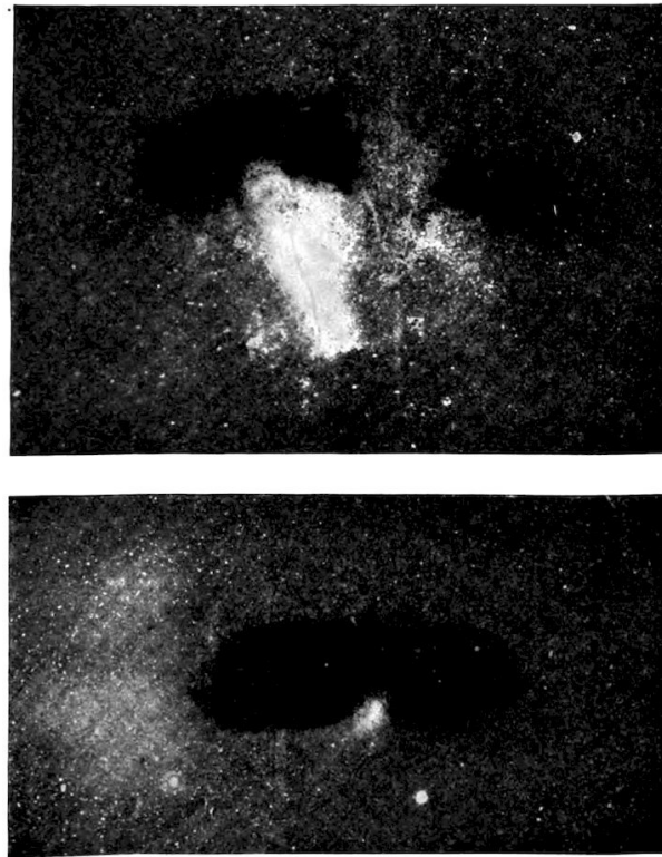
FIG. 18.— Magellanic Clouds.
