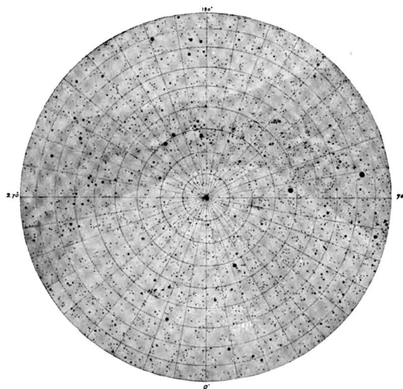
FIG. 2.—Stars visible in the Southern Hemisphere.
