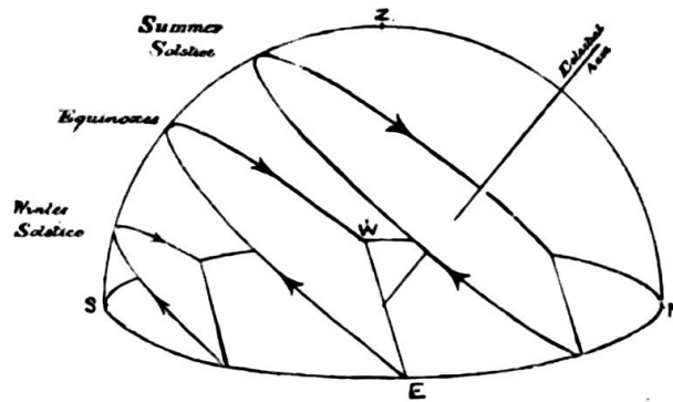
FIG. 6.— Apparent Paths of Sun at Equinoxes and Solstices.
