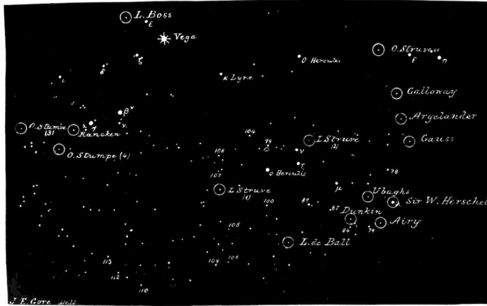
FIG. 3.—Diagram showing “Solar Apex,” and the different Positions found by various Computers.
