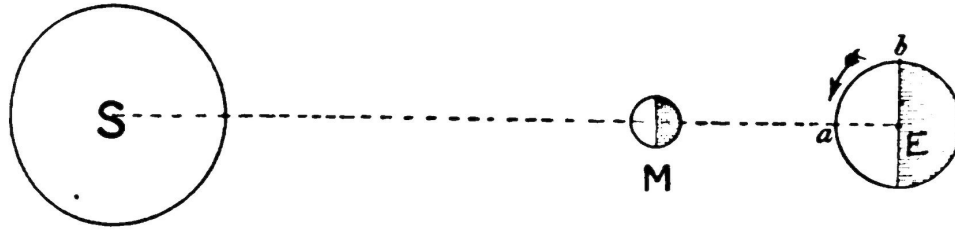
FIG. 32.— Duration of a Solar Eclipse.
