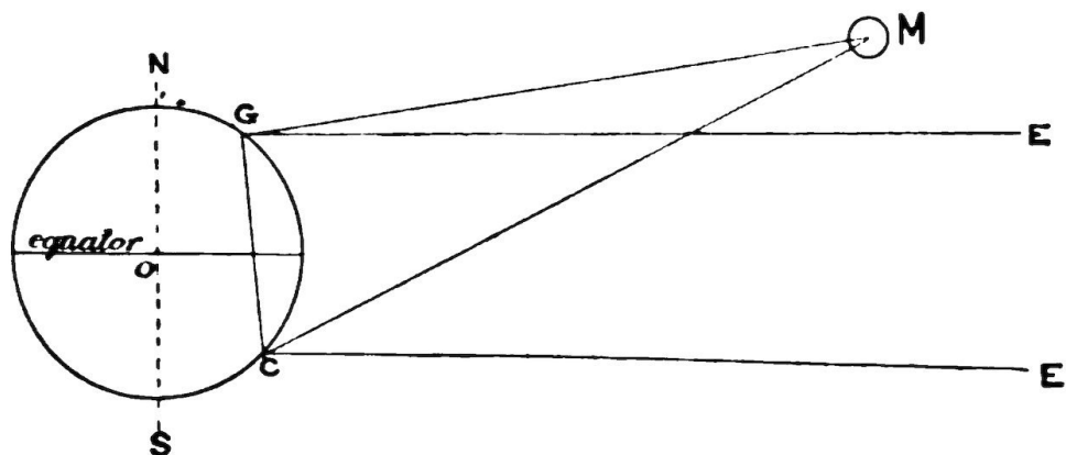
FIG. 40.—Measurement of the Moon's Distance.
