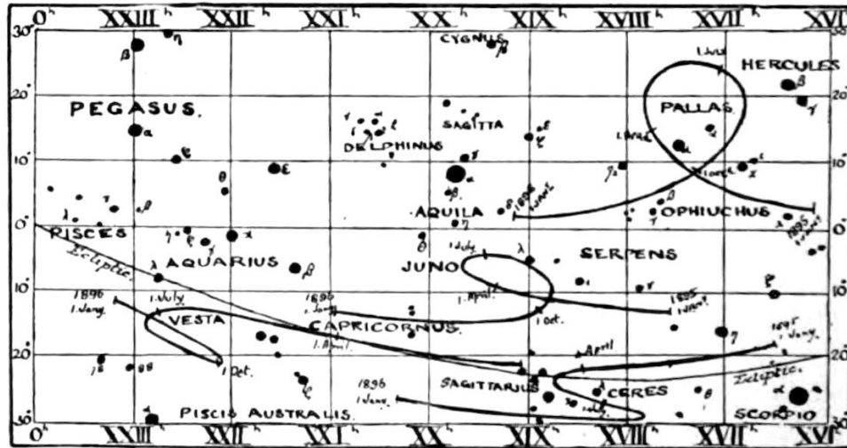
FIG. 26.—Apparent Paths of Ceres, Pallas, Juno and Vesta, in 1896.
