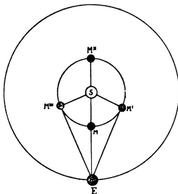
FIG. 23.—Movement of an Interior Planet.
