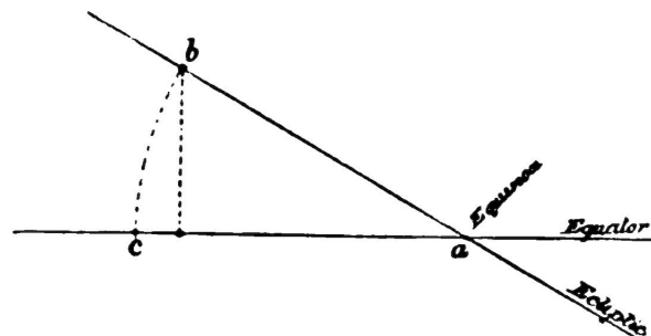
FIG. 17.— Effect of Obliquity of Ecliptic upon the Equation of Time.
