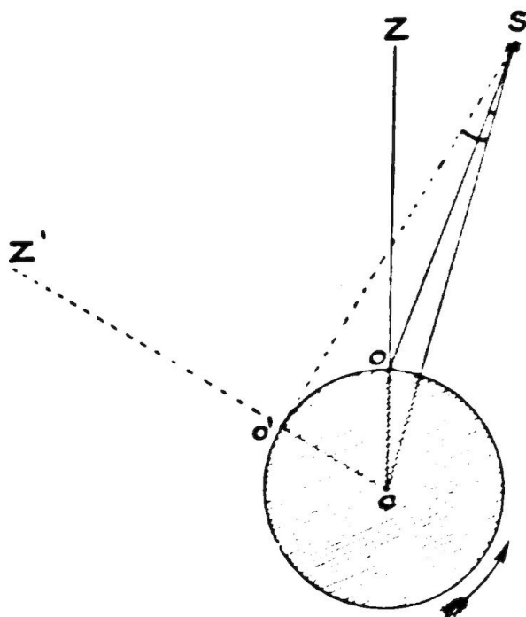
FIG. 38.—Parallax of a Heavenly Body.
