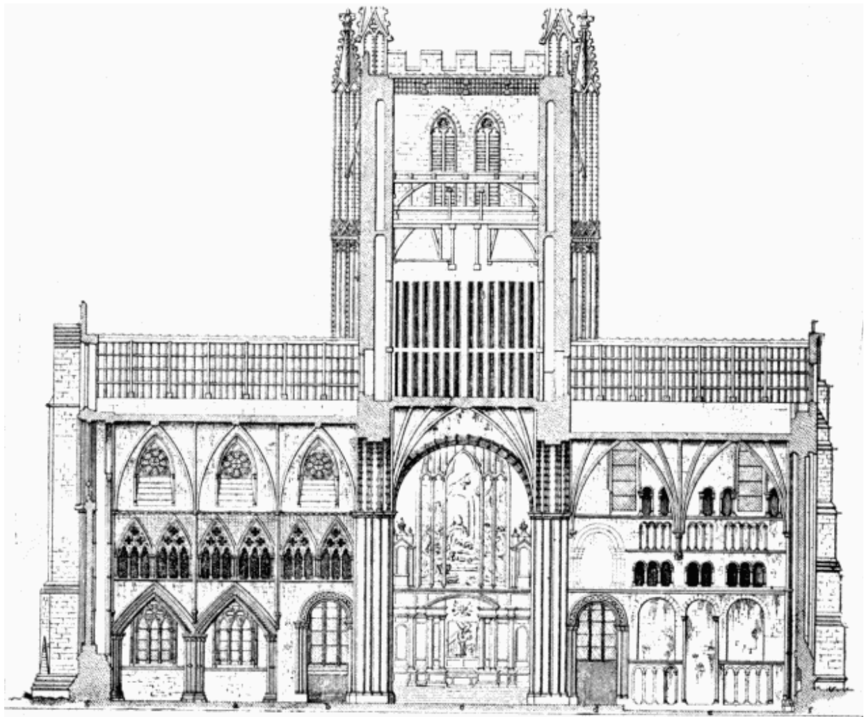
SECTION THROUGH TOWER AND TRANSEPTS.
