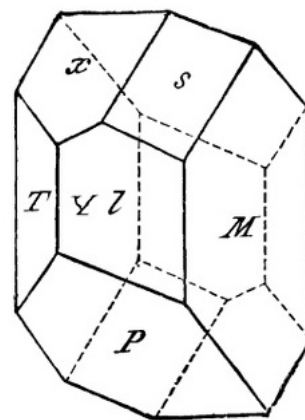
FIG. 11.—Triclinic pyramid. FIG. 12.—Triclinic system. Albite, &c.
