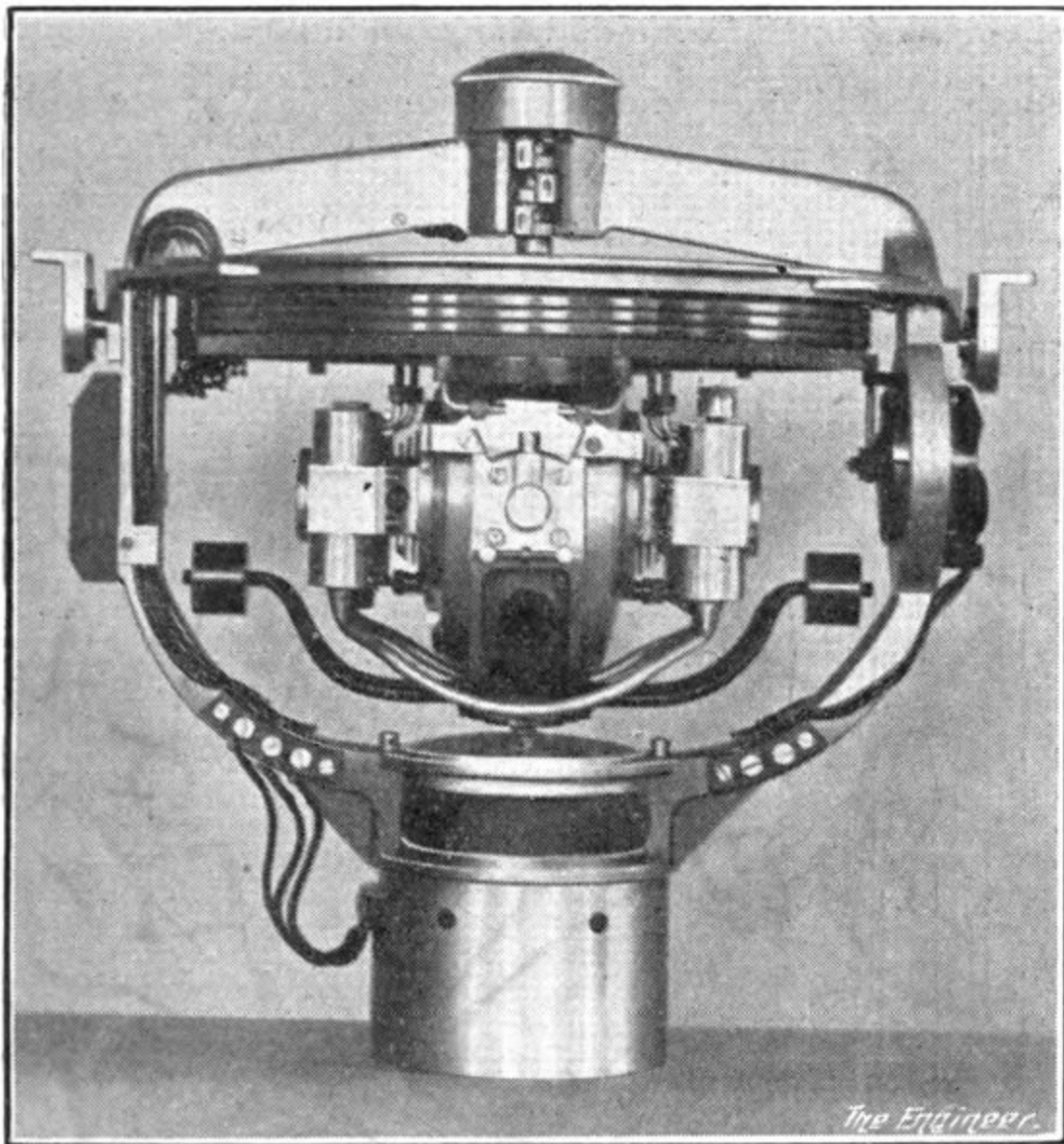
FIG. 48. The Brown Compass Removed from Binnacle.
