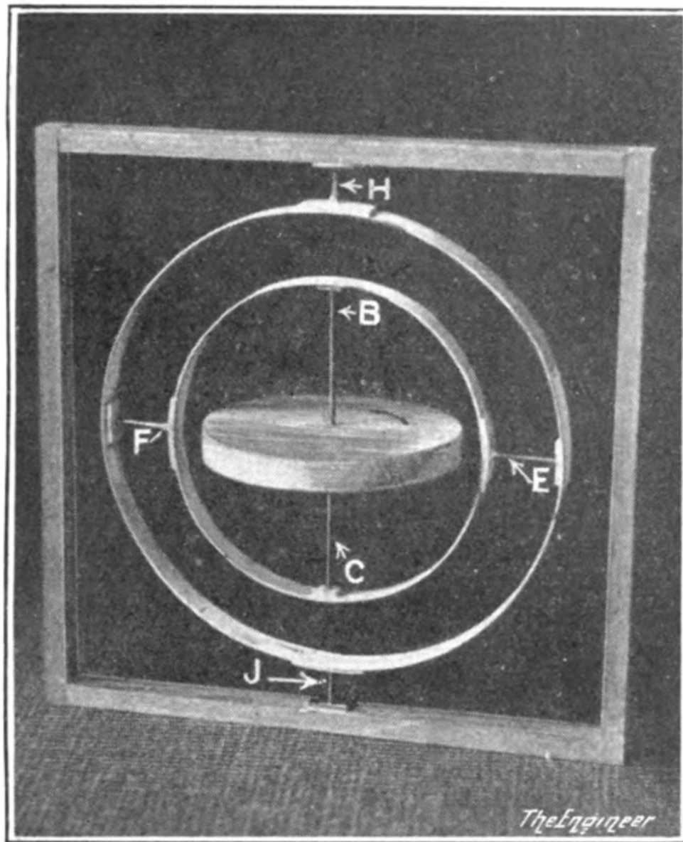
FIG. 4. One Degree of Freedom Lost.
