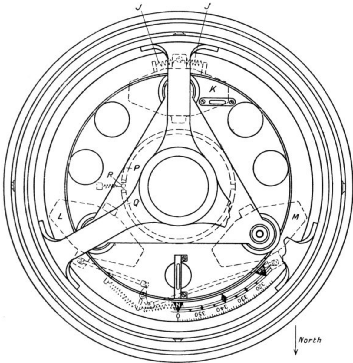
FIG. 50. Plan of Anschütz (1912) Compass.
