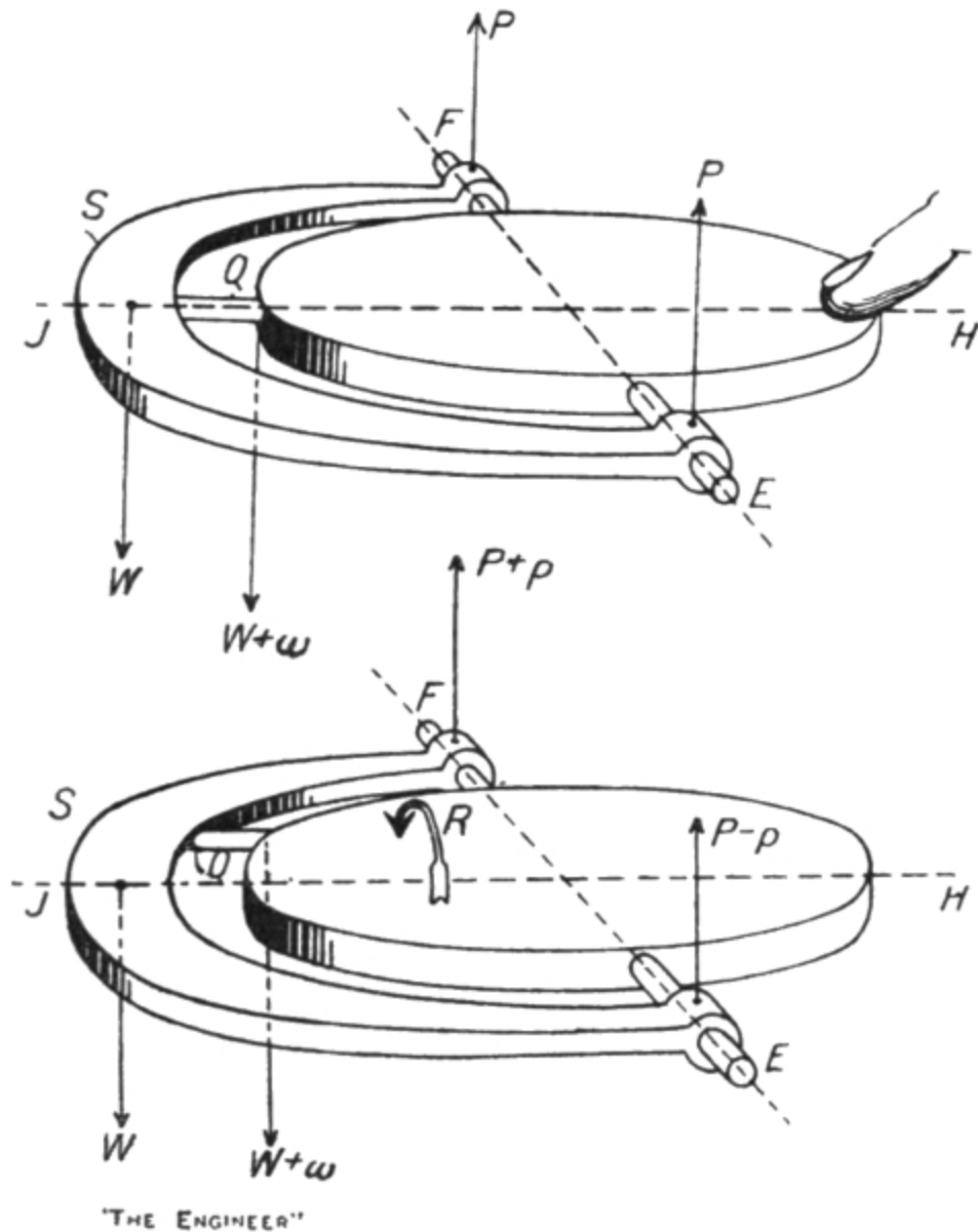
FIG. 20. Action of Excentric Pin in Sperry Compass.
