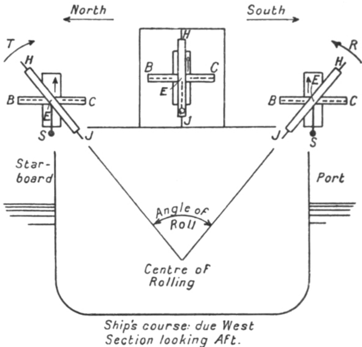
FIG. 30. Effect of Rolling on due West Course.
