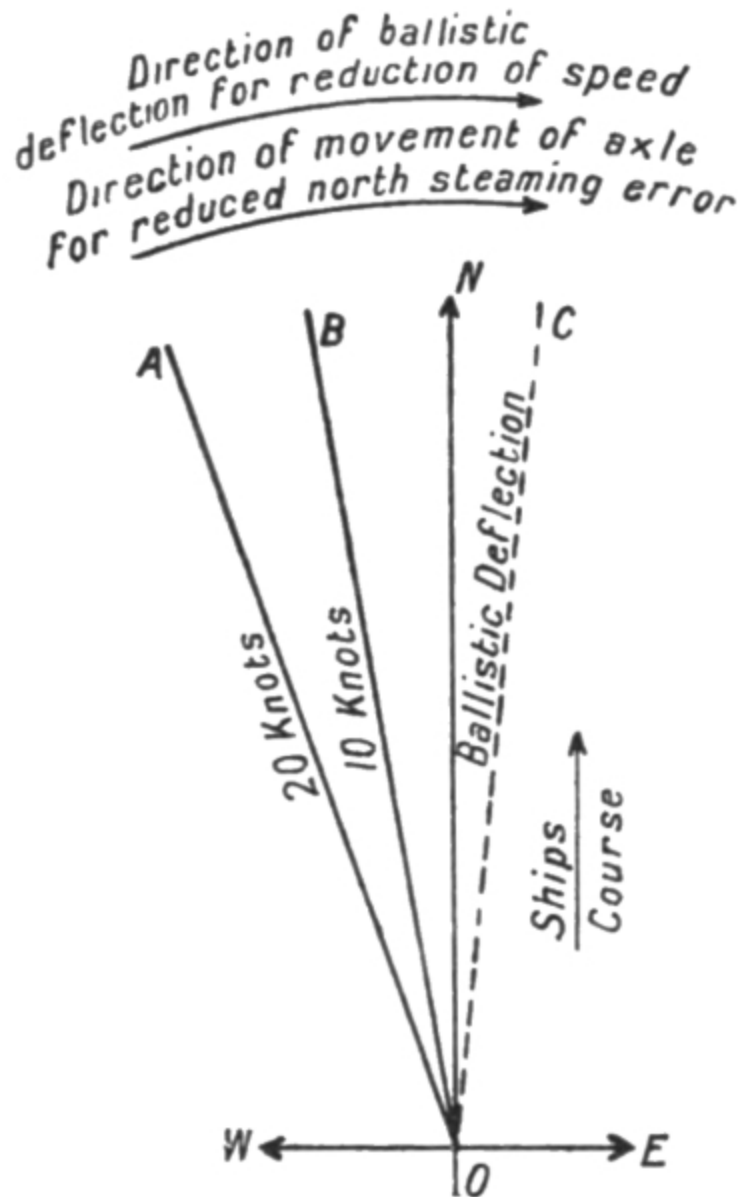
FIG. 28. Ballistic Deflection.
