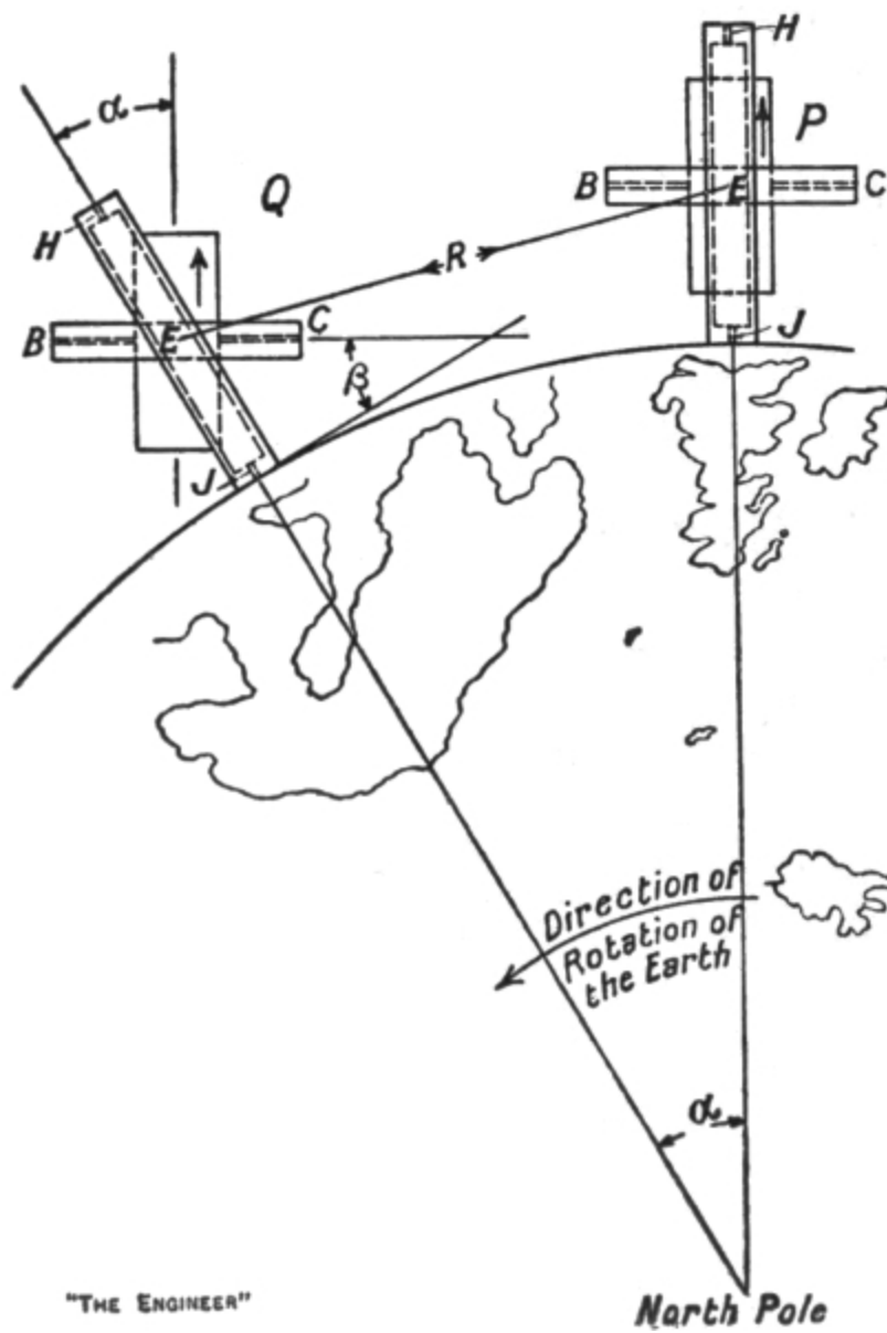
FIG. 7. Elementary Gyroscope at Equator.
