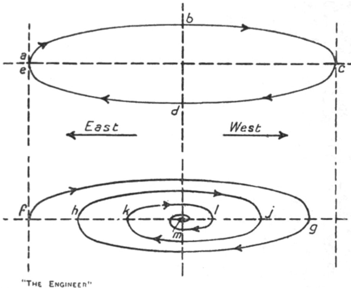
FIG. 17. Free and Damped Motion of Axle.
