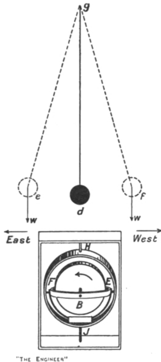
FIG. 13. Pendulum and Compass.
