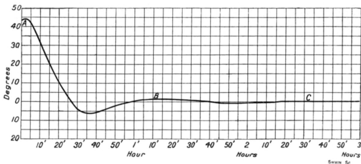
FIG. 18. Damping Curve from Anschütz (1910) Compass.
