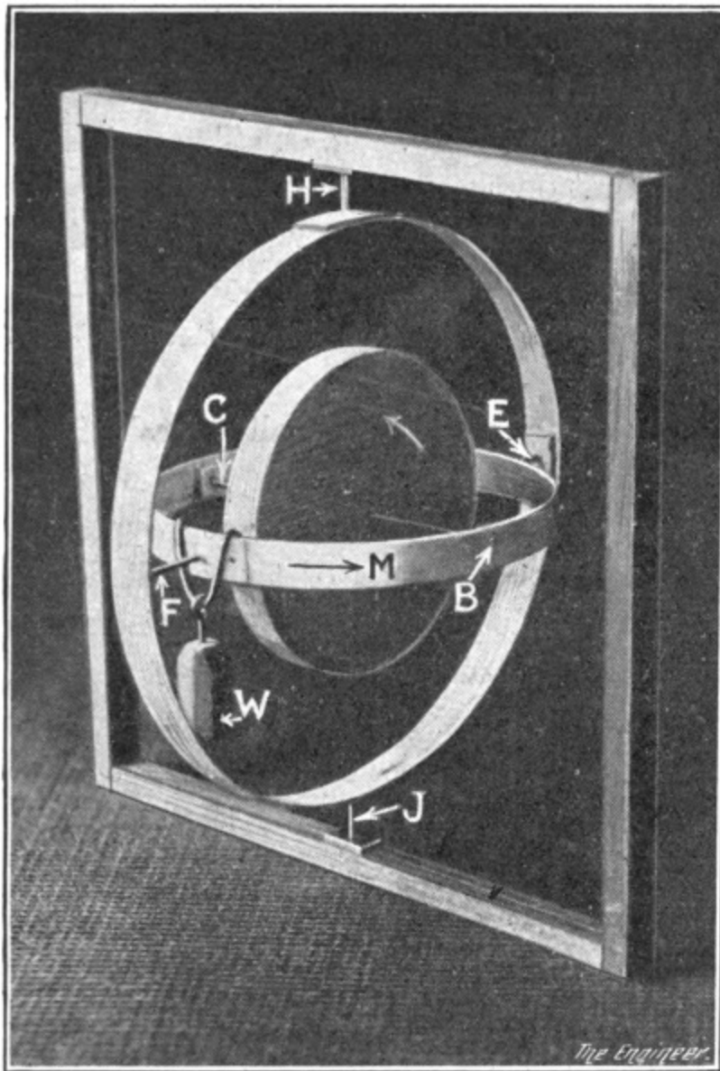
FIG. 2. Model Gyroscope, with Three Degrees of Freedom.
