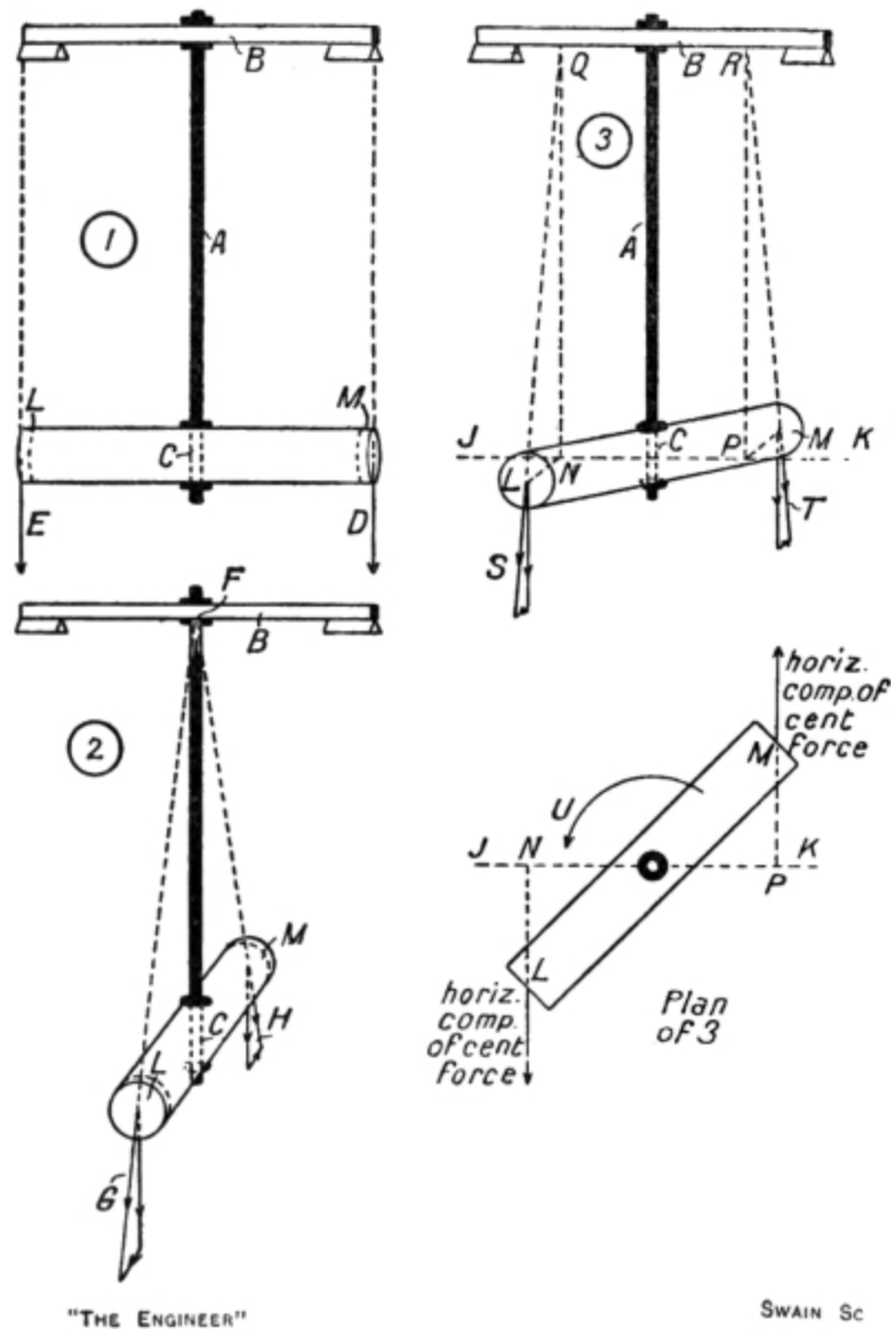
FIG. 43. Centrifugal Forces on a Pendulum.
