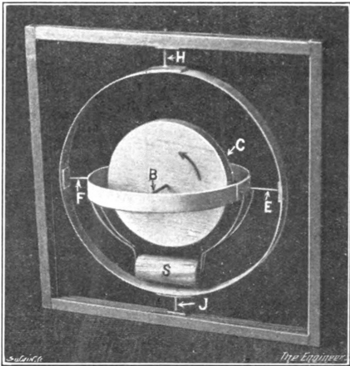
FIG. 9. Elementary Gyro-Compass.
