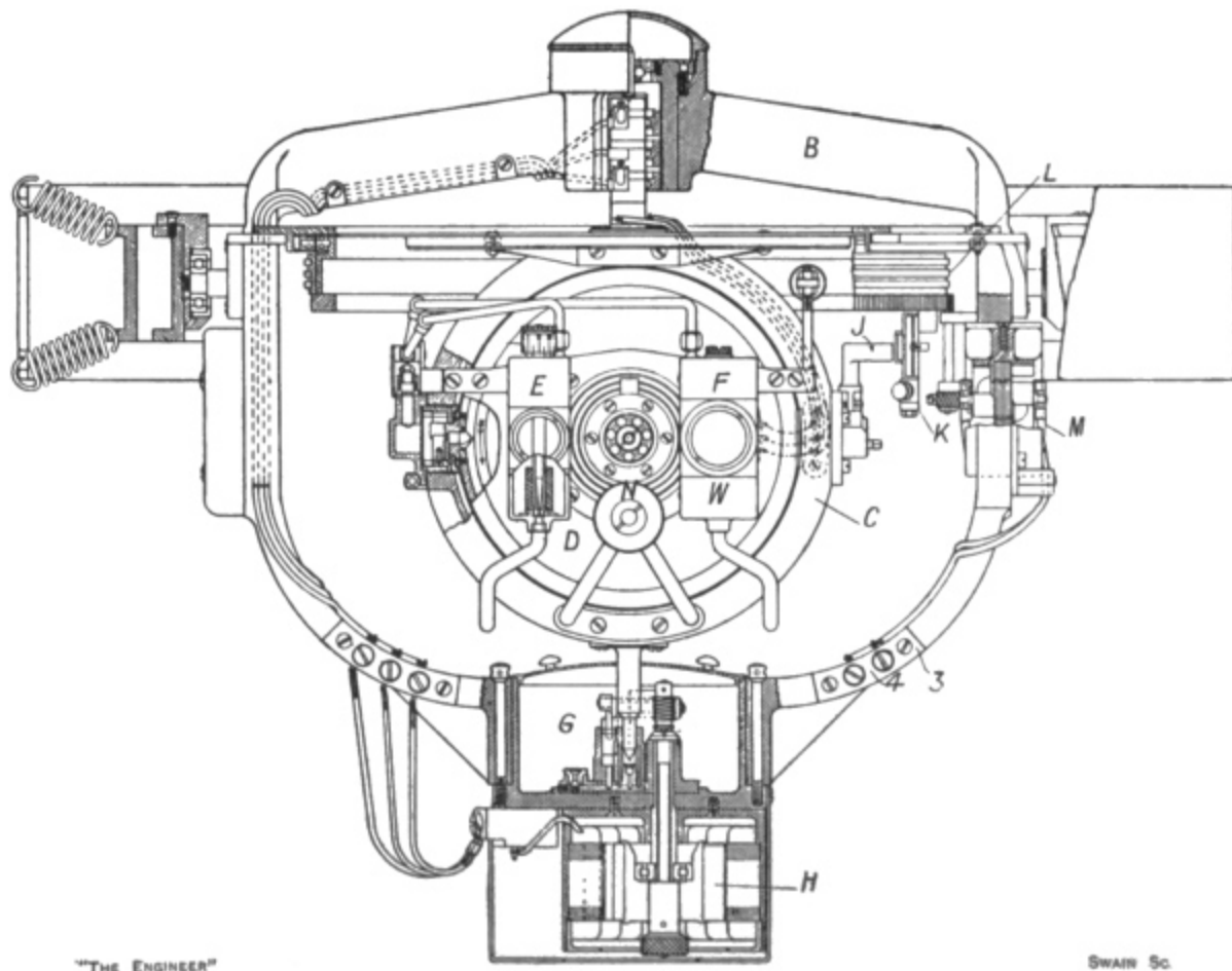
FIG. 49. The Brown Compass.
