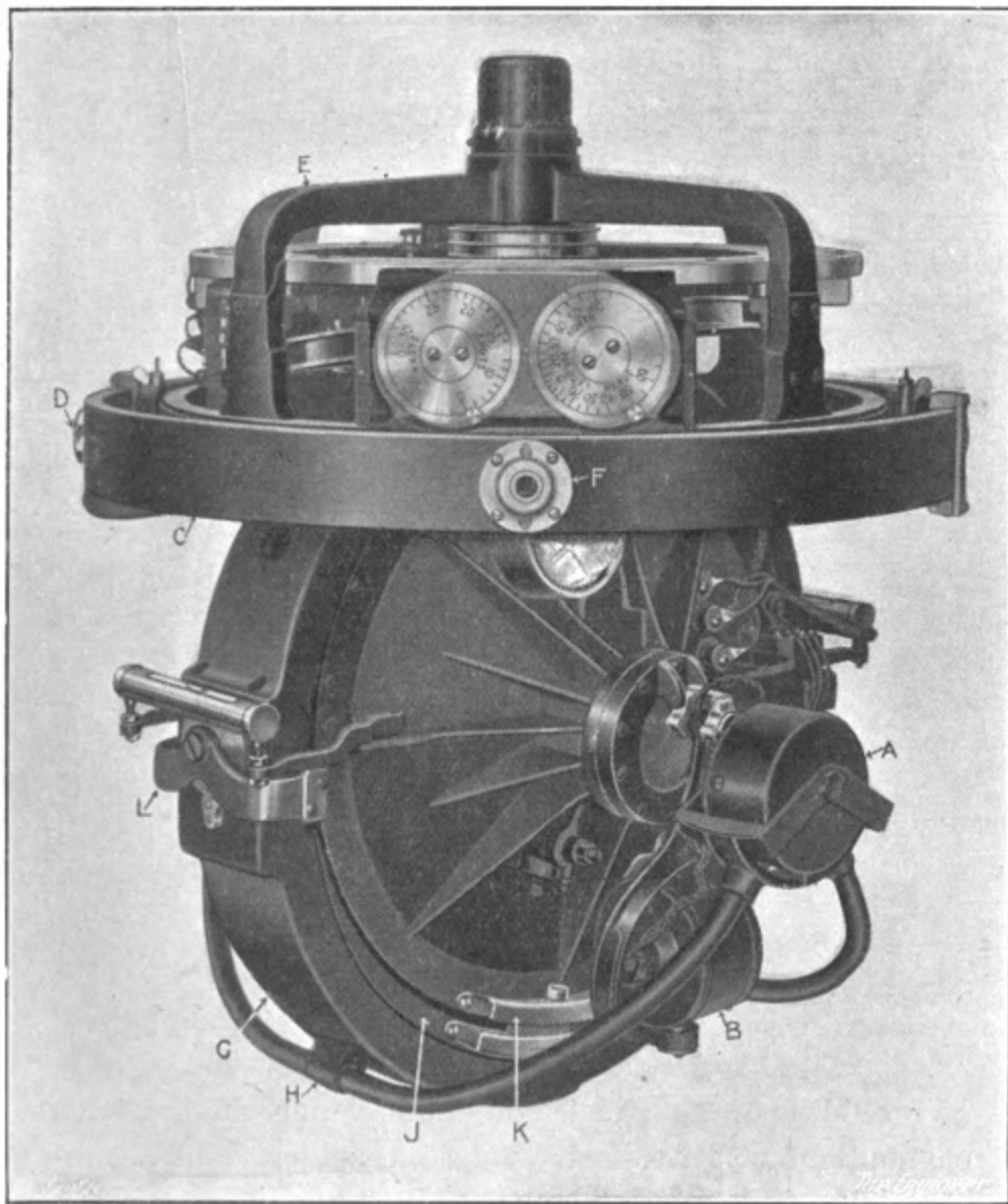
FIG. 45. The Sperry Compass Removed from Binnacle.
