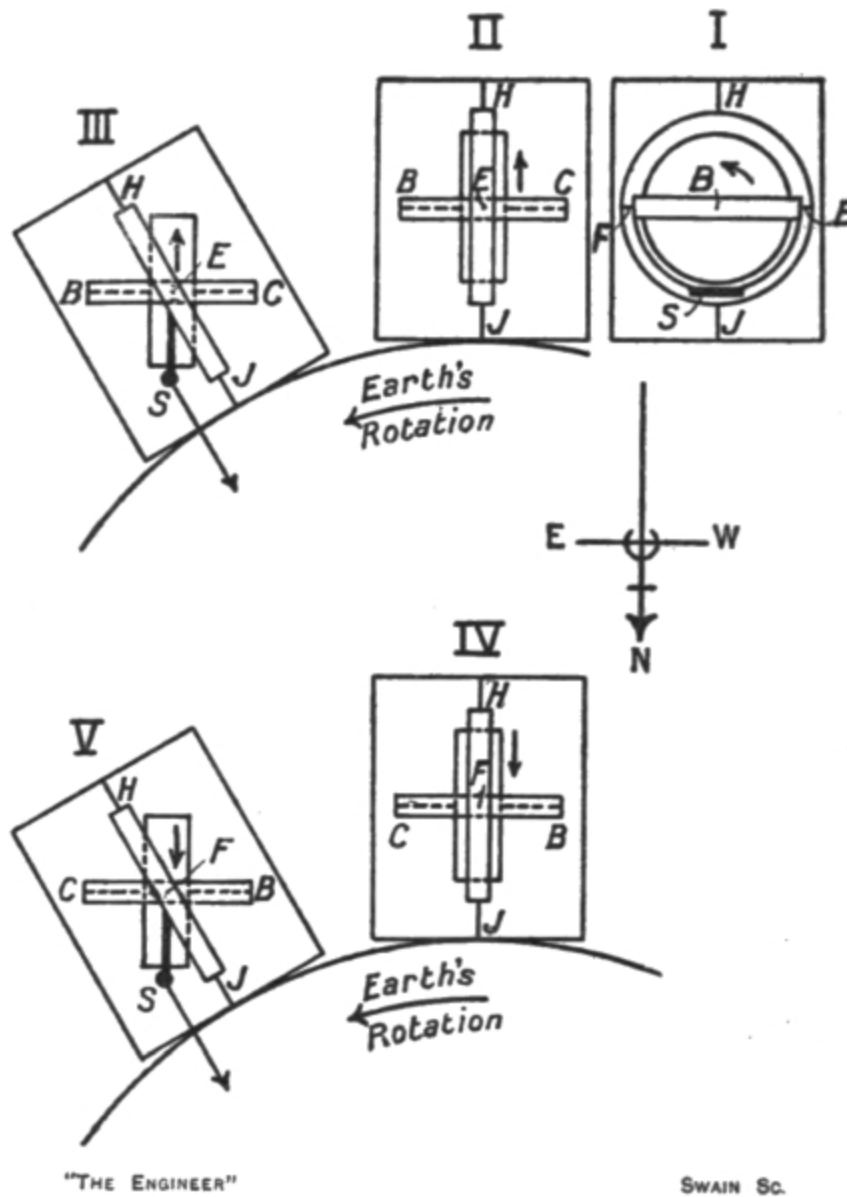
FIG. 10. Elementary Compass at Equator.
