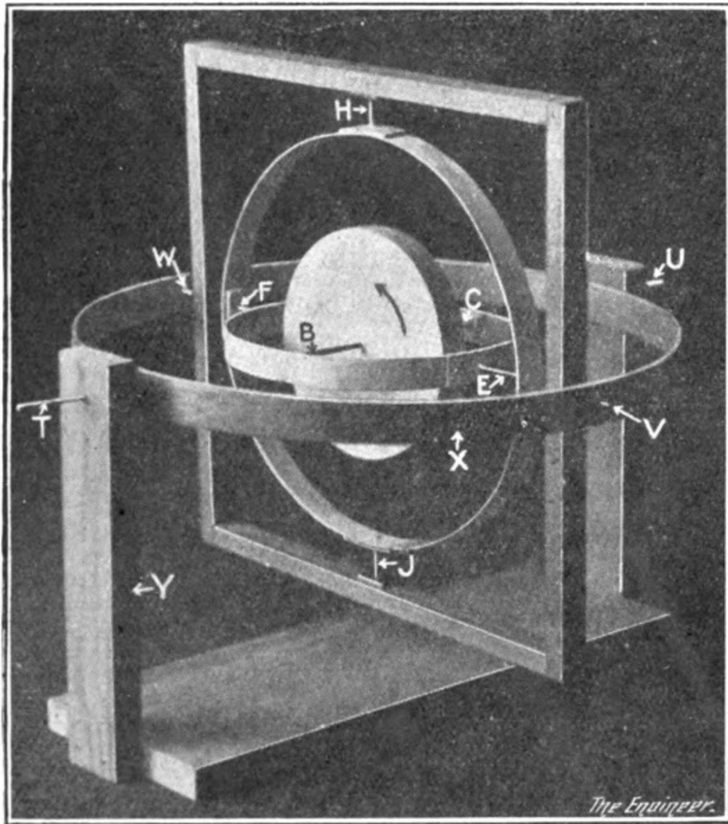
FIG. 6. Lost Degrees of Freedom Restored.
