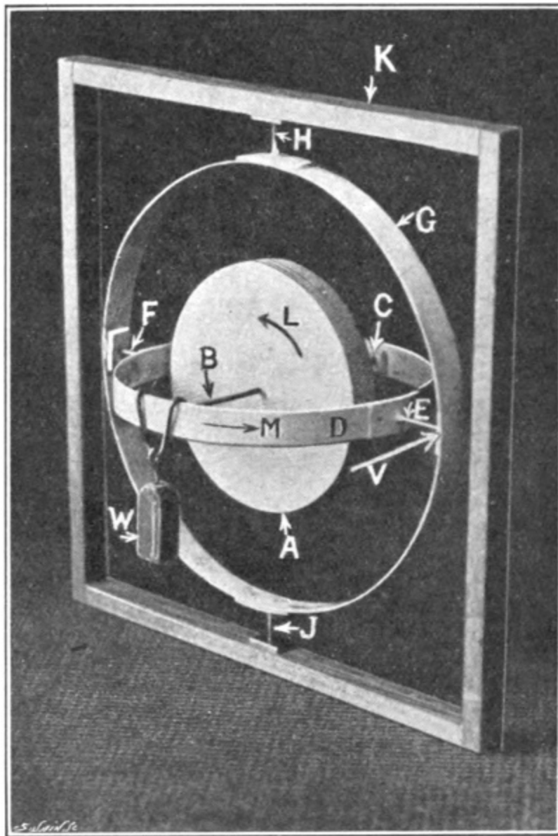
FIG. 1. Model Gyroscope, with Three Degrees of Freedom.
