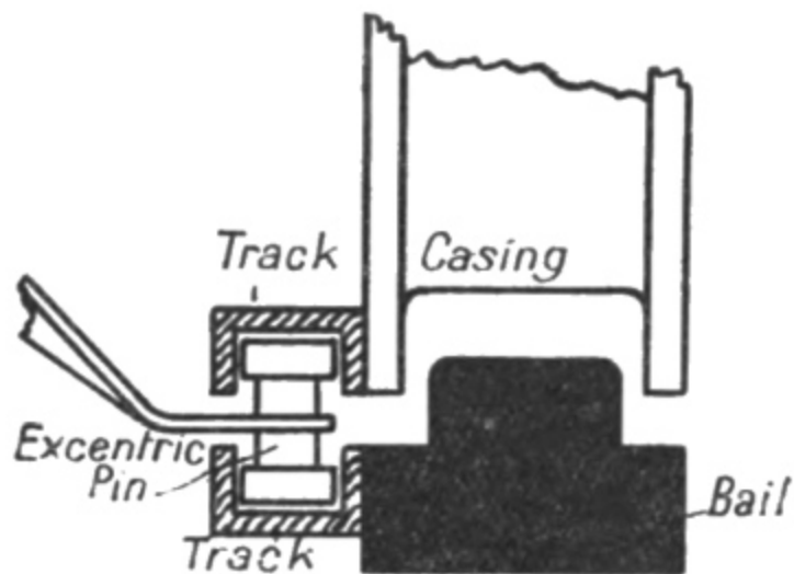
FIG. 37. Stabilized Excentric Pin (Sperry Compass).
