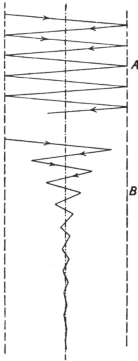
FIG. 14. Damped and Undamped Vibrations.
