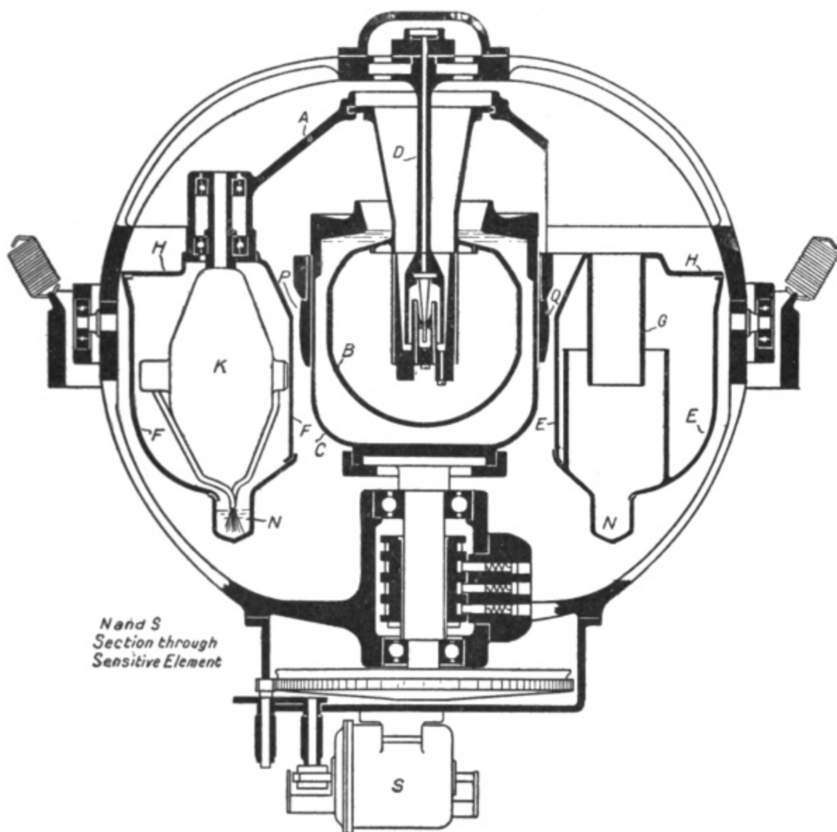
FIG. 51. Sectional Elevation of Anschütz (1912) Compass.
