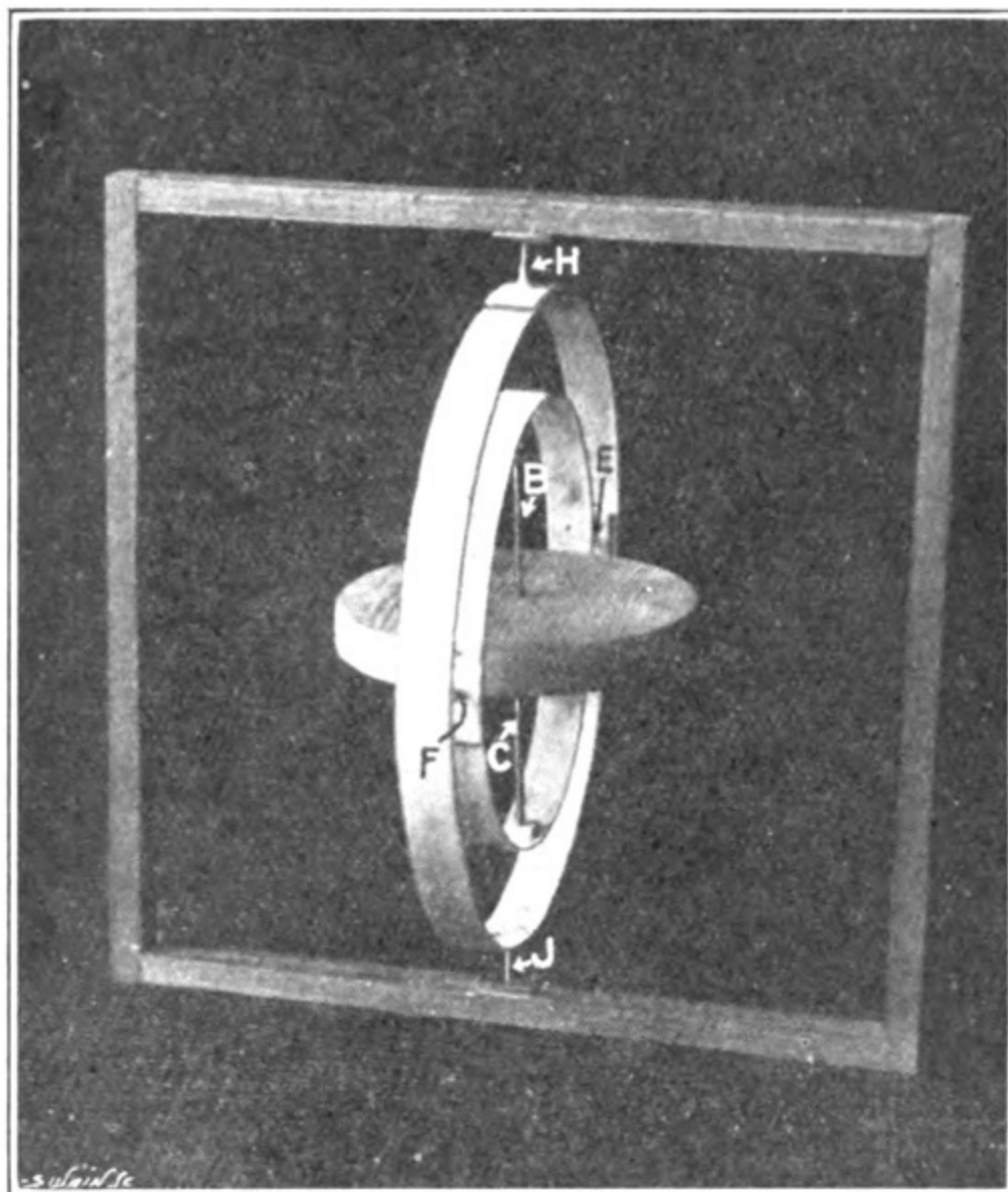
FIG. 5. Second Degree of Freedom Lost.
