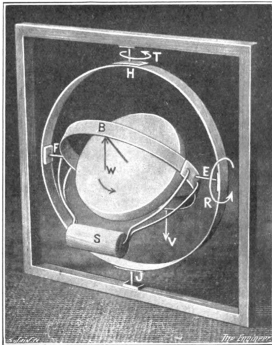
FIG. 22. Gyro-Pendulum with Axle Tilted.
