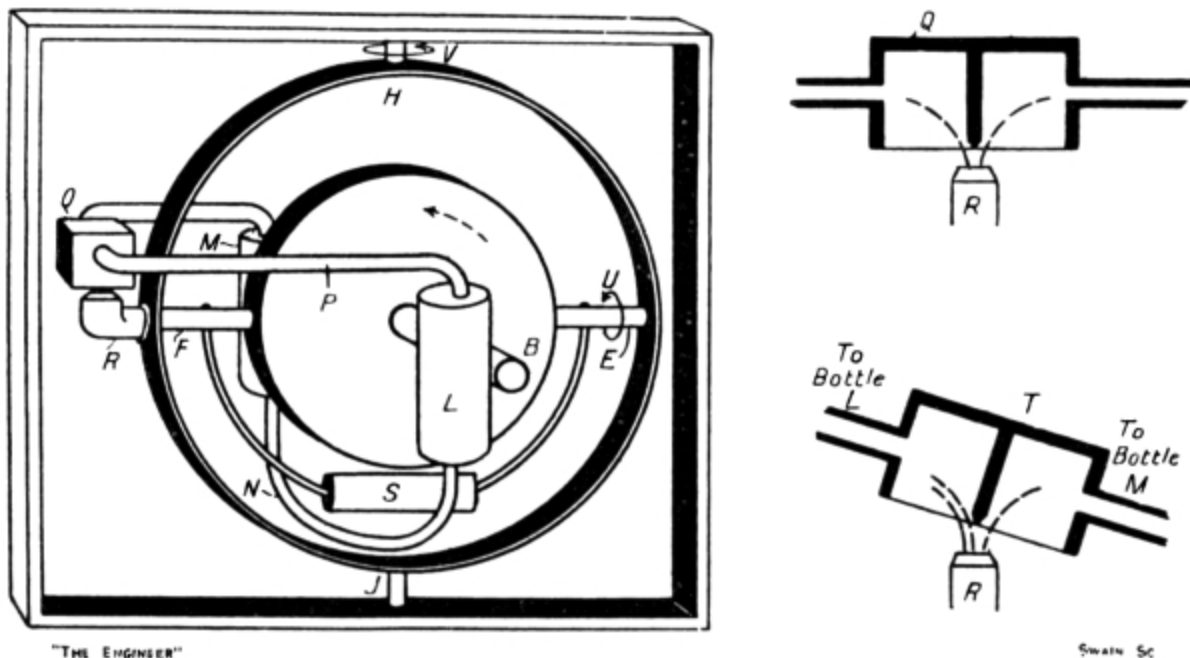
FIG. 23. Damping System of Brown Compass.
