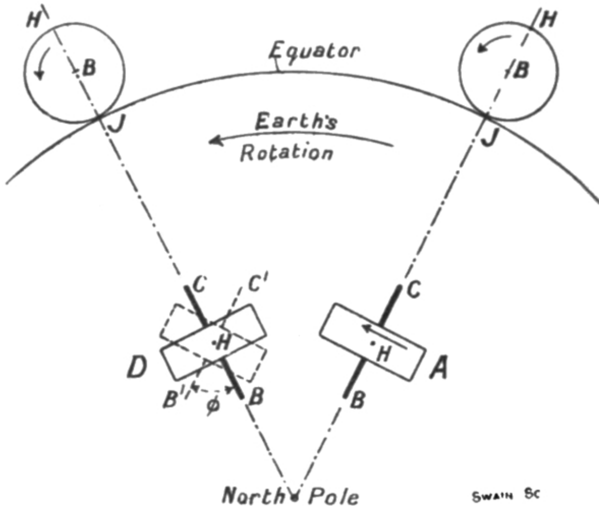
FIG. 12. Compass at Equator and near North Pole.
