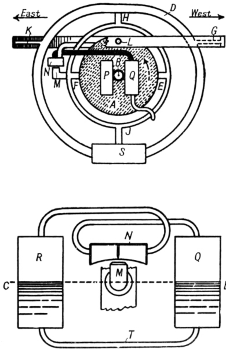
FIG. 38. Diagram of Brown Compass.
