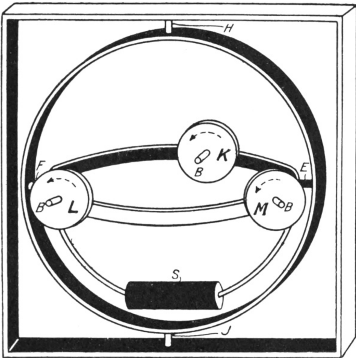
FIG. 41. Diagram of Anschütz (1912) Compass.
