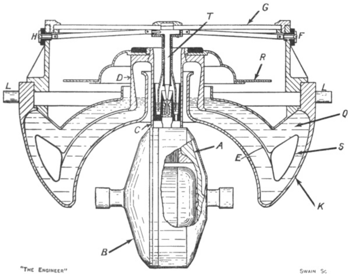
FIG. 44. The Anschütz (1910) Compass.
