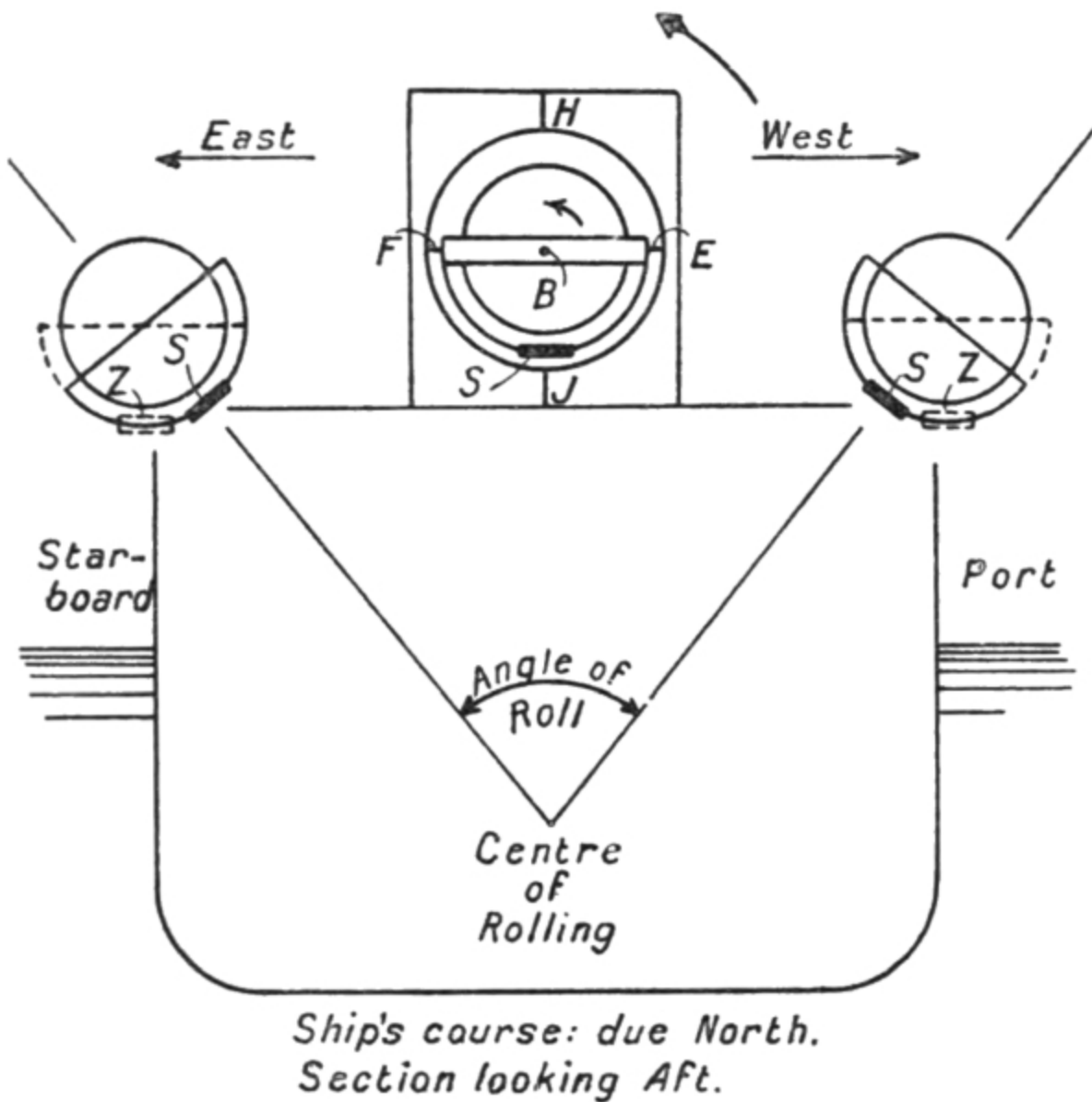
FIG. 29. Effect of Rolling on due North Course.
