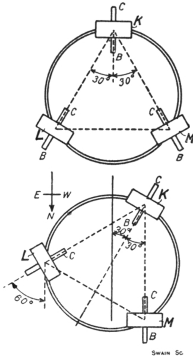
FIG. 42. Plans of Gyros.
