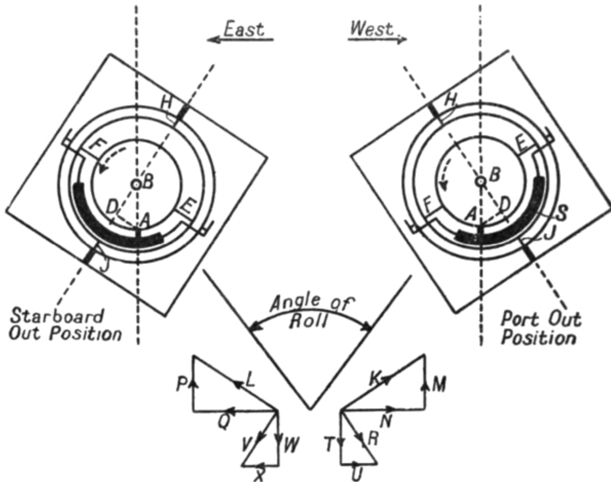
FIG. 35. Sperry Compass on N.W. course.
