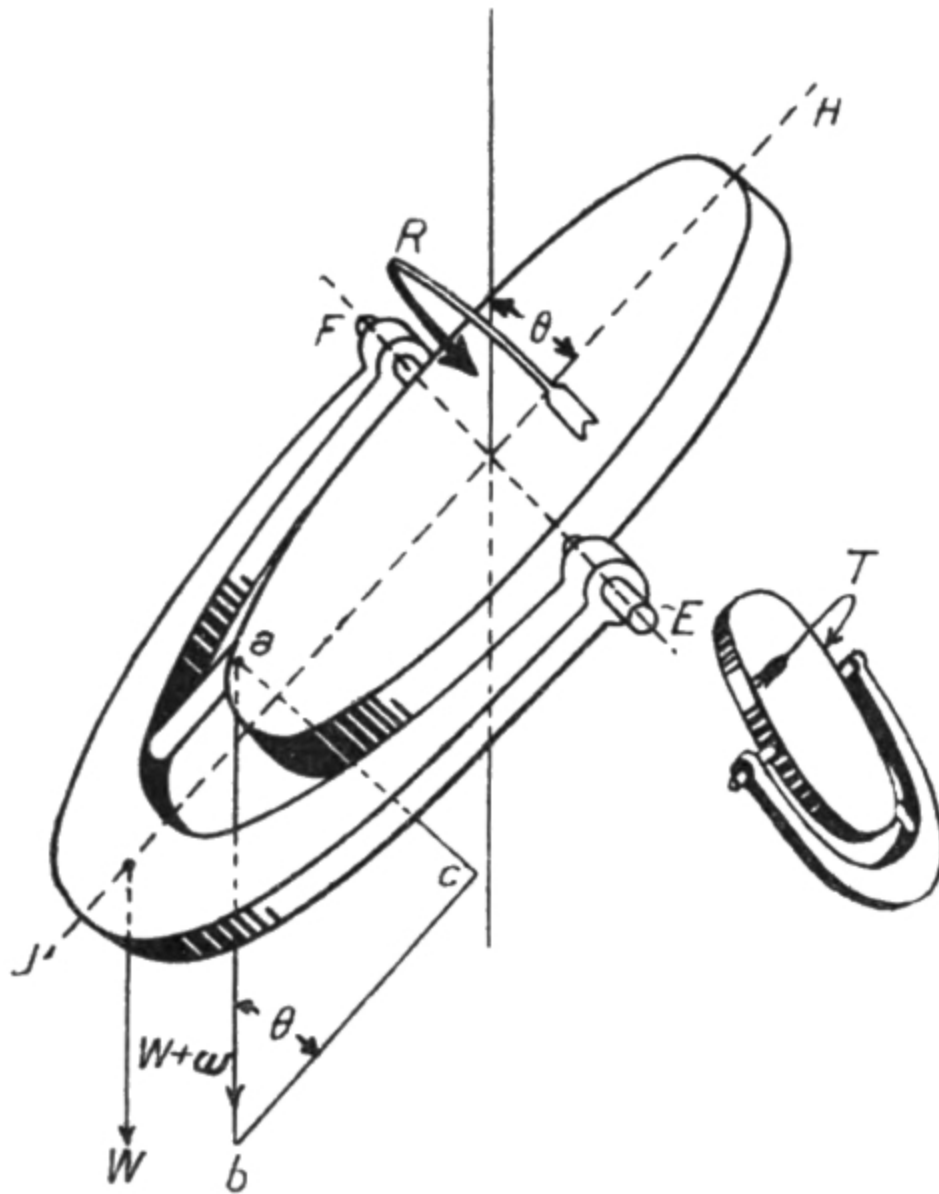
FIG. 21. Action of Excentric Pin in Sperry Compass.
