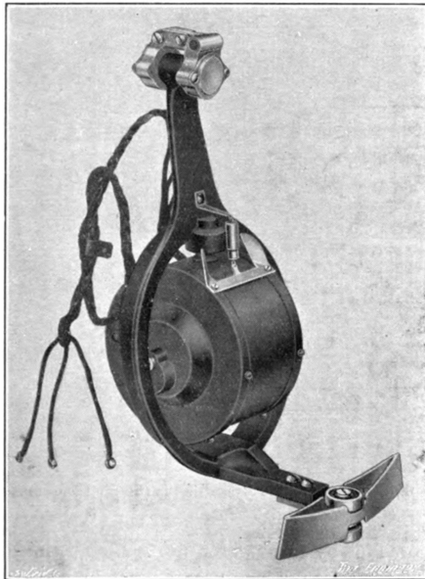
FIG. 36. Sperry Ballistic Gyro.
