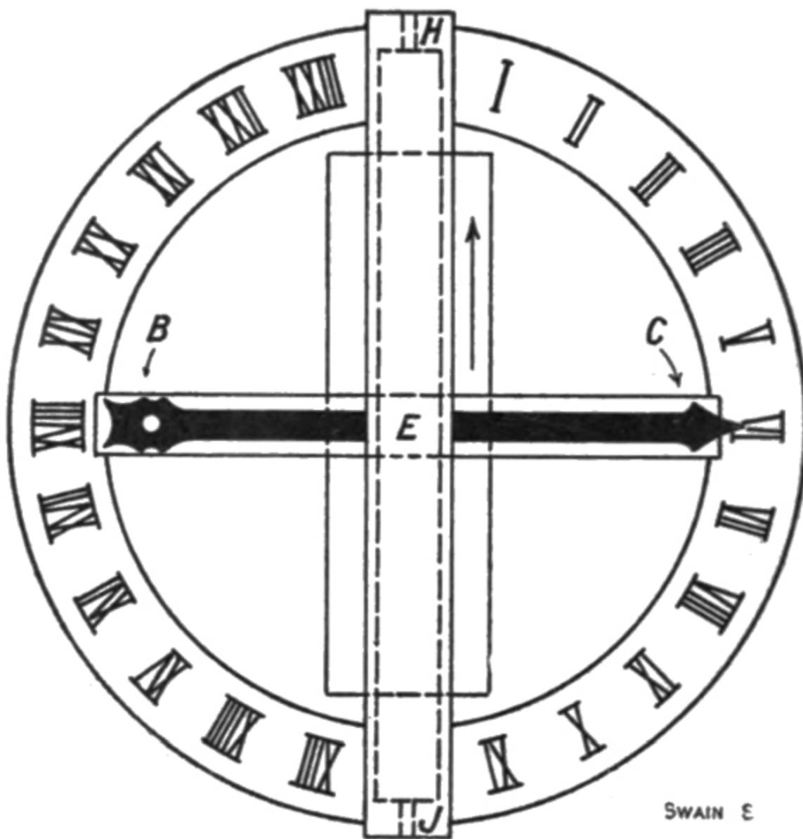
FIG. 8. Gyroscopic Clock.
