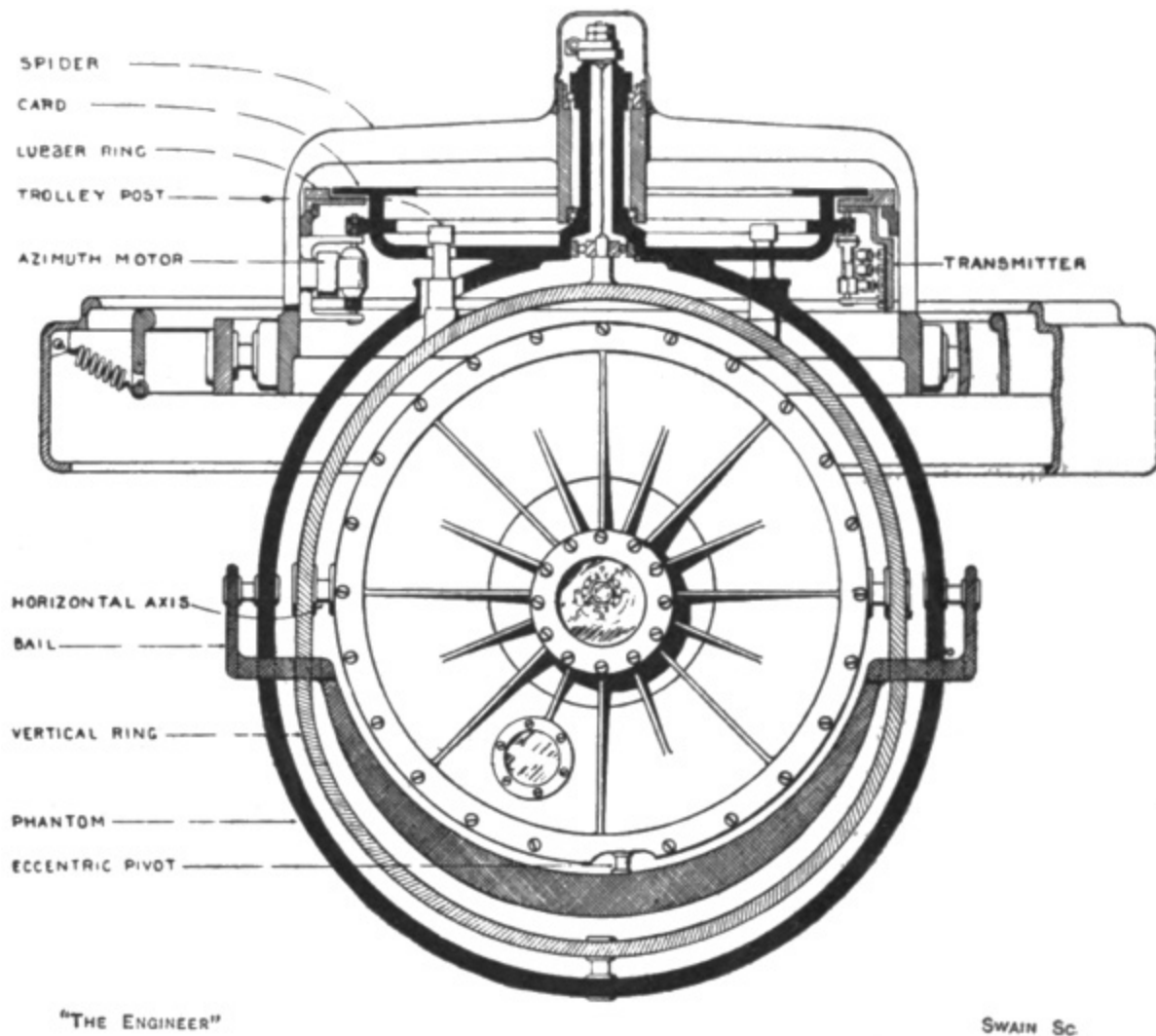
FIG. 46. The Sperry Compass.
