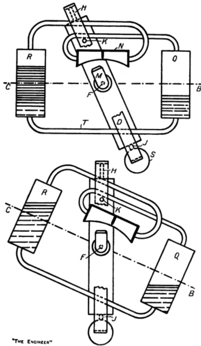
FIG. 39. Oil Control Bottles (Brown Compass).
