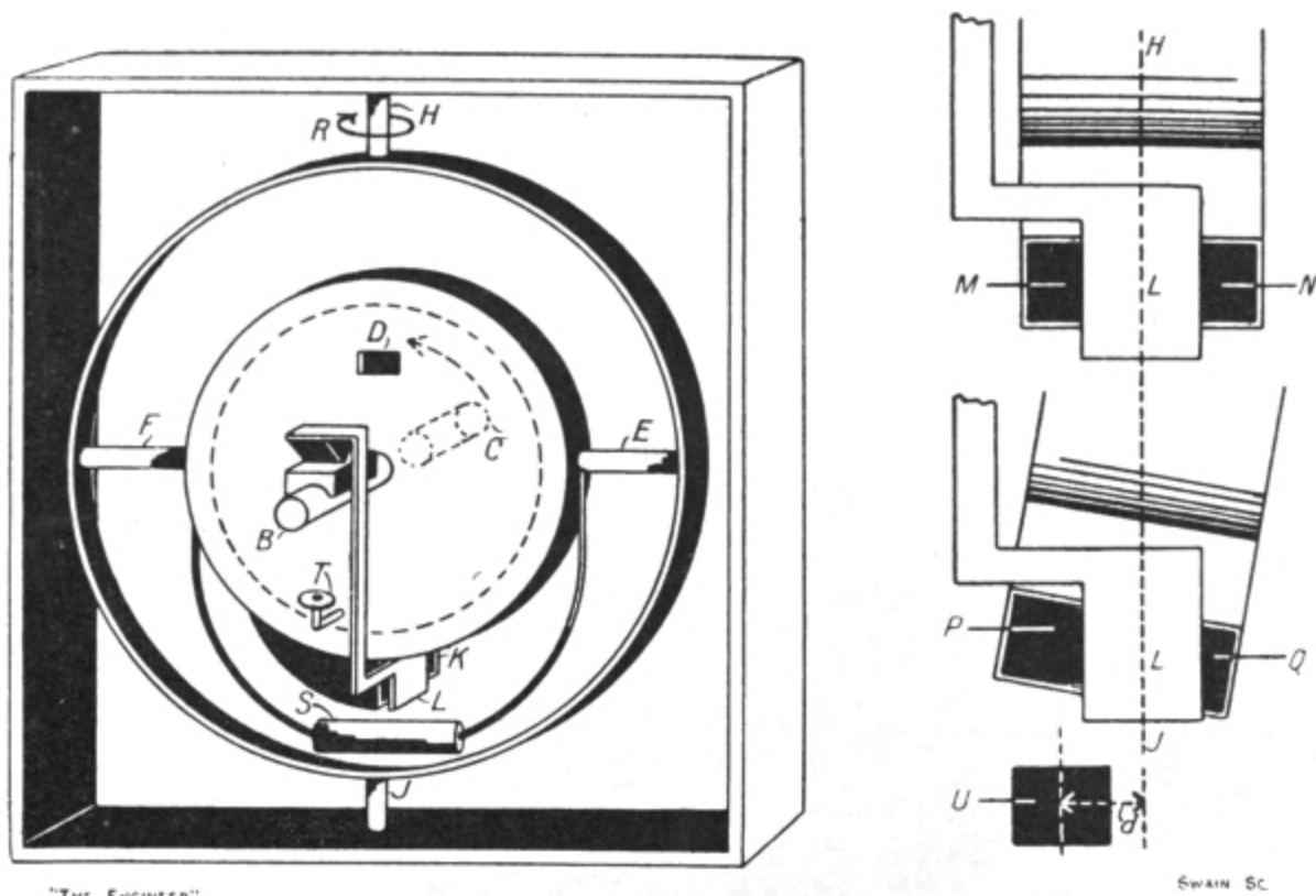
FIG. 16. Air Blast Damping System of Anschütz (1910) Compass.
