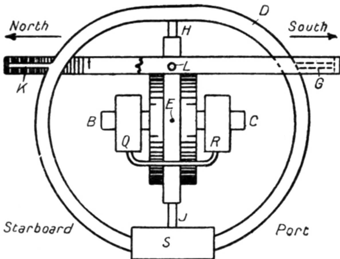
Ship's course: due west View of compass looking aft
