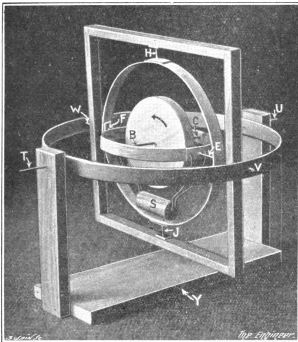
FIG. 31. External Gimbal Mounting.
