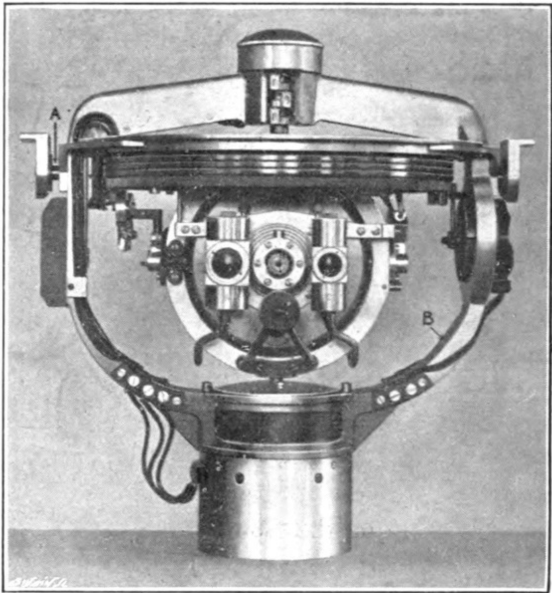
FIG. 47. The Brown Compass Removed from Binnacle.
