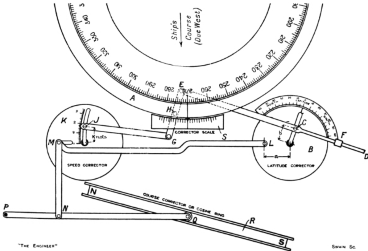
FIG. 25. Sperry Correction Mechanism for Latitude and North Steaming Errors.
