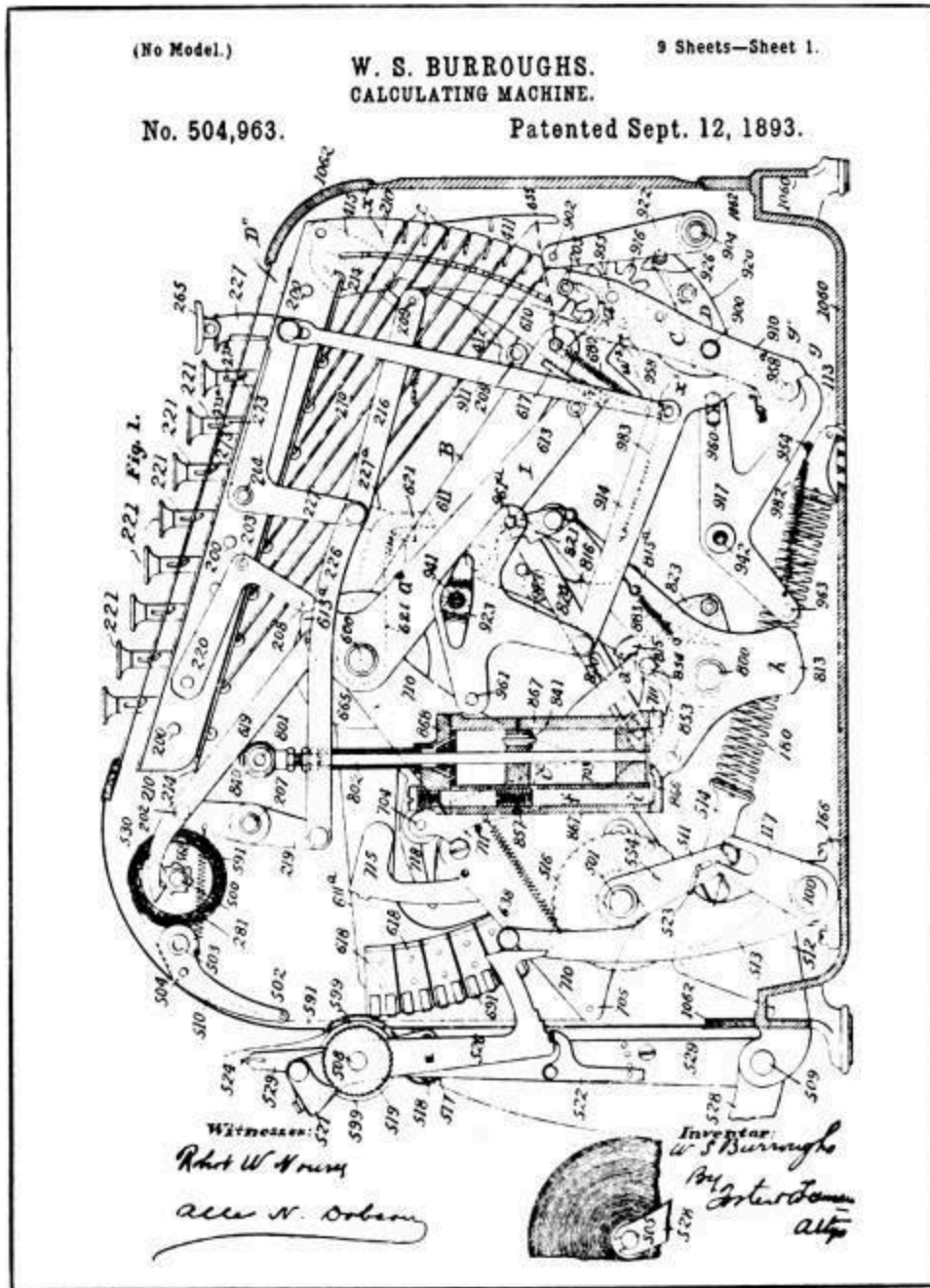
From Drawings of Burroughs' Patents Nos. 504,963 and 505,078
