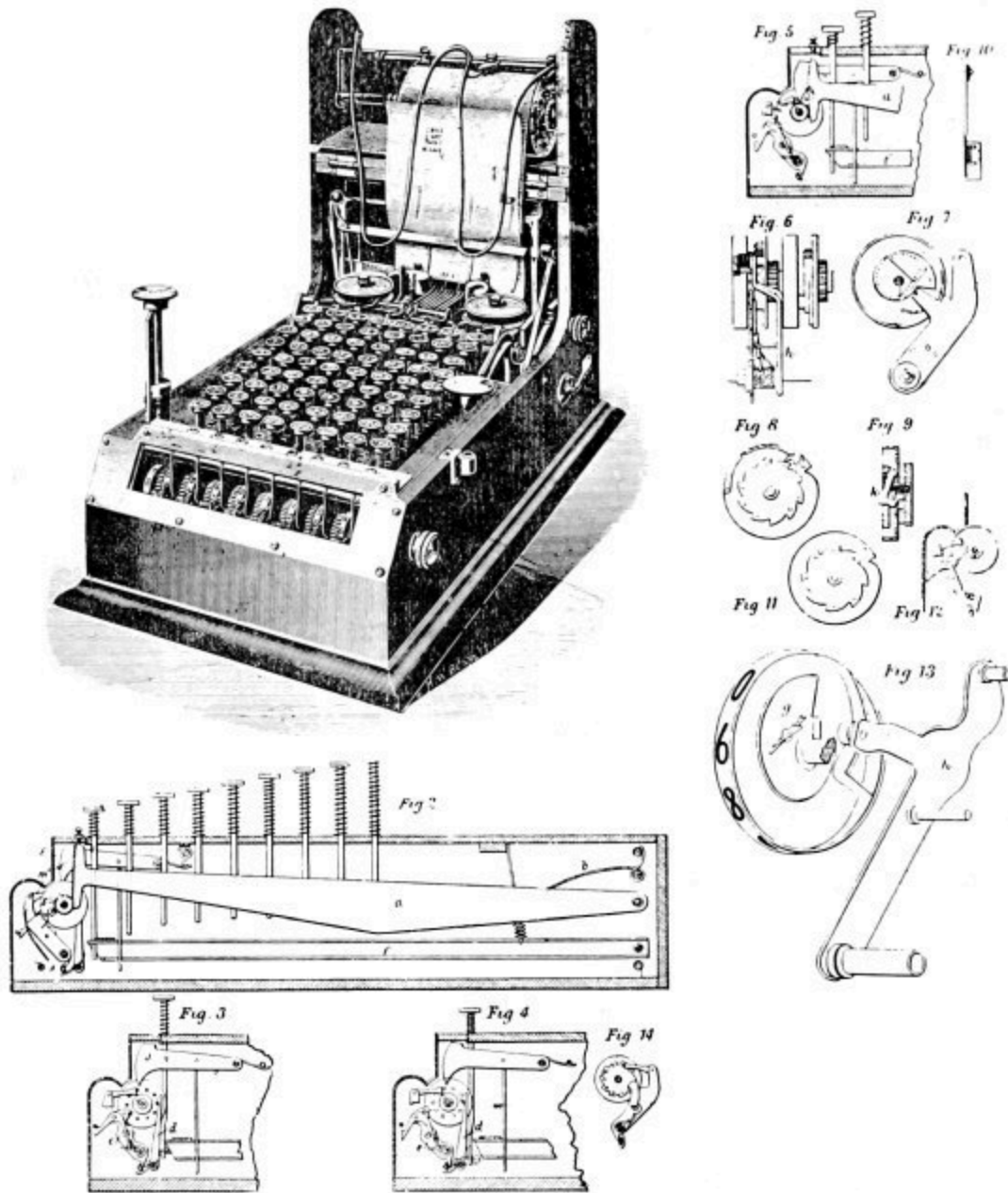
One of the Early “Comptographs”
