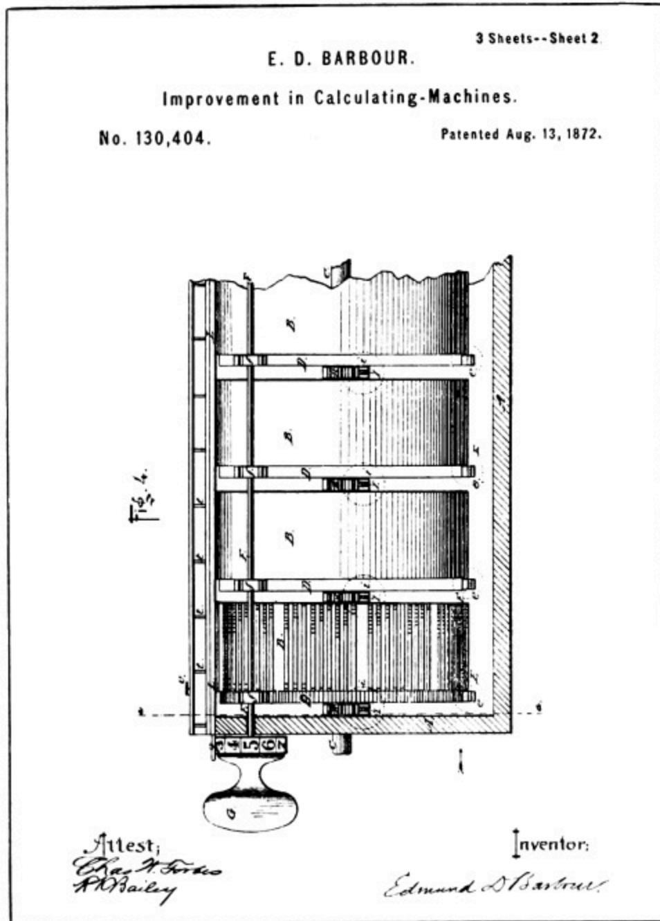
From Drawings of Barbour Patent No. 130,404
