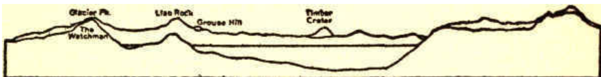
CROSS-SECTION OF CRATER LAKE
