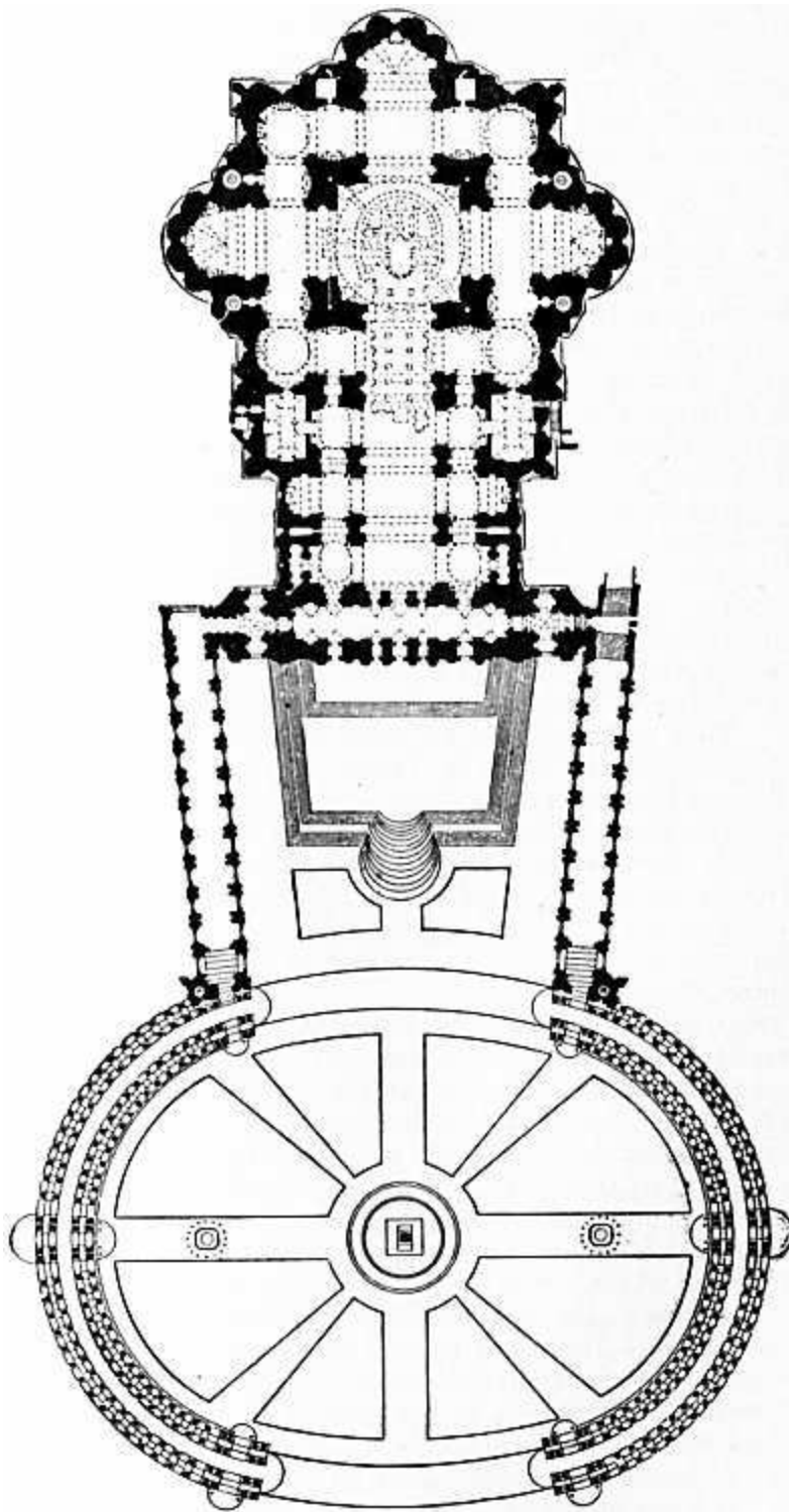
FIG. 51.—Plan of St Peter's at Rome.
