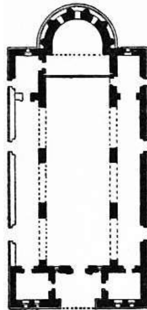
FIG. 31.—Plan of Church of Kalb-Lauzeh.
