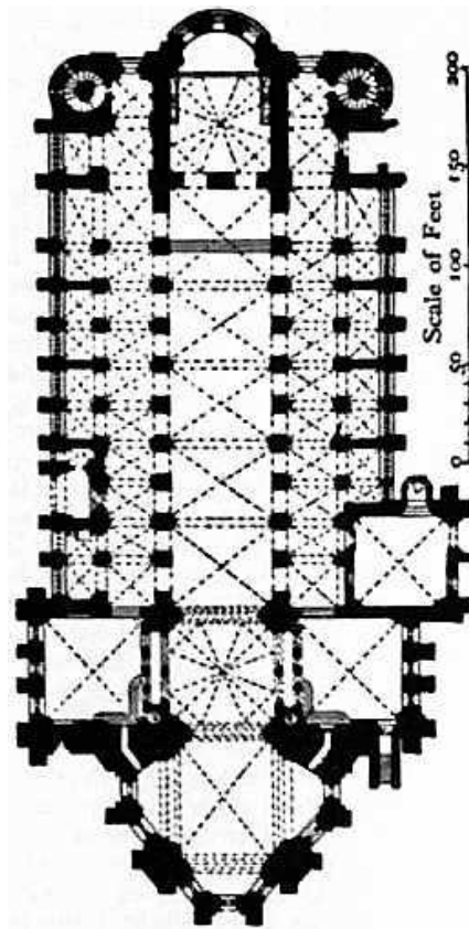
FIG. 45.—Plan of Cathedral at Mainz.
