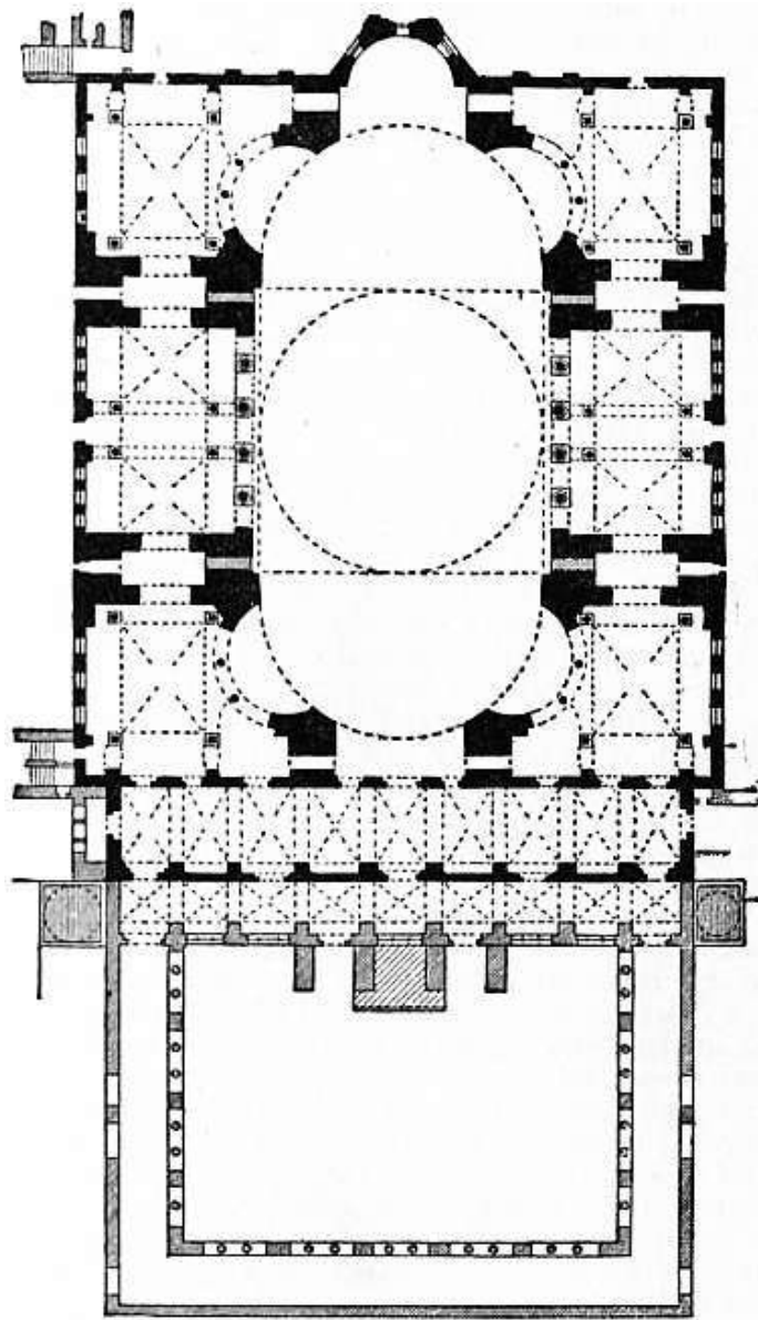
FIG. 28.—Plan of St Sophia.
