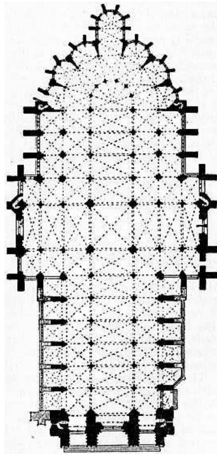
FIG. 40.—Plan of Cathedral at Amiens.
