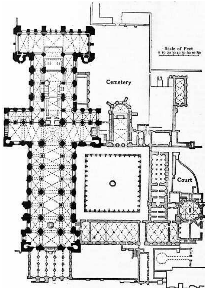
FIG. 42.—Plan of Durham Cathedral.
