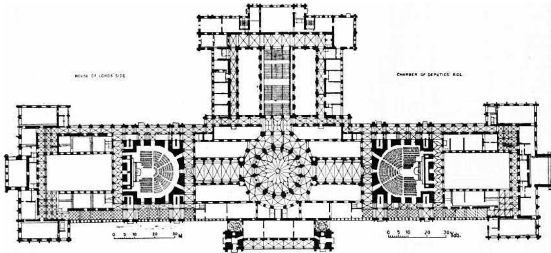
FIG. 92.—Plan of the Parliament House, Budapest. (Steindl.)
