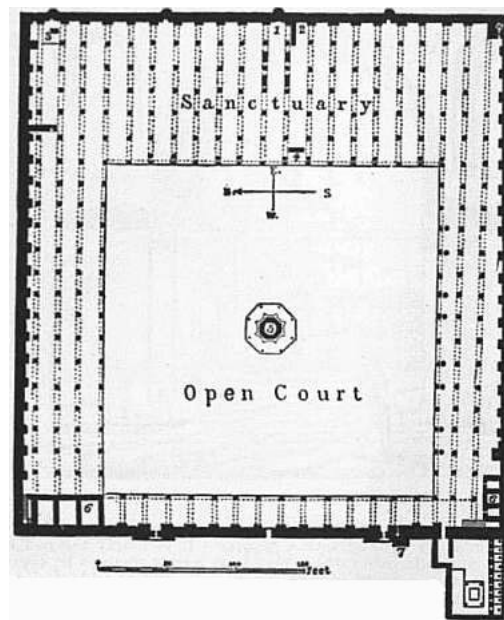
FIG. 54.—Plan of Mosque of 'Amr. Old Cairo.
