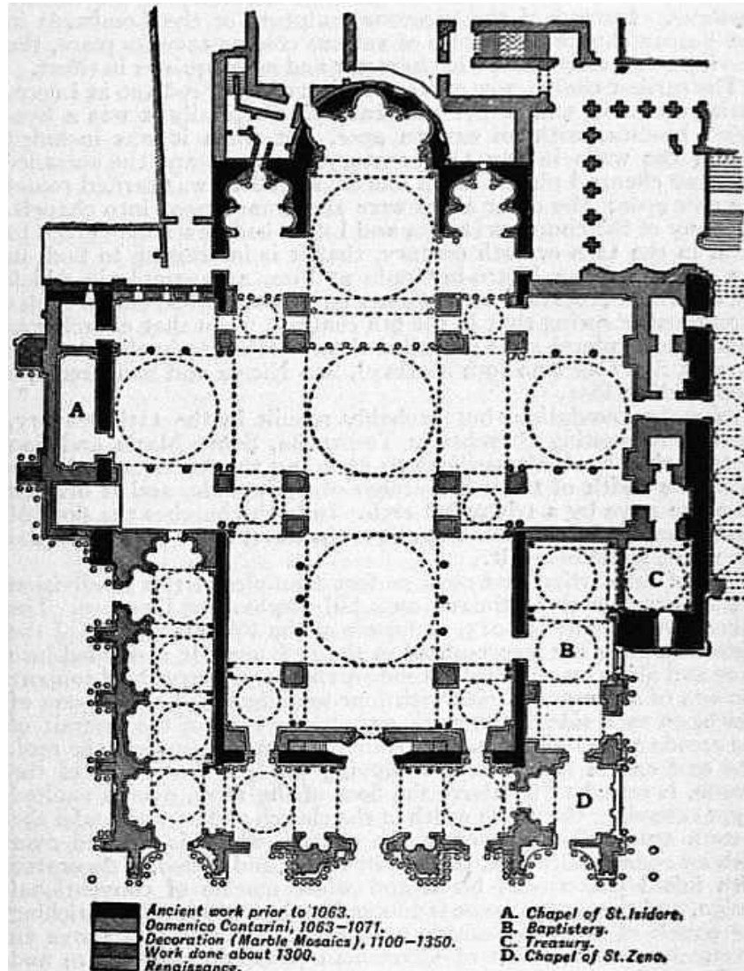
FIG. 37.—Plan of St Mark's, Venice.
