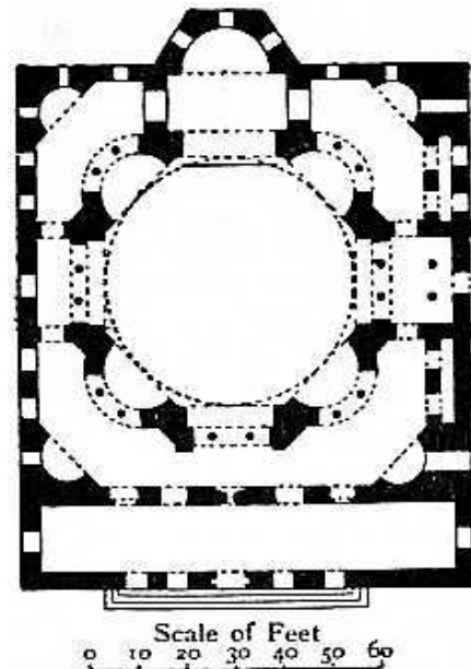
FIG. 27.—Plan of SS. Sergius and Bacchus.
