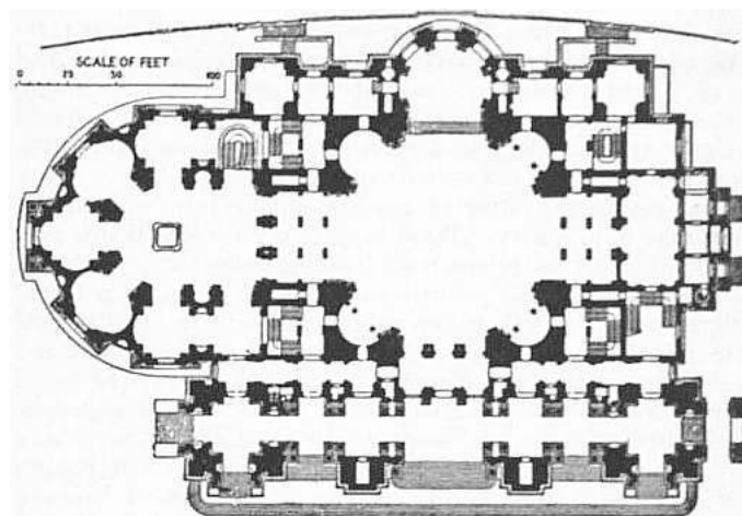
FIG. 112.—Plan of Cathedral at Berlin.
