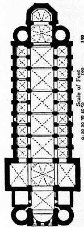
FIG. 46.—Plan of Cathedral at Worms.
