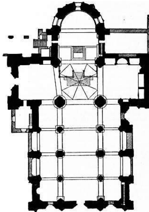
FIG. 36.—Plan of San Michele Pavia.
