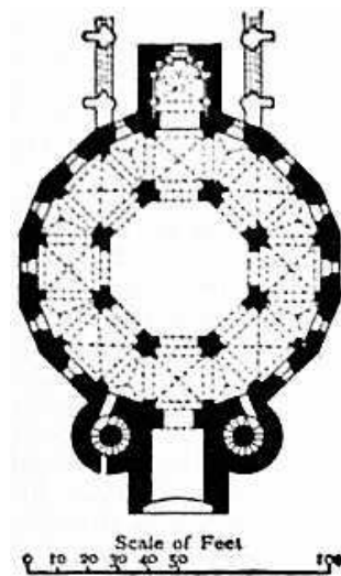
FIG. 44.—Plan of Cathedral at Aix-la-Chapelle.
