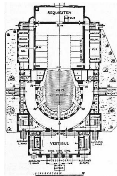
FIG. 114.—Plan of Lessing Theatre, Berlin.
