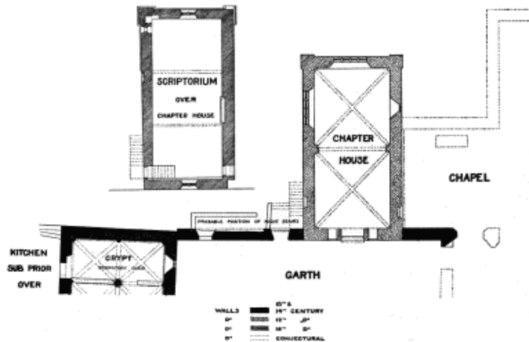
PLAN OF SCRIPTORIUM, BIRKENHEAD PRIORY
