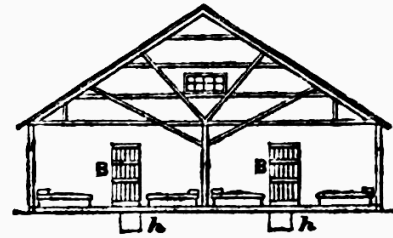
Transverse Section.
