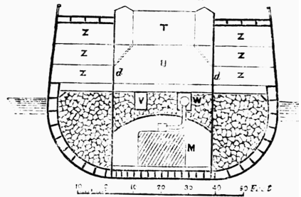
Midship Section showing Cabins & Boiler Room.
