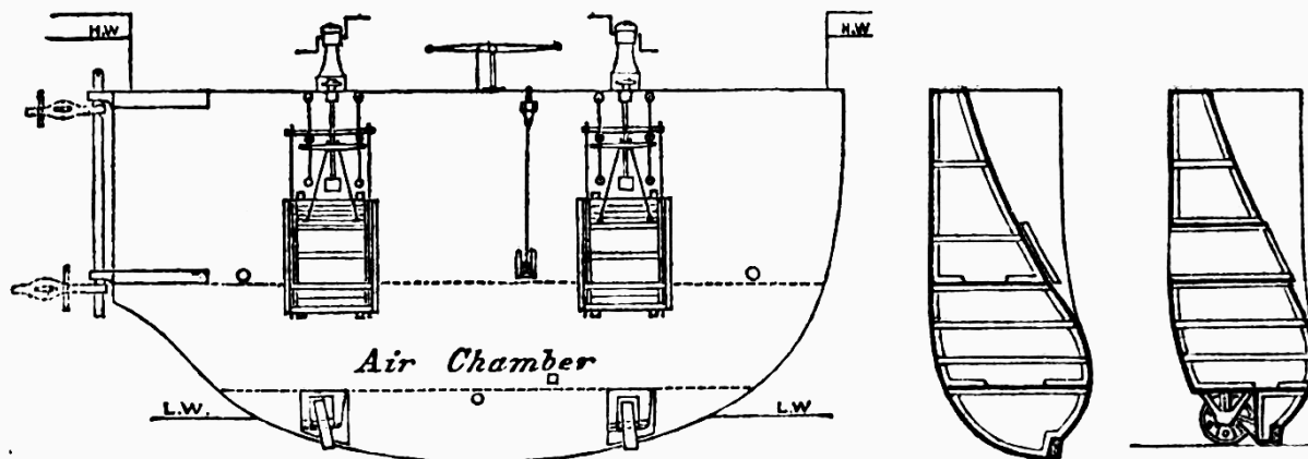
Fig. 18. Bristol Dock Gate.
