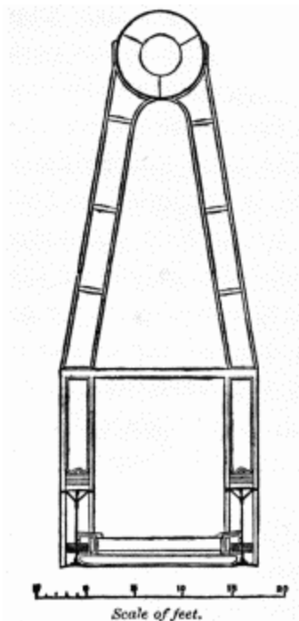
Fig. 11. Truss of Chepstow Bridge. Transverse Section.
