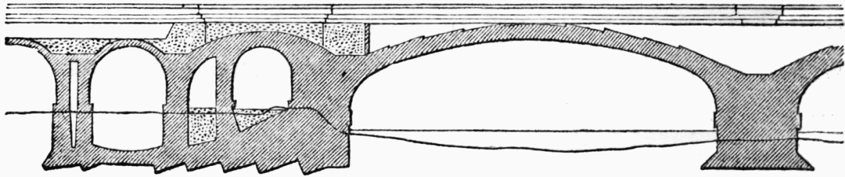
Fig. 1. Maidenhead Bridge. Longitudinal Section.
