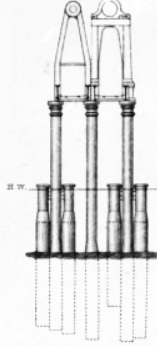
CHEPSTOW BRIDGE. Transverse Section at Middle of Span at Middle Pier
