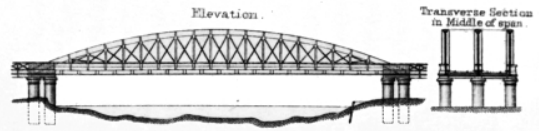
WINDSOR BRIDGE.
