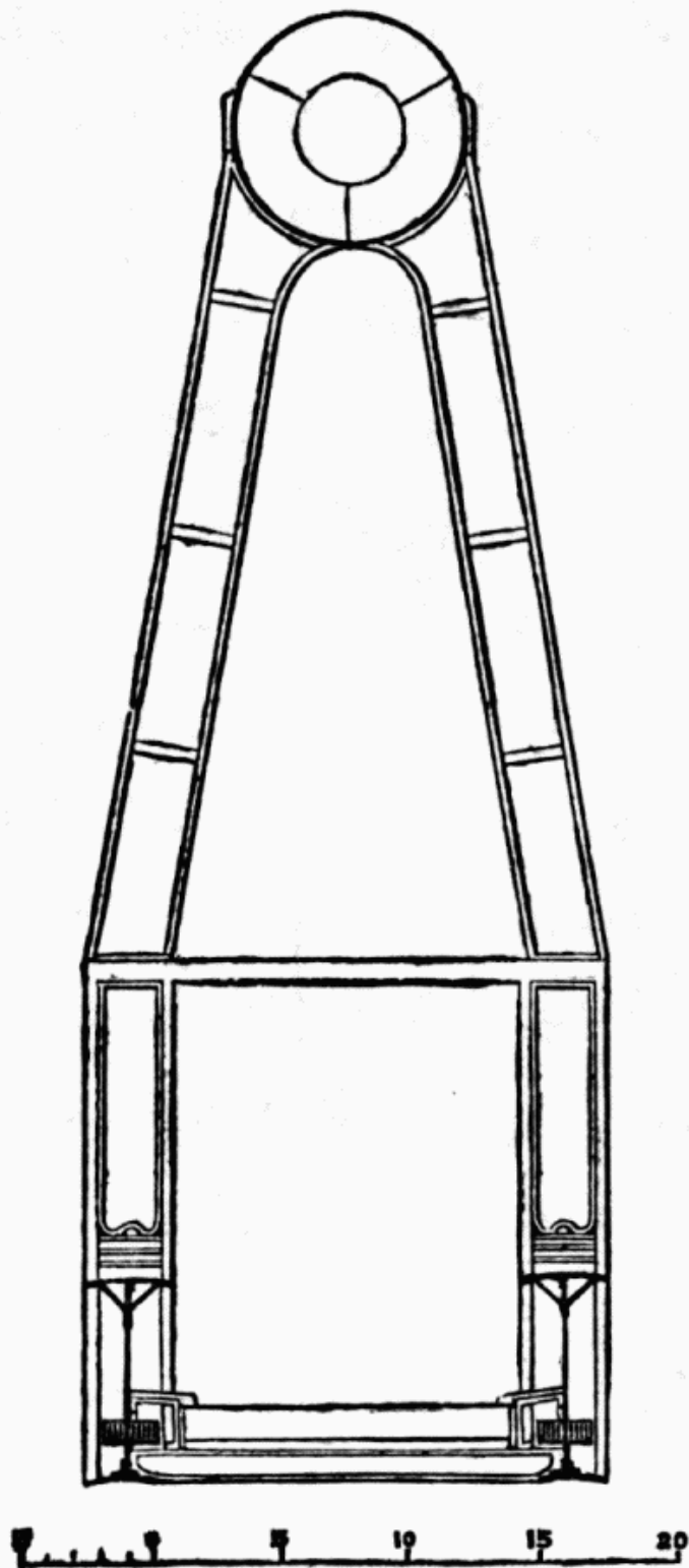
Fig. 11. Truss of Chepstow Bridge. Transverse Section.
