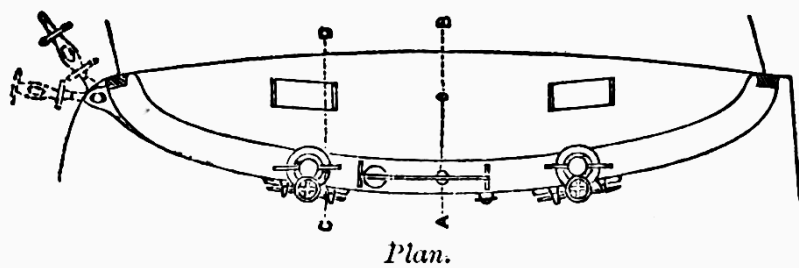
Fig. 18. Bristol Dock Gate.
