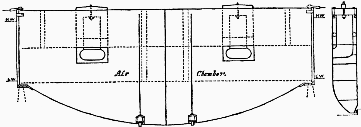
Fig. 19. Plymouth Dock Gates. Elevation.
