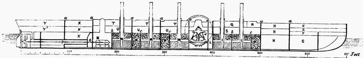
Plan showing Machinery and Coals
