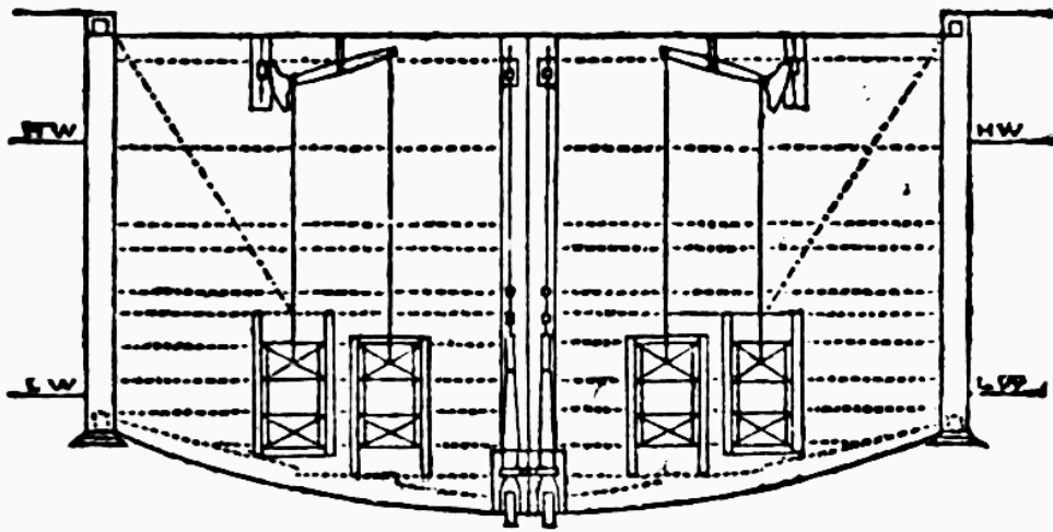
Fig. 17. Monkwearmouth Dock Gates, Elevation.
