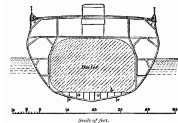
Fig. 13. 'Great Britain' Steam-Ship.
