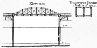
CHEPSTOW BRIDGE. Elevation.
