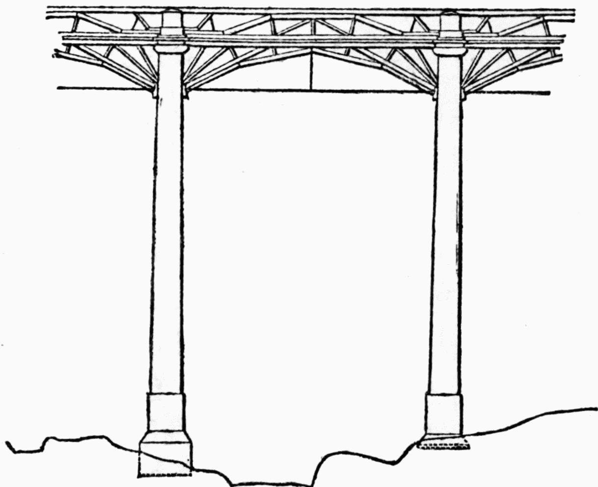
Fig. 3. Ivybridge Viaduct.
