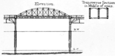
CHEPSTOW BRIDGE.
