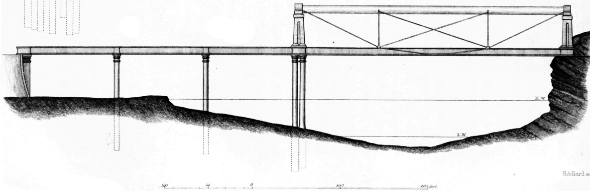
CHEPSTOW BRIDGE. Elevation.
