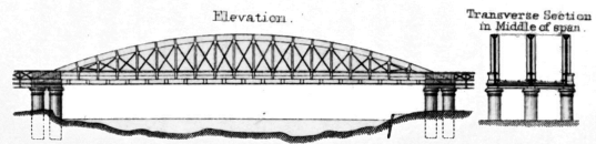
WINDSOR BRIDGE.
