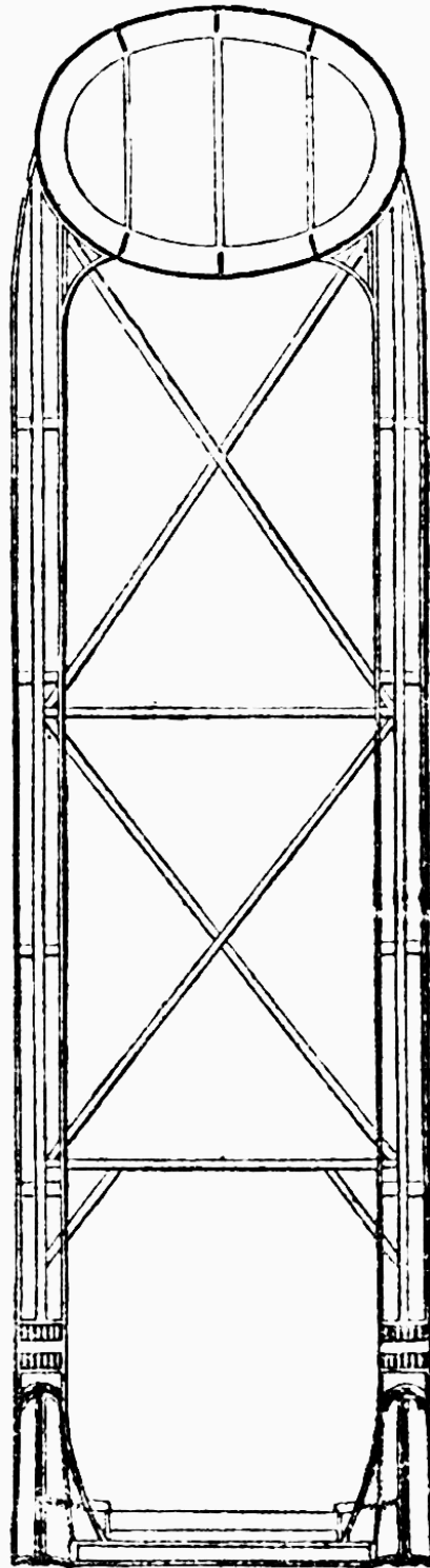
Fig. 12. Truss of Saltash Bridge. Transverse section.
