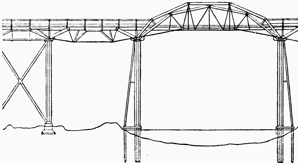
Fig. 4. Landore Viaduct.
