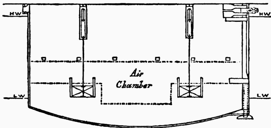
Fig. 20. Briton Ferry Dock Gate. Elevation.
