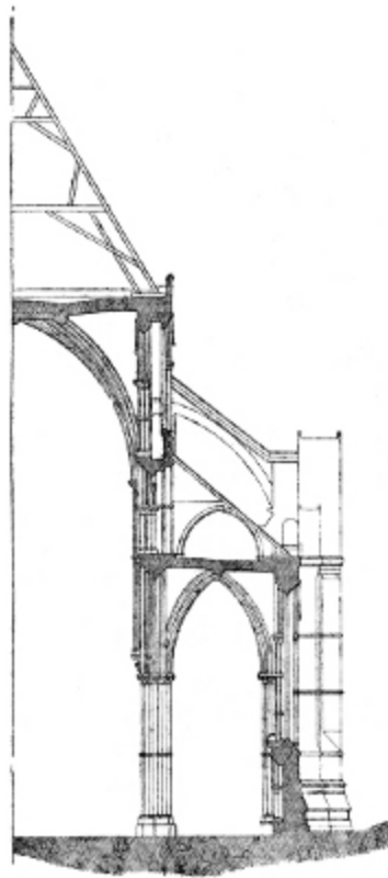
HALF SECTION OF THE NAVE, LOOKING WEST.
