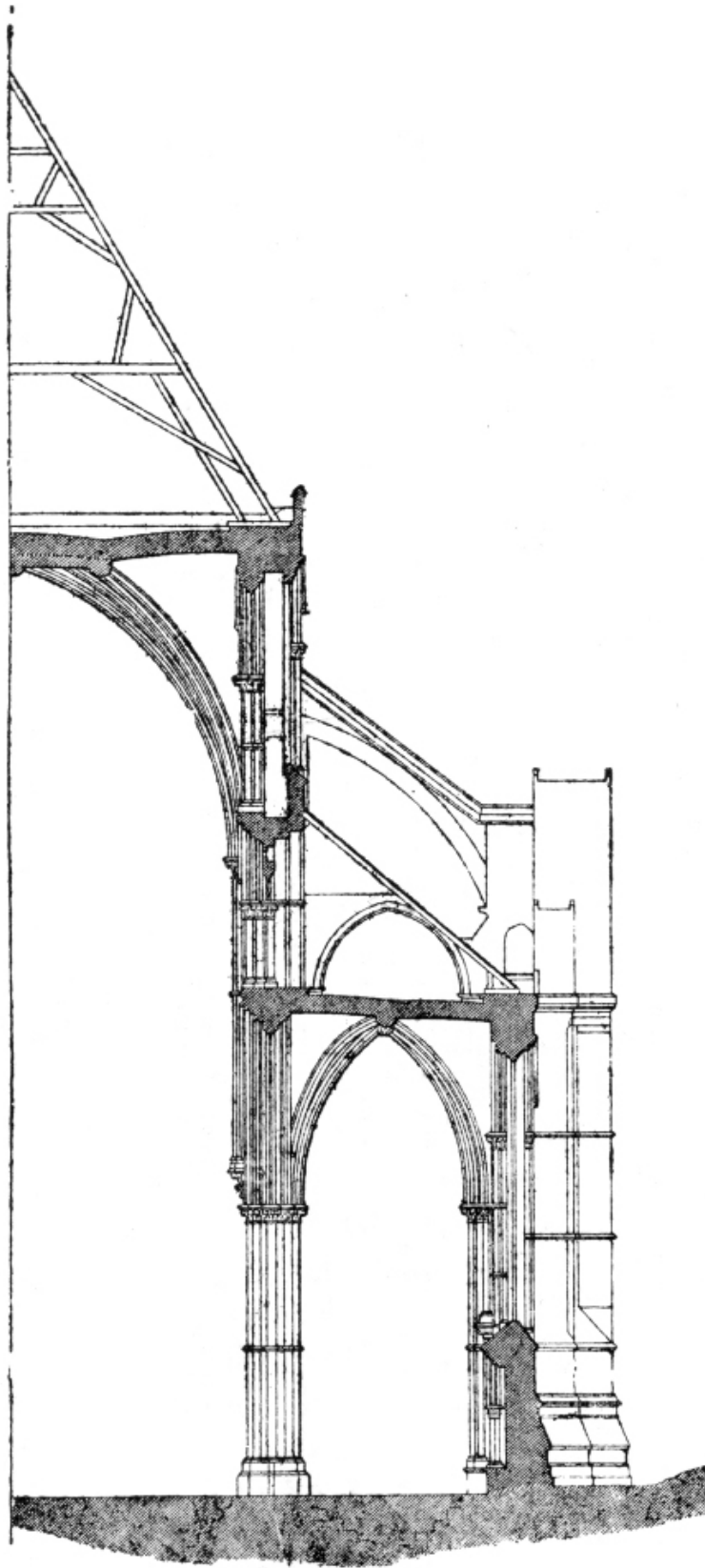
HALF SECTION OF THE NAVE, LOOKING WEST.
