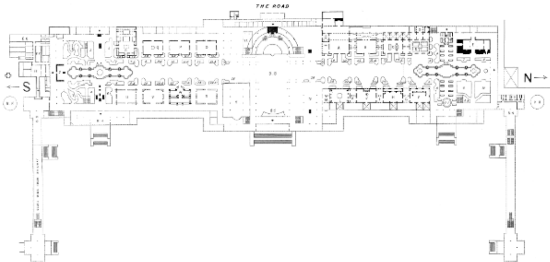
GROUND PLAN OF THE CRYSTAL PALACE.
