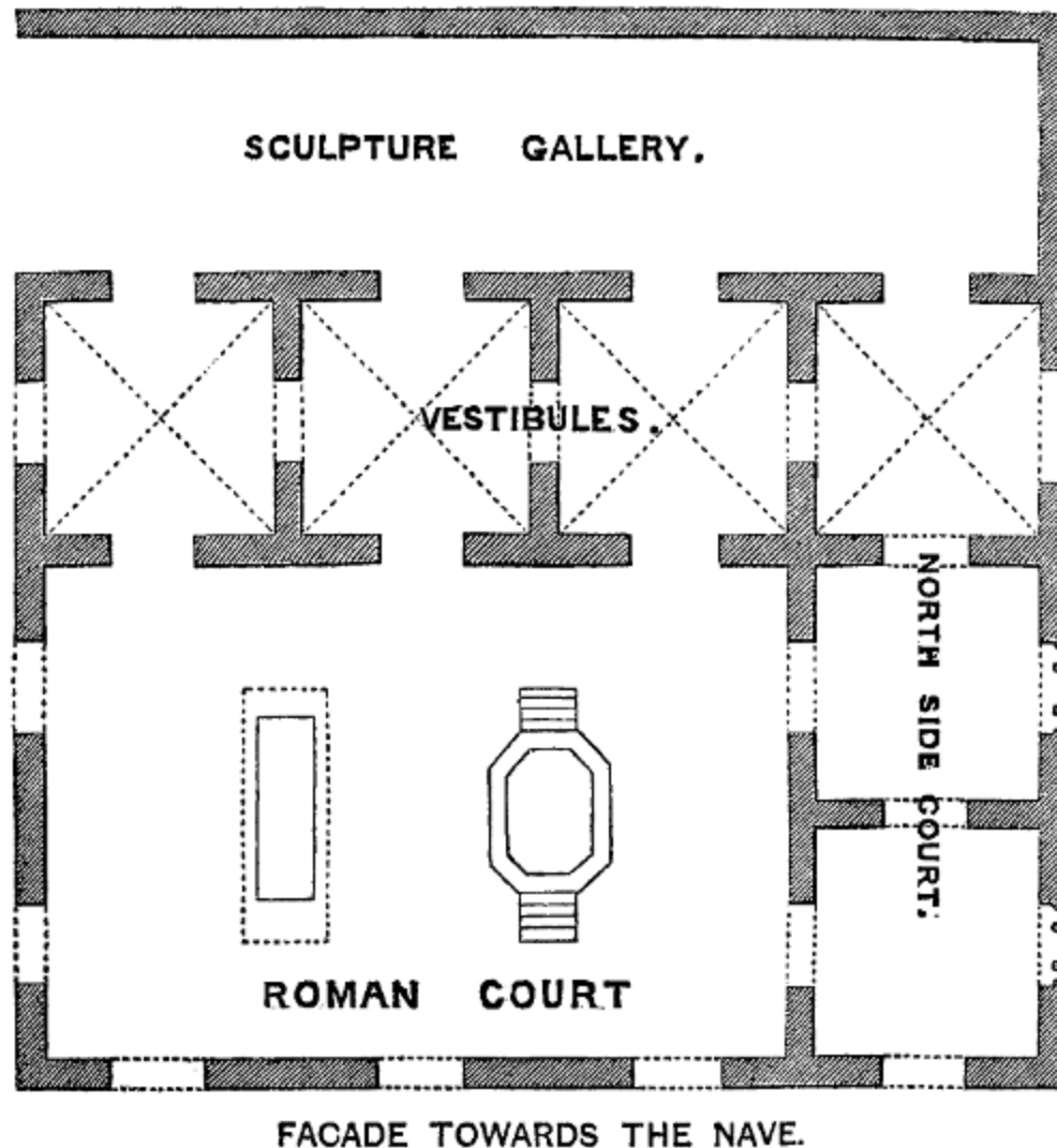
Plan of the Roman Court.
