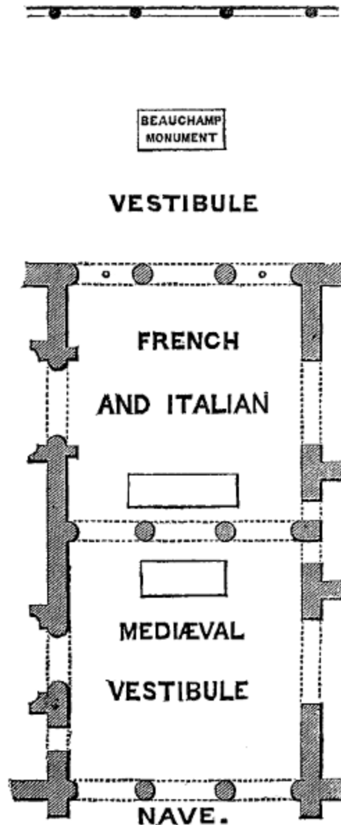
Plan of the French and Italian Mediæval Vestibule.
