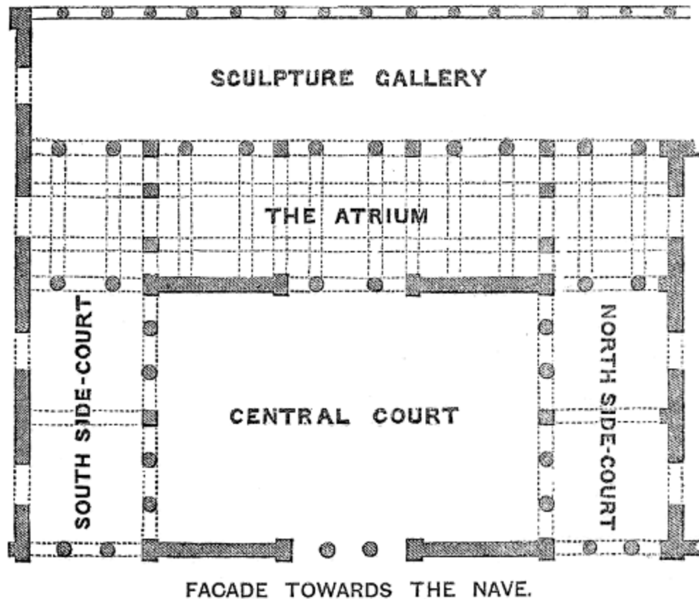
Plan of the Greek Court.
