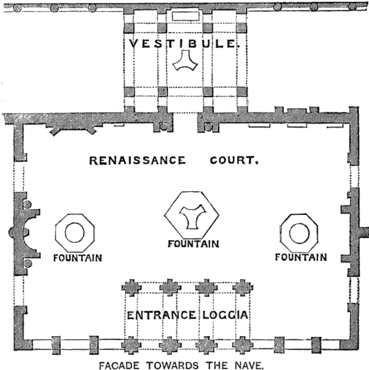
Plan of the Renaissance Court.
