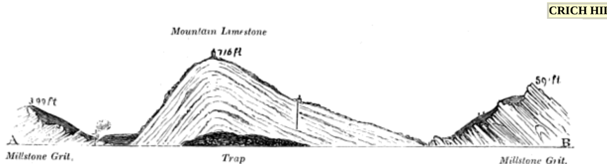
LIGN. 274. SECTION OF CRICH HILL; from A to B on the plan, Lign. 273 . (Natural scale.)
