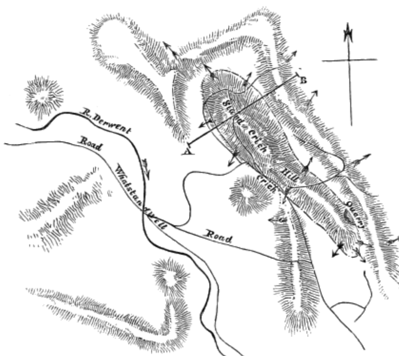
LIGN. 273. GROUND PLAN OF CRICH HILL, Derbyshire. (Scale, one inch to a mile. ) By HENRY CARR, Esq. C. E. from actual Survey.
