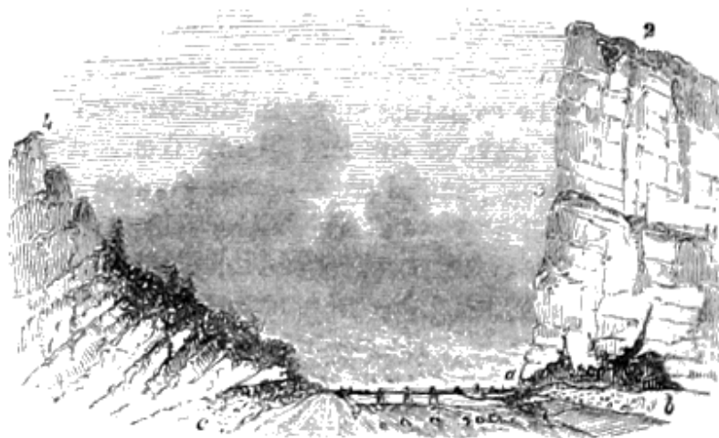
LIGN. 270. SECTION ACROSS THE VALLEY OF THE DERWENT, AT THE HIGH TOR, MATLOCK.
