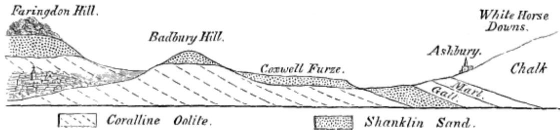
LIGN. 269. SECTION OF THE STRATA AT FARRINGTON, BERKS; from FARRINGTON HILL to the CHALK DOWNS on the South.
