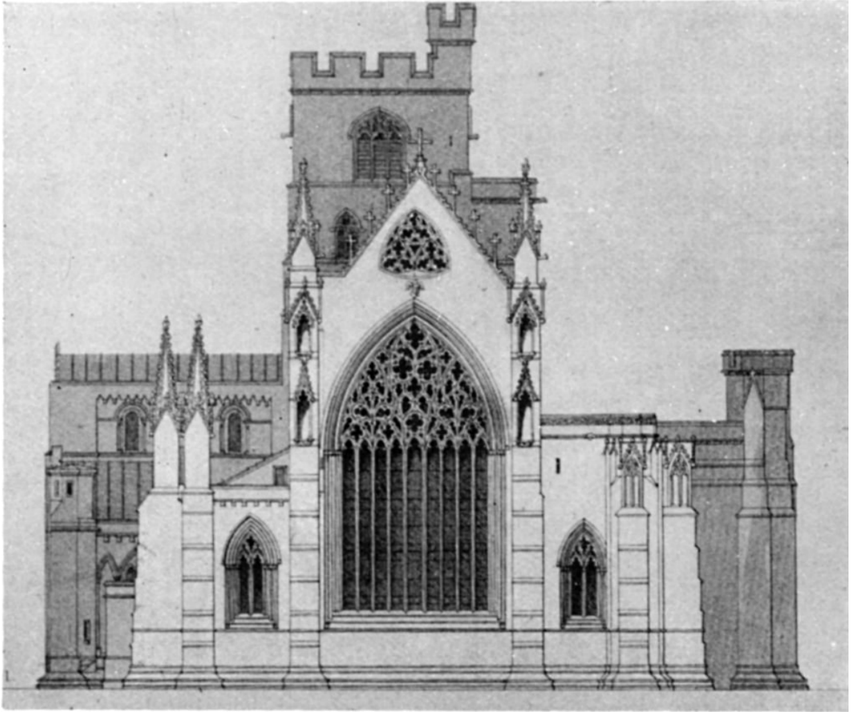
ELEVATION OF EAST END.
