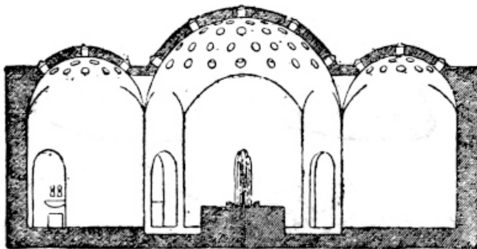
SECTION OF THE HARÁRAH.
