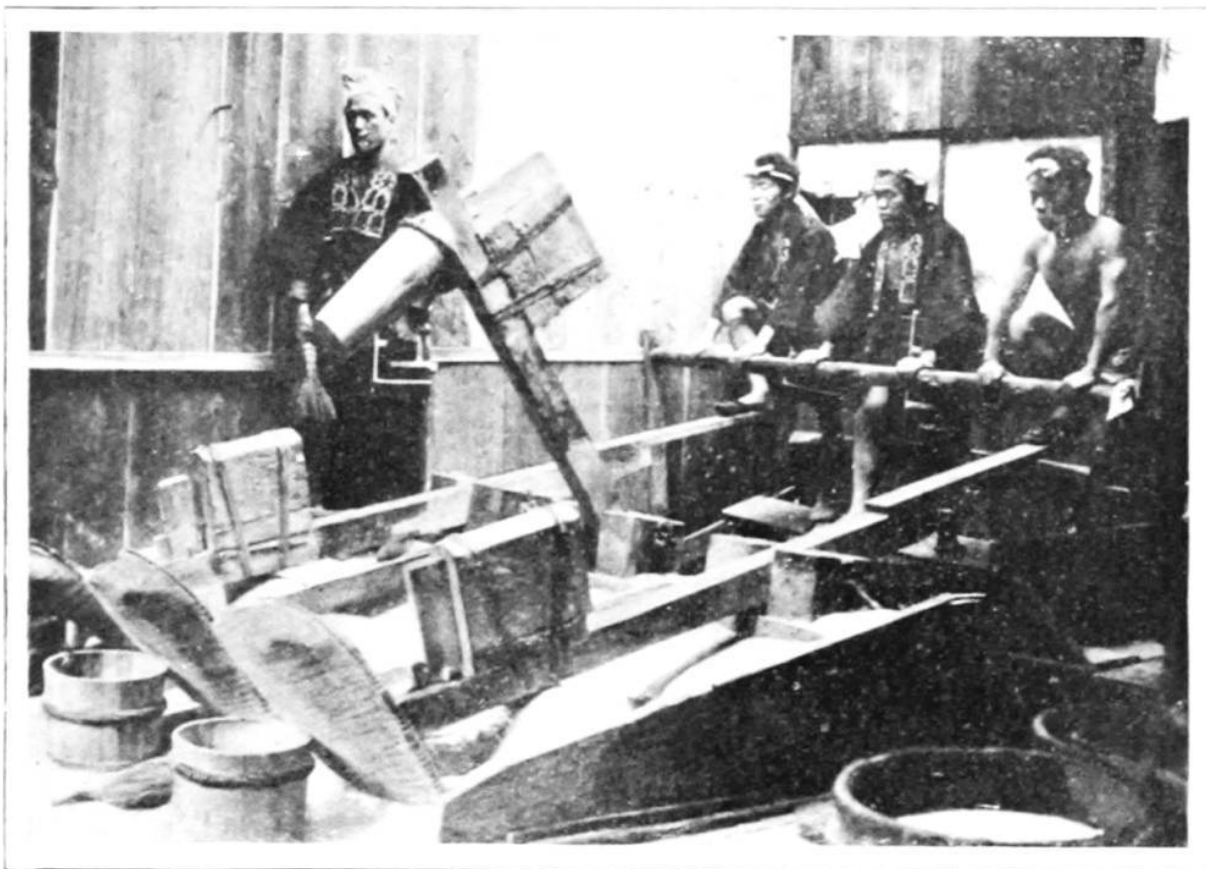
THE PROCESSES OF WEIGHING AND POUNDING RICE
