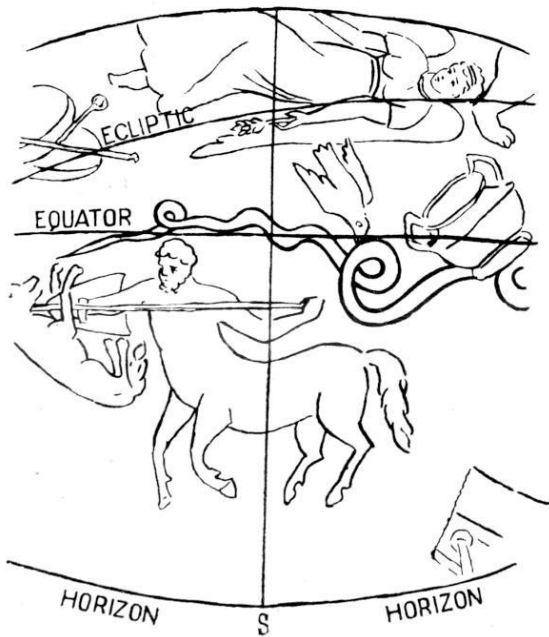
3,589 B.C. Lat. 35° N. Constellations above Southern Horizon. Invisible—Noon, 7th Month, Calendrical Year. Visible—Midnight, beginning Calendrical Year.
