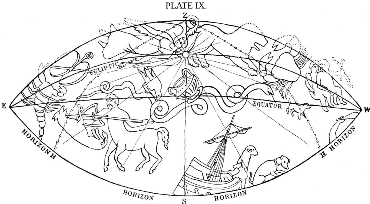
Position of the Sun amongst the Constellations at Summer Solstice, 4,000 B.C. Observer in Lat. 40° N.
