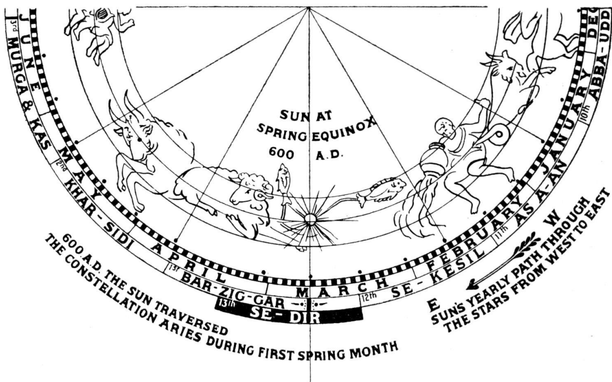
The first and last months of the Accadian, sidereal, year, compared with the months of the Gregorian, tropical, year: at 6,000 B.C. and at 600 A.D.
