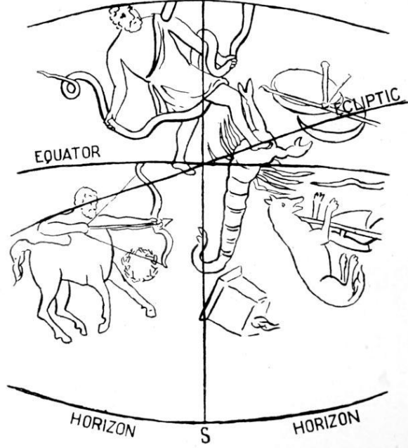
3,589 B.C. Lat. 35° N. Constellations above Southern Horizon. Invisible—Noon, Autumn Equinox. Visible—Midnight, Spring Equinox.
