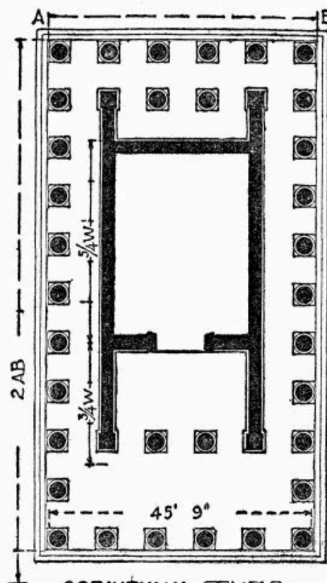
CORINTHIAN TEMPLE AT LABRANDA
