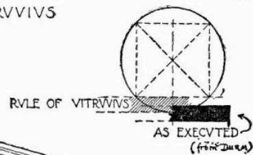
THEATRE AT OROPVS
