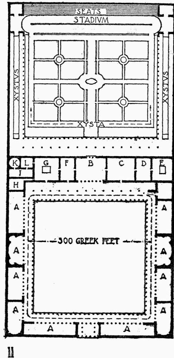
I. THE PALAESTRA AT OLYMPIA II. THE GREEK PALAESTRA ACCORD- ING TO VITRUVIUS
