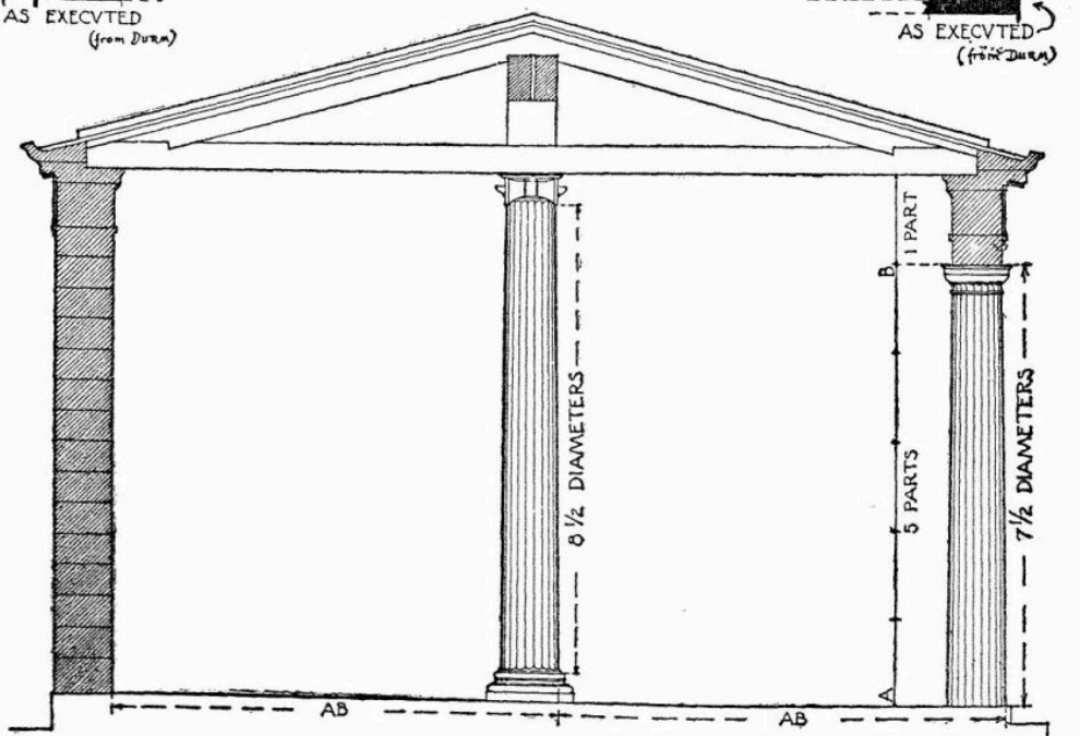
THE THEATRE PORTICO ACCORDING TO VITRUVIUS
