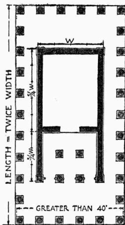
ACCORDING TO VITRUVIUS
