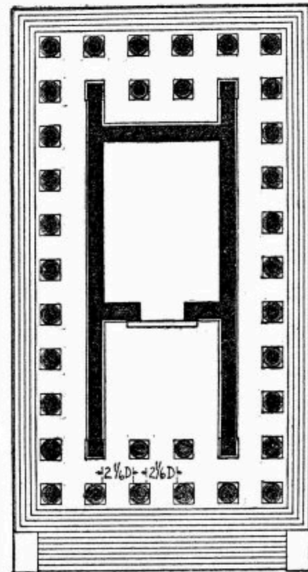
THE TEMPLE AT TEOS IN ASIA MINOR
