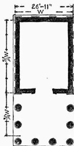
TEMPLE OF HERCULES AT CORI
