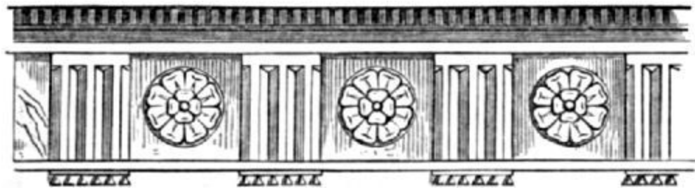
Fig. 7. Metopes and Triglyphs.
