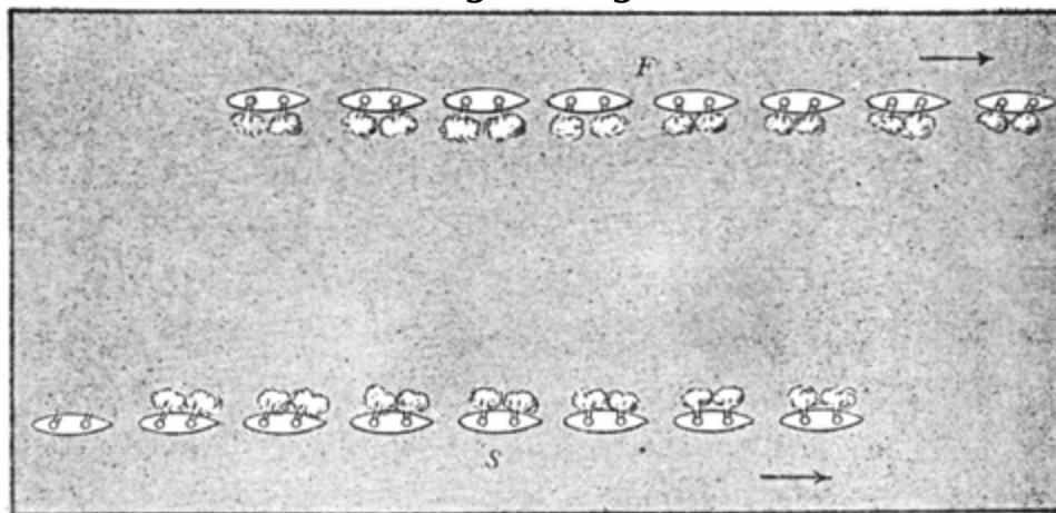
Fig. 2.--The faster fleet, F, forges ahead, concentrating the fire of both its front ships on the van ship of the slow fleet, while the rear ship of fleet S is thrown out of range and out of action.
