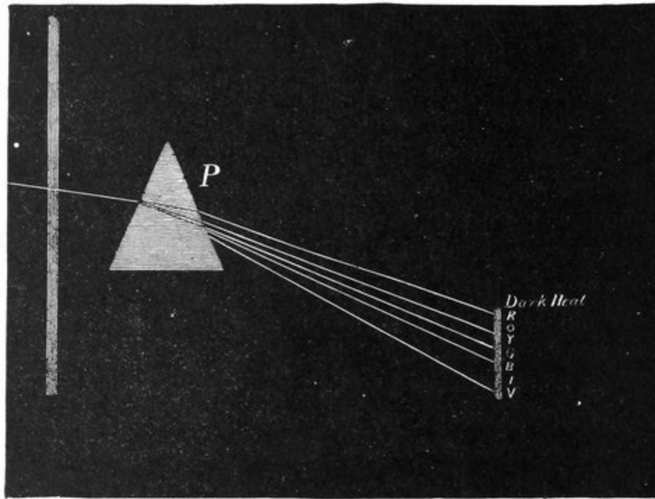
FIG. 85.—How to split up a Ray of Light.
