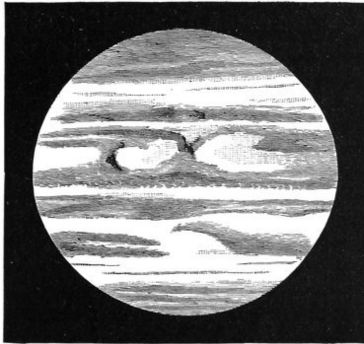
FIG. 67.—The Clouds of Jupiter.
