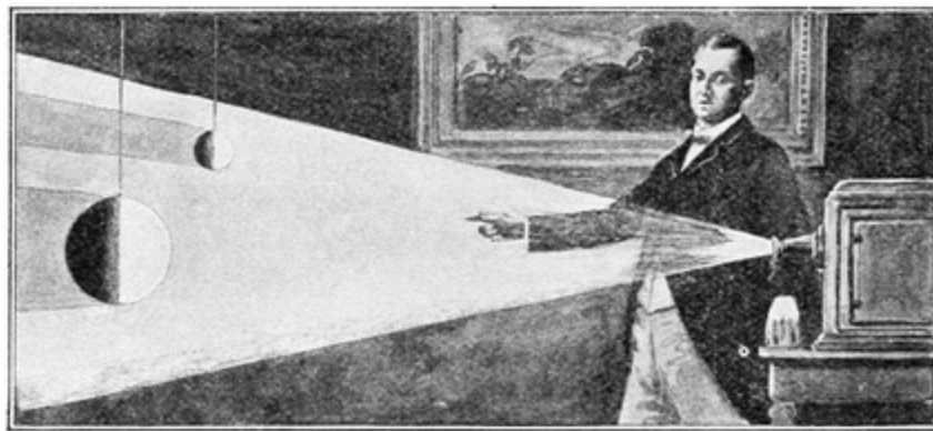
FIG. 28.—To show that the Moon is lighted by Sunbeams.
