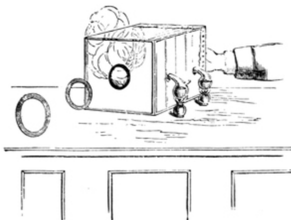
FIG. 88.—How to make the Smoke-rings.
