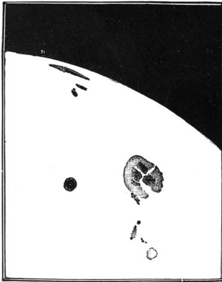
FIG. 16.—Spot nearing the Sun's Edge.
