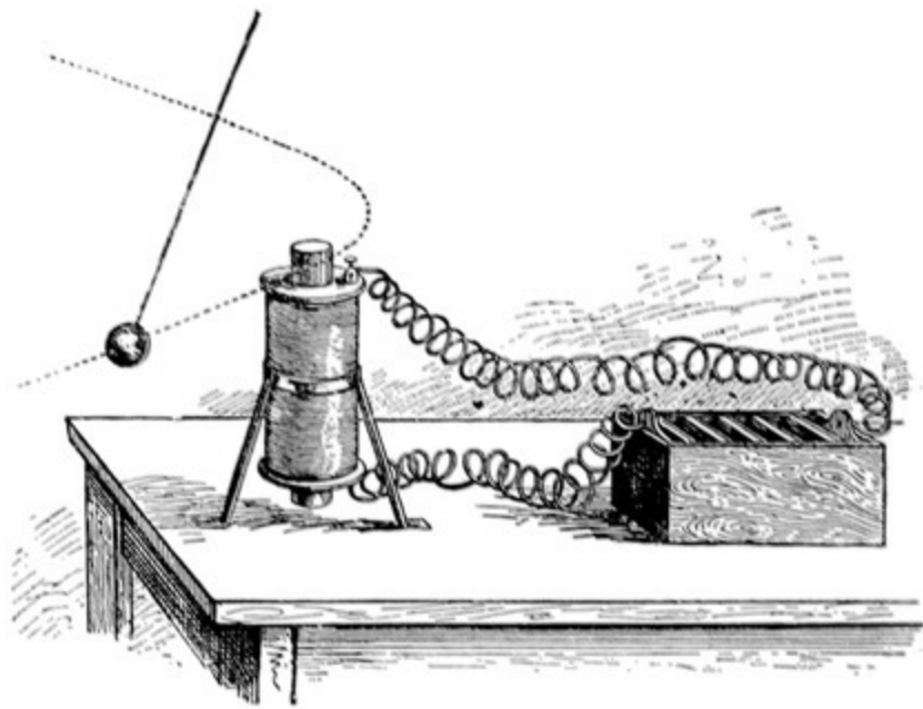
FIG. 59.—The Effect of Attraction.
