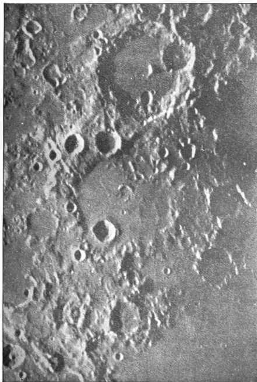
FIG. 41.—View on the Moon.
