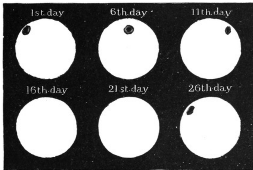
FIG. 17.—How the Sun turns round.
