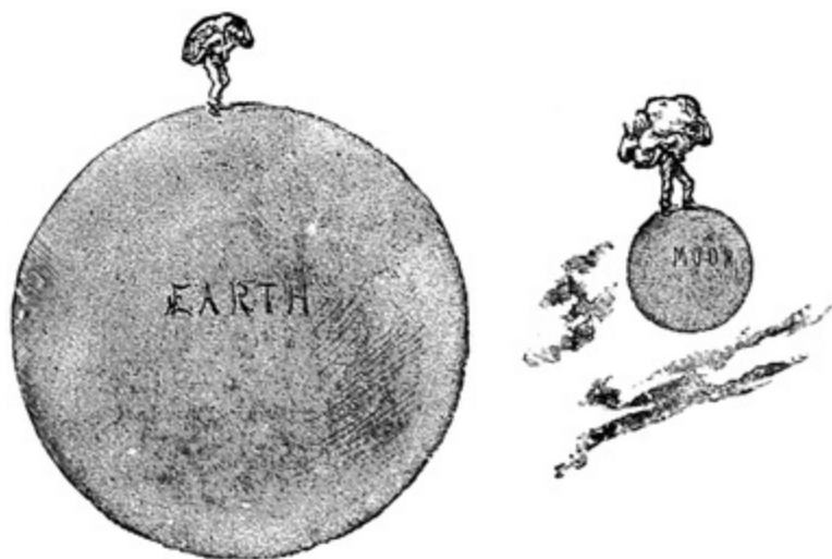
FIG. 45.—The Lessened Gravitation on the Moon.
