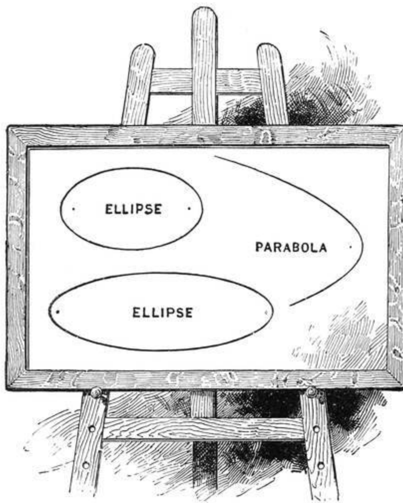
FIG. 55.—Specimens of Ellipses.
