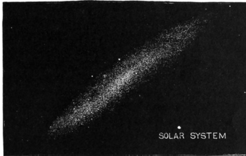
FIG. 91.—To show how Small the Solar System is compared with a Great Nebula.
