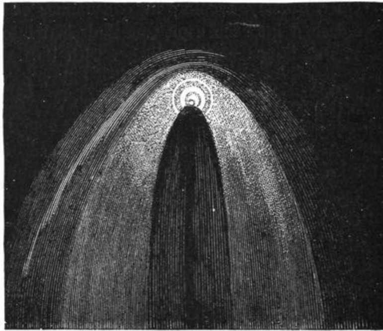
FIG. 76.—How the Tail of a Comet arises.
