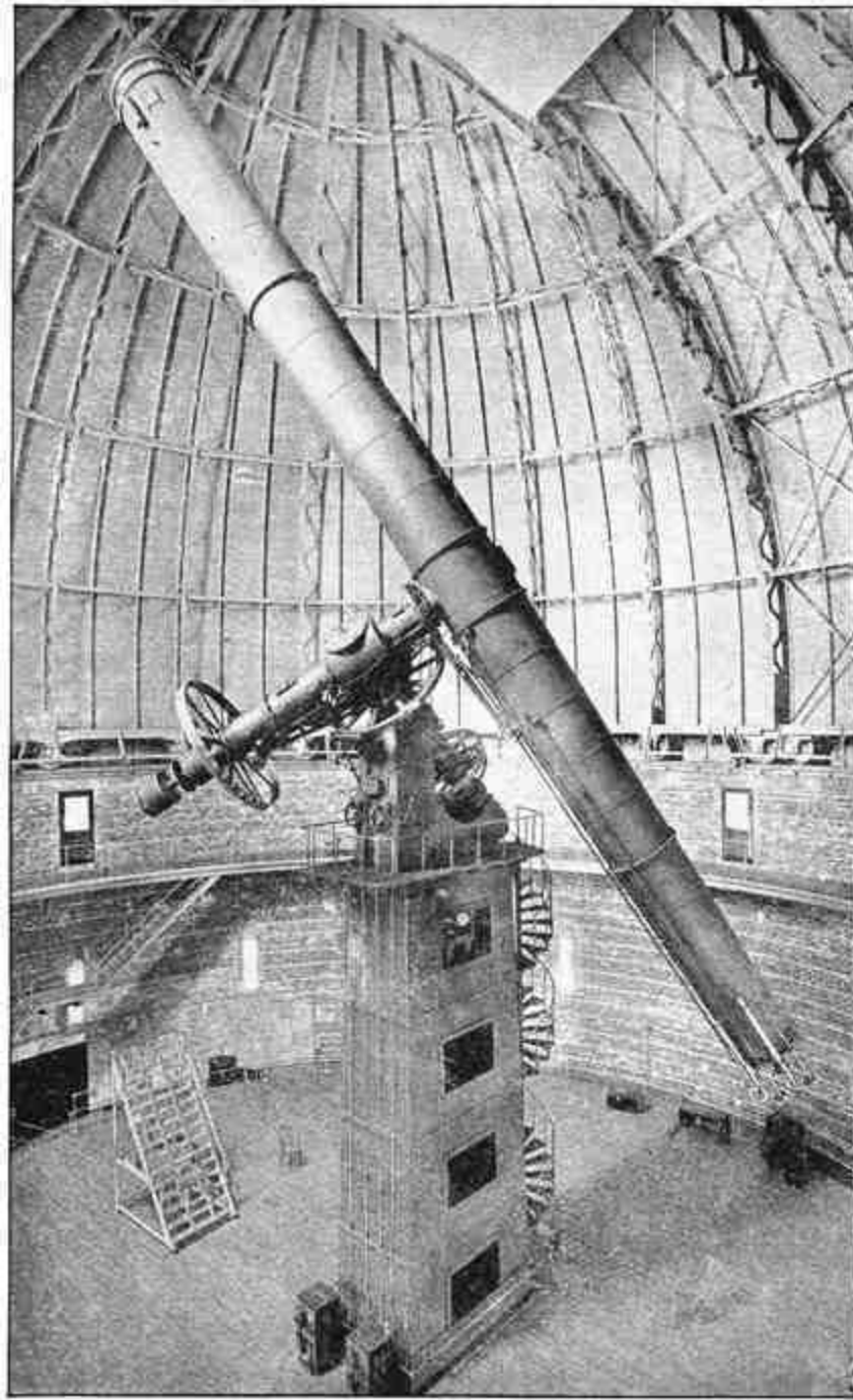
FIG. 38.—The Yerkes Telescope, University of Chicago.
