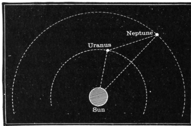
FIG. 71.—Orbits of Uranus and Neptune.
