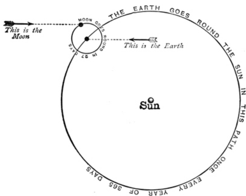
FIG. 33.—To show how the Earth goes round the Sun and the Moon round the Earth.
