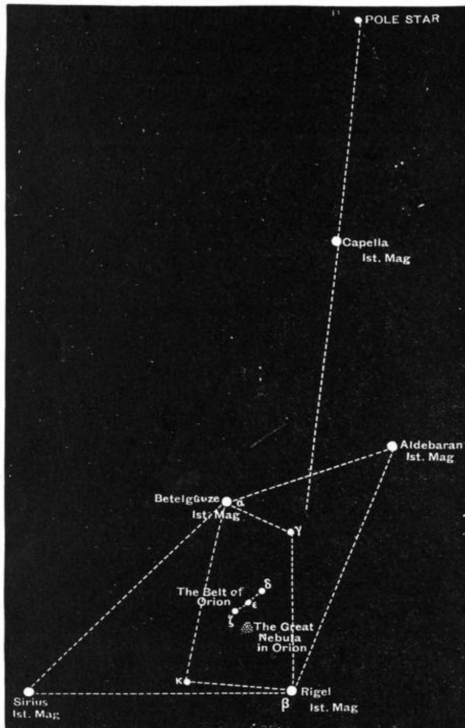
FIG. 94.—Orion and Sirius.
