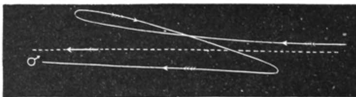
FIG. 53.—A Specimen of the Track of Mars.
