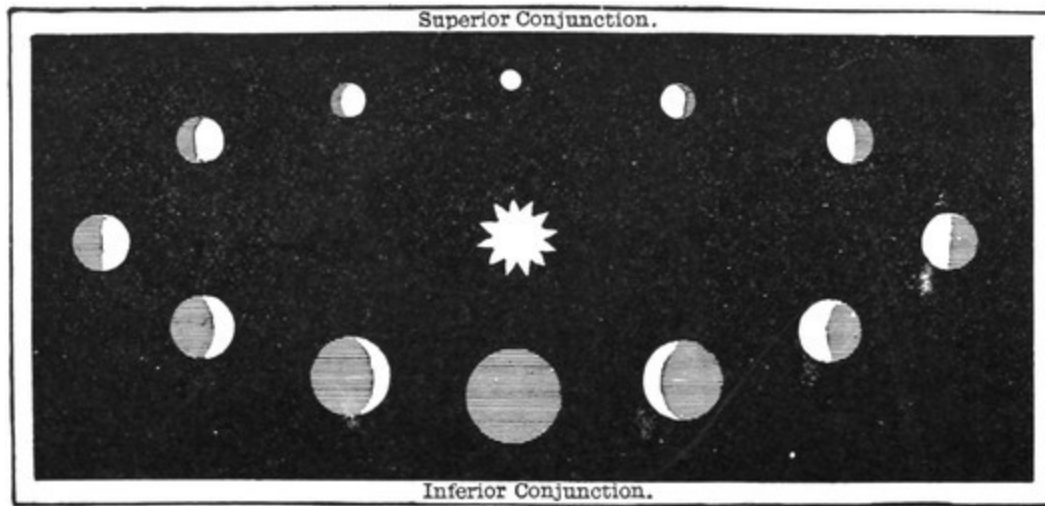
FIG. 48.—Phases of an Inferior Planet.
