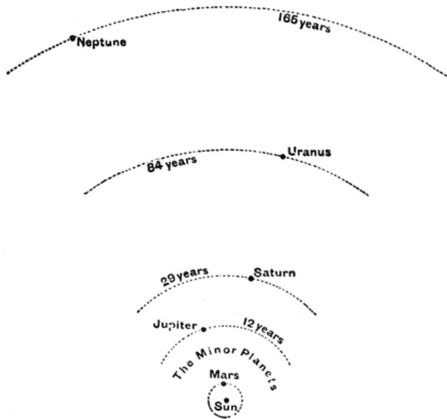
FIG. 65.—The Orbits of the Four Giant Planets.
