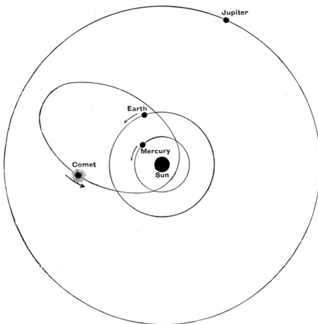
FIG. 73.—The Orbit of Encke's Comet.
