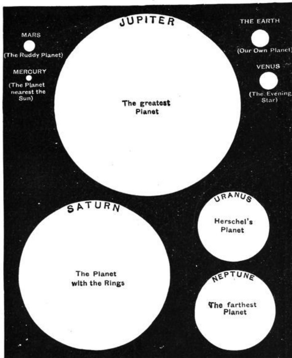
FIG. 47.—Comparative Sizes of the Planets.
