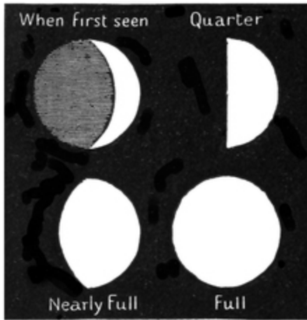
FIG. 31.—The Changes in the Moon.
