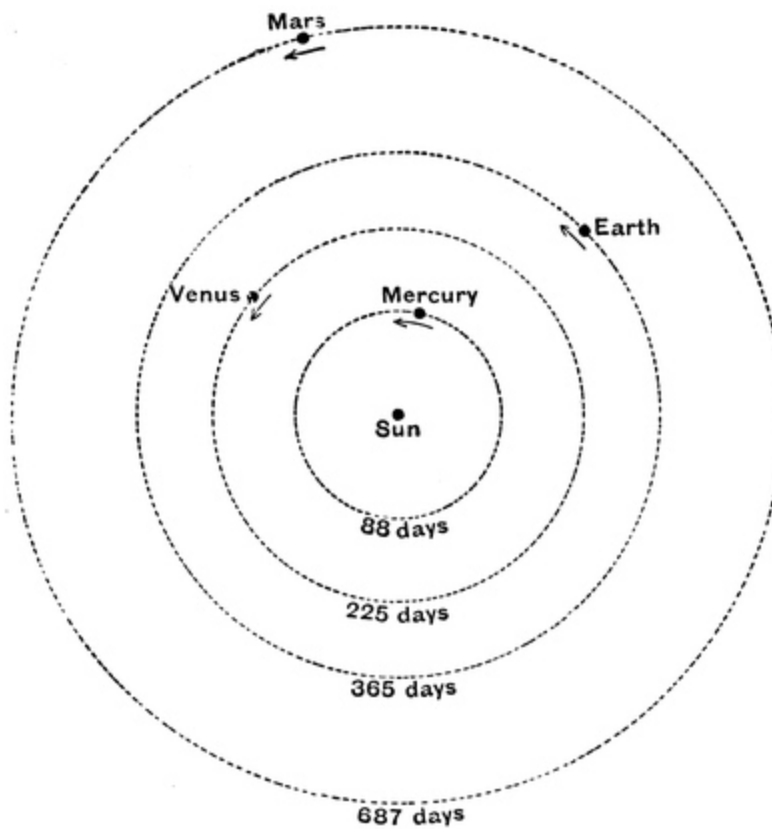
FIG. 46.—The Orbits of the Four Inner Planets.
