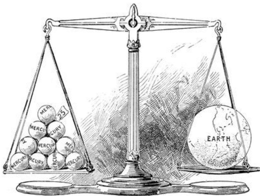
FIG. 49.—Relative Weights of Mercury and the Earth.
