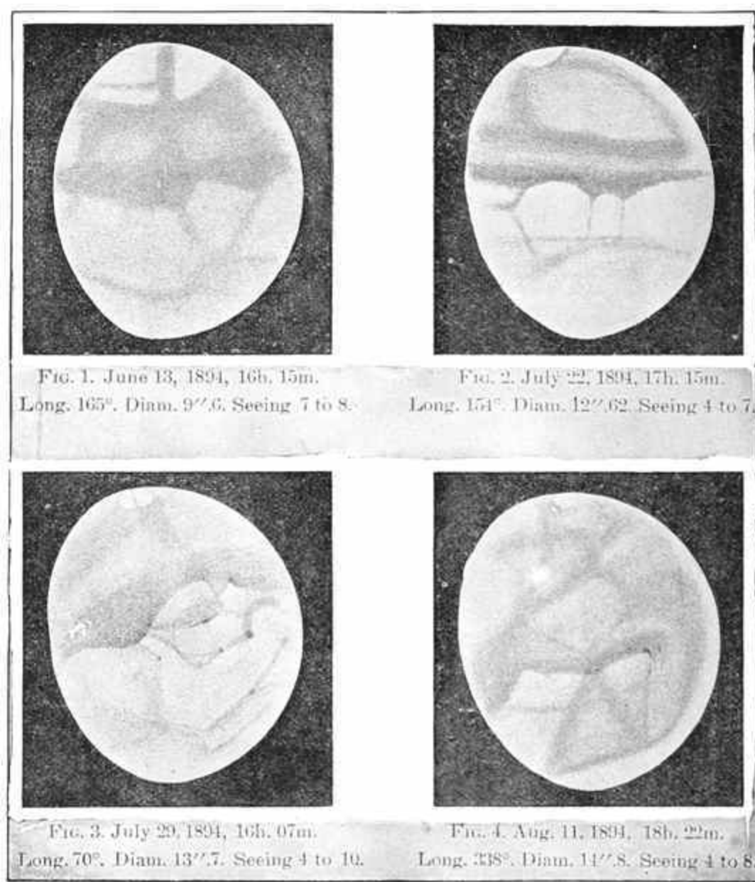
FIG. 61.—Mars.
