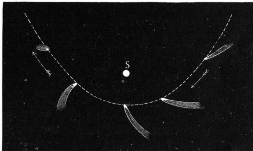
FIG. 72.—How the Comet's Tail is disposed.
