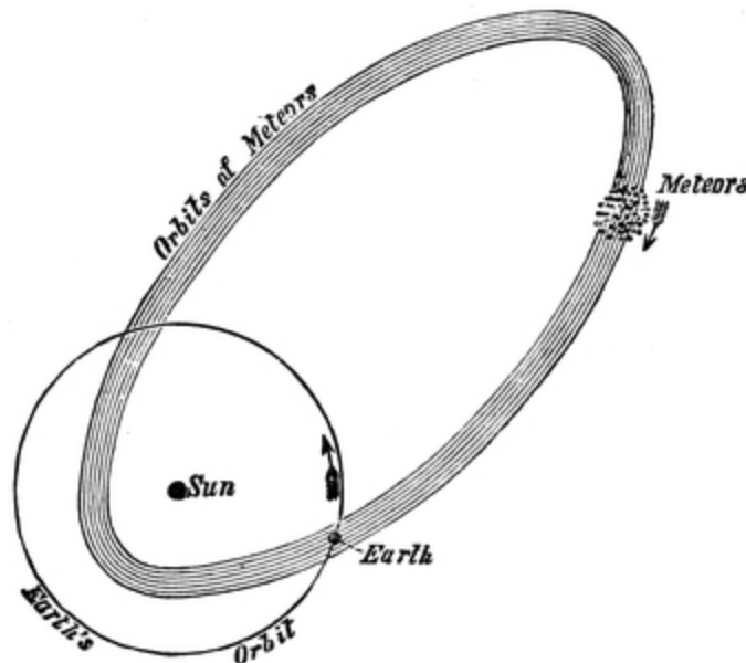
FIG. 80.—The Earth crossing the Track of Meteors.
