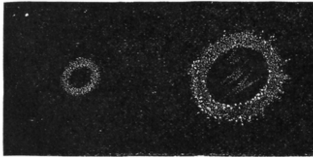
FIG. 86.—The Ring Nebula in Lyra, under Different Telescopic Powers.
