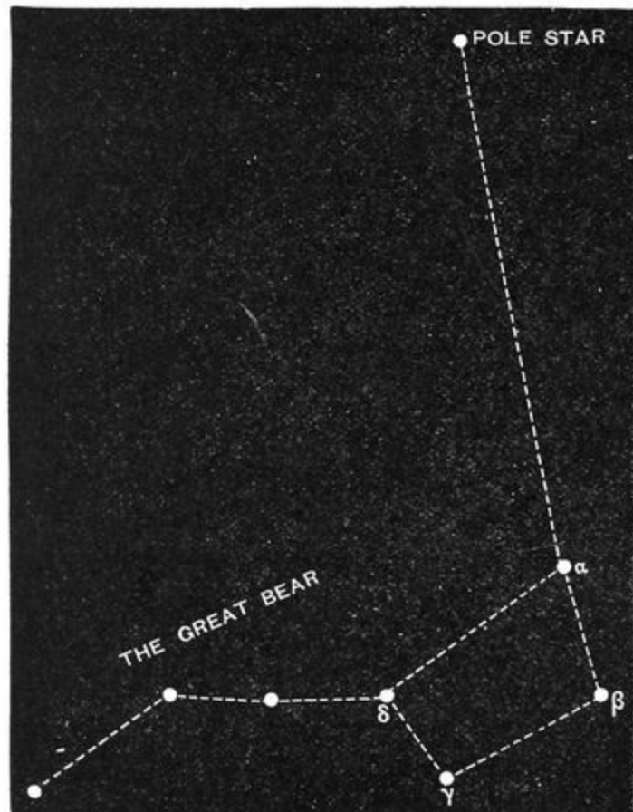
FIG. 92.—The Great Bear and the Pole Star.
