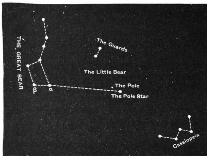
FIG. 82.—The Great Bear and the Pole.
