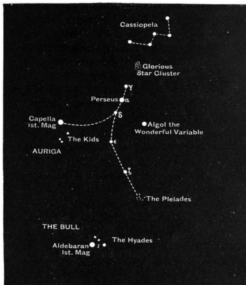
FIG. 84.—Perseus and its Neighboring Stars, including Algol.
