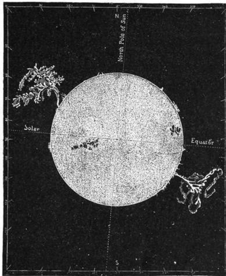
FIG. 20.—Solar Prominences ( drawn by Trouvelot ).
