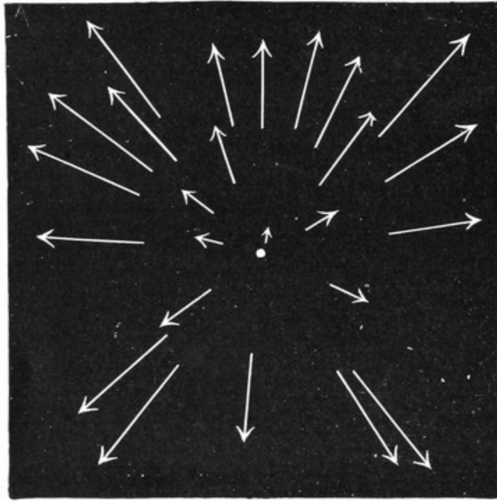
FIG. 81.—The Radiant.
