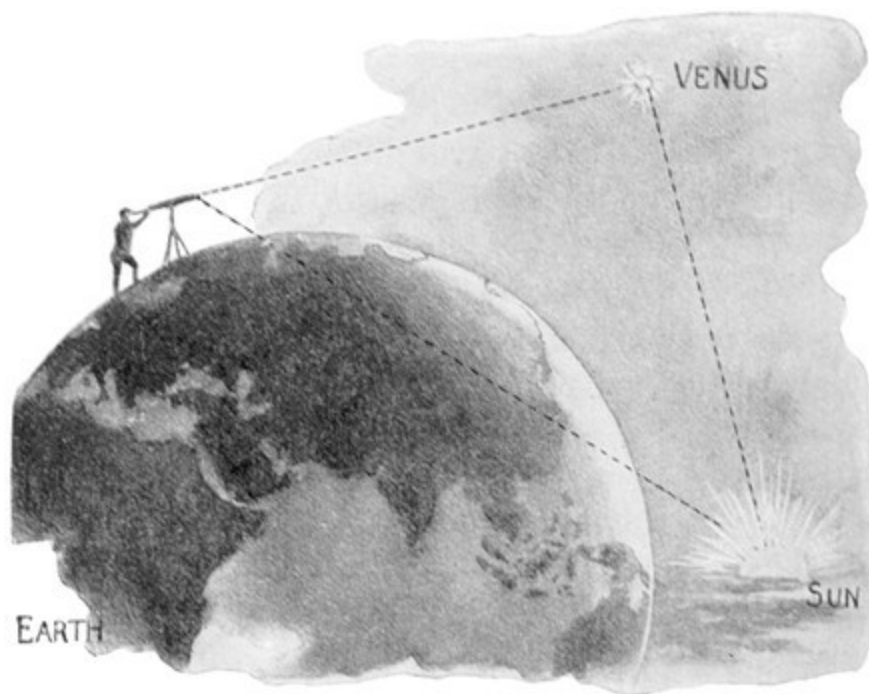
FIG. 50.—To show that Venus shines by Sunlight.
