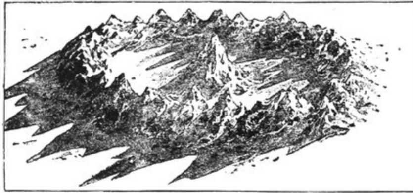
FIG. 42.—Our Model of a Lunar Crater.
