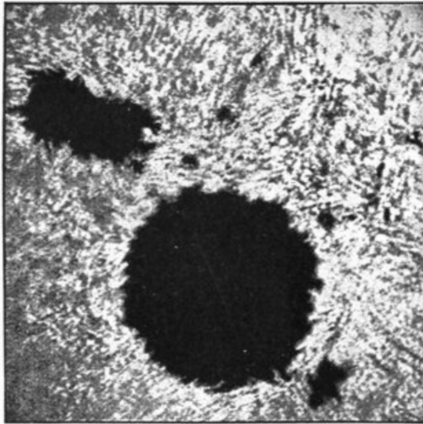
FIG. 14.—A Sun-spot ( after Janssen ).
