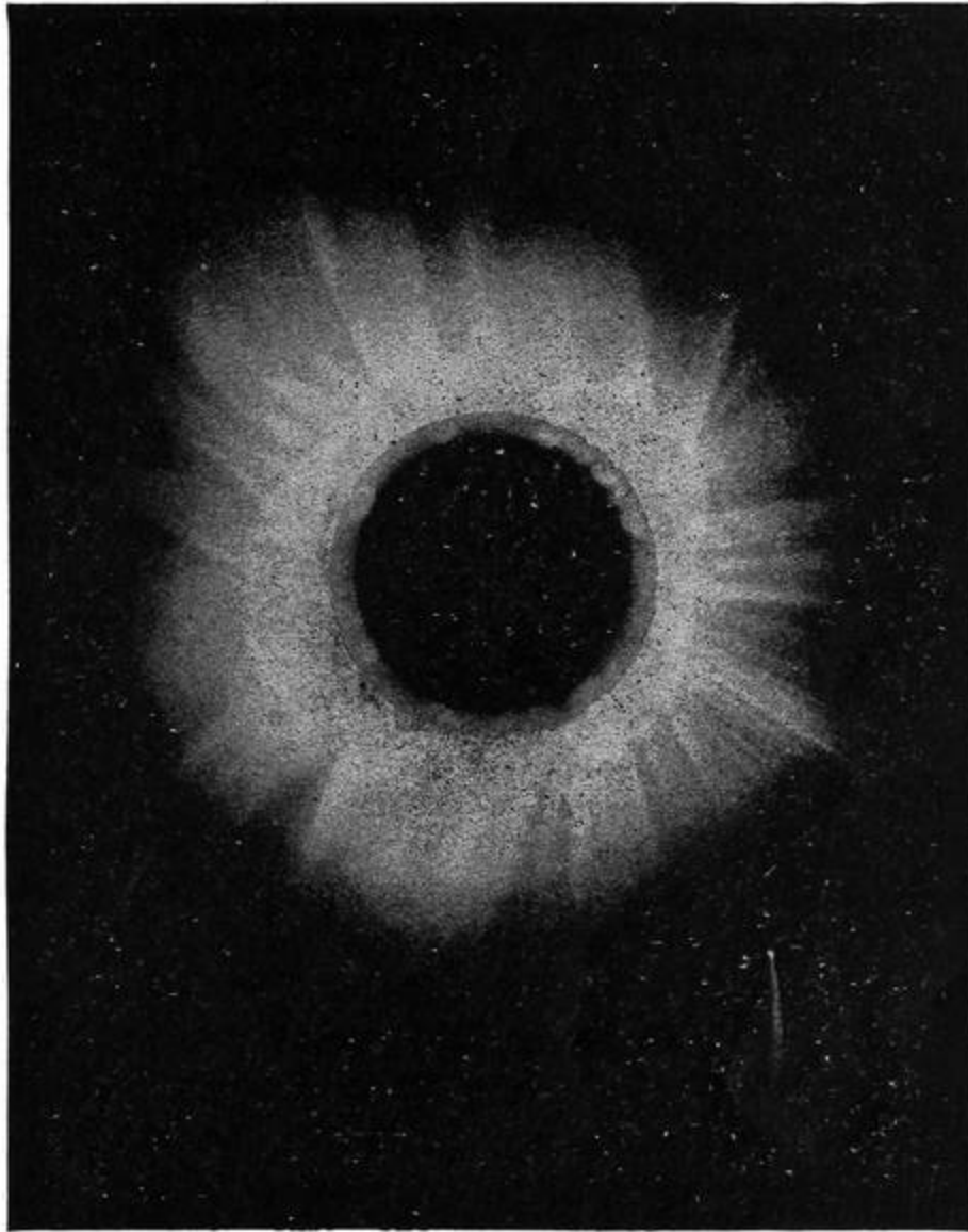
FIG. 19.—The Corona of the Sun, 1882 ( by Schuster ).
