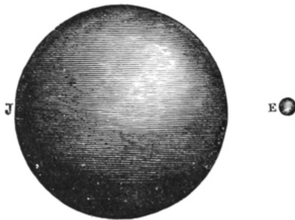
FIG. 66.—Jupiter and the Earth compared.
