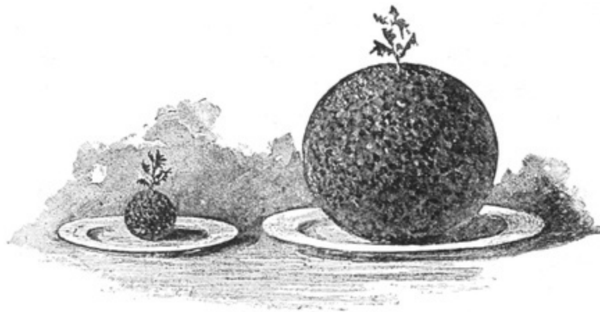
FIG. 32.—Relative Sizes of the Earth and Moon.
