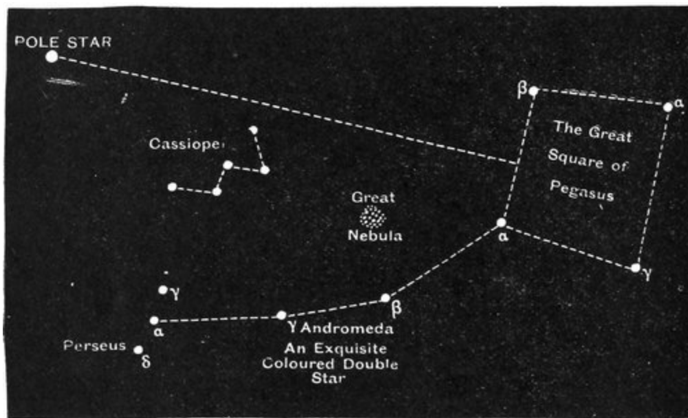
FIG. 93.—The Great Square of Pegasus.
