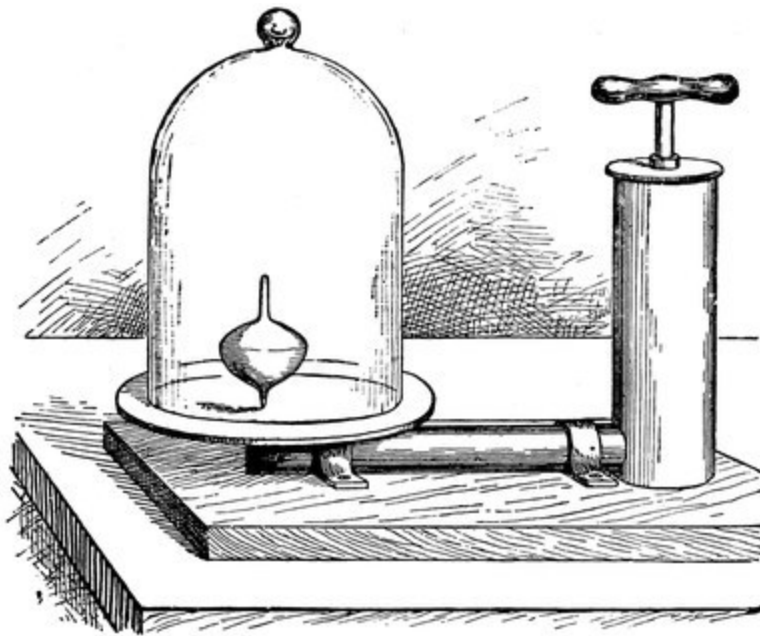
FIG. 58.—To illustrate the First Law of Motion.
