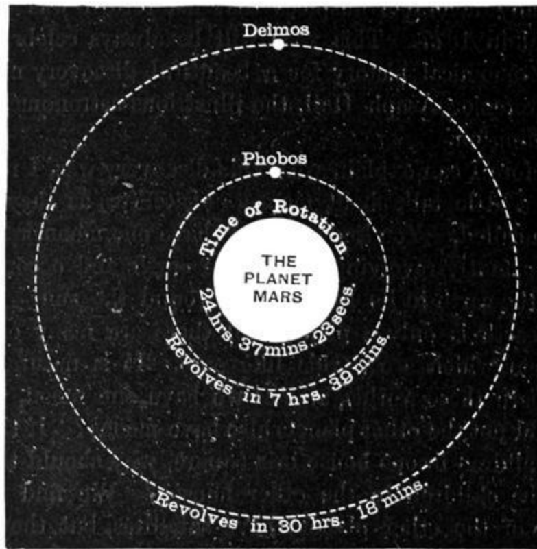
FIG. 63.—Mars and his Two Satellites.
