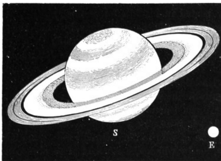
FIG. 68.—Saturn and the Earth compared.
