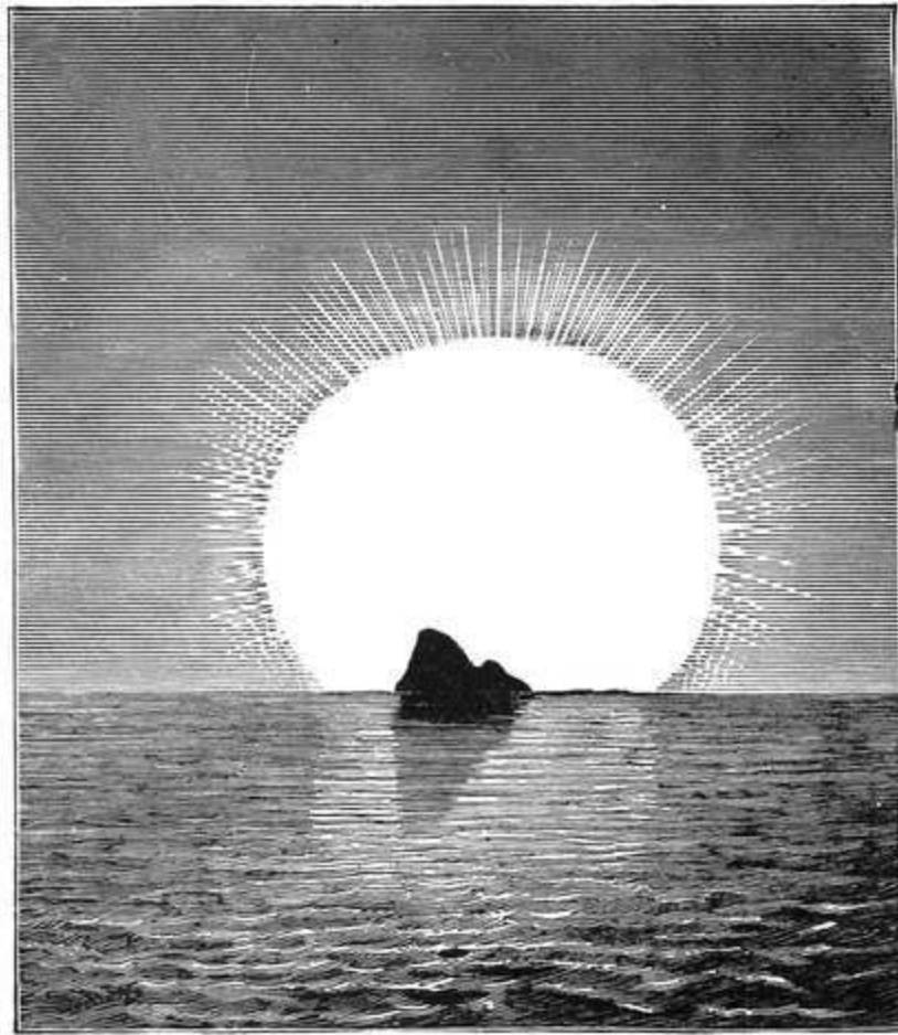
FIG. 10.—A Sunset viewed from Marseilles ( Marcus Codde ).
