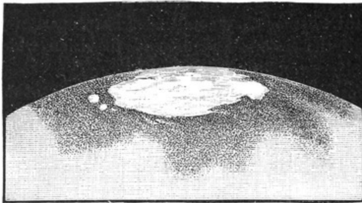
FIG. 62.—The South Pole of Mars, September, 1877 ( Green ).
