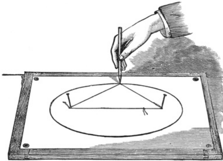
FIG. 54.—How to draw an Ellipse.
