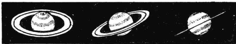
Saturn
