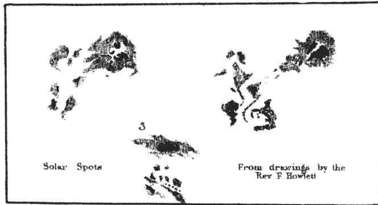
Solar Spots
