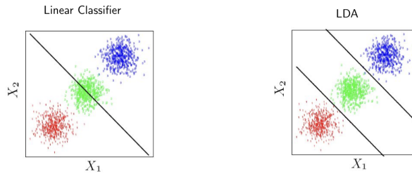
Figura 3.1: Boundary Conditions LDA.
