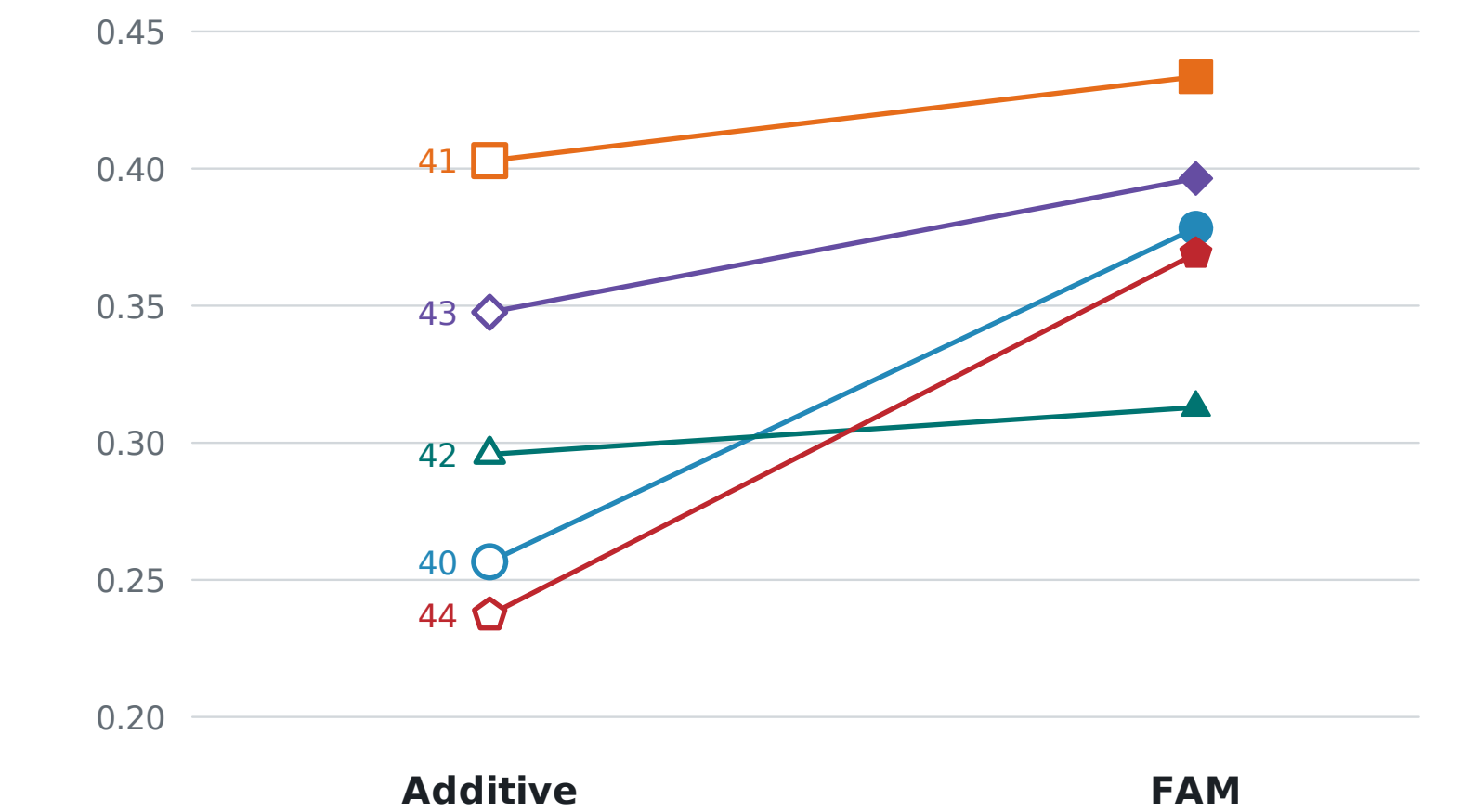
B Delta mAP@50 relative to standard FAM
