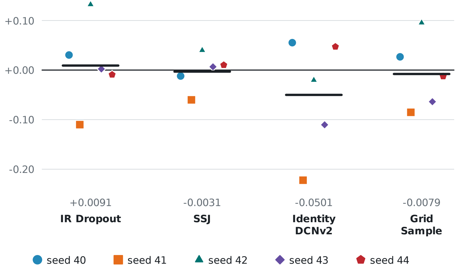
B Delta mAP@50 relative to standard FAM
