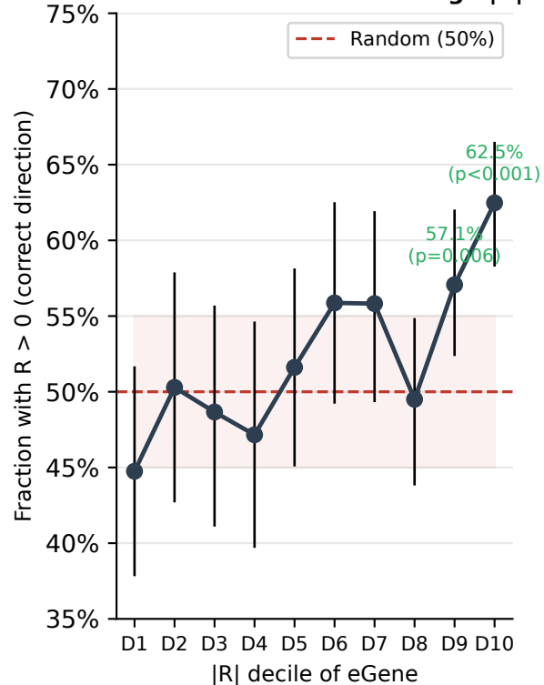
(C) Direction accuracy barely exceeds chance even at high |R|
