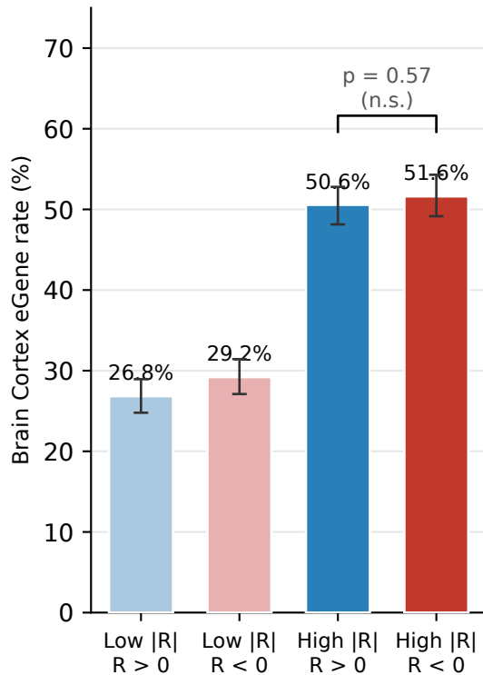
(B) Within same |R| , direction does not predict eGene status
