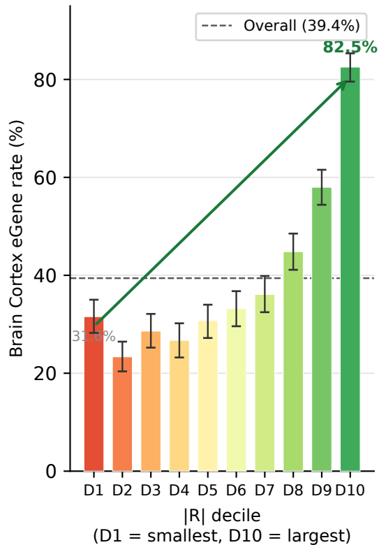
(A) |R| monotonically predicts eQTL gene status
