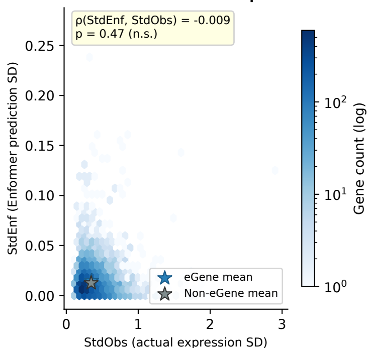
(C) Enformer prediction spread uncorrelated with actual spread
