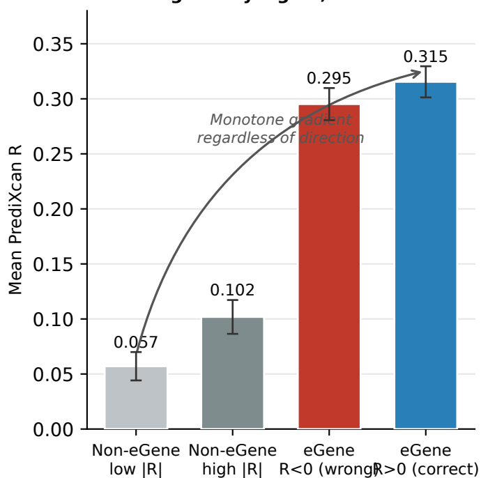
(B) PrediXcan R increases with regulatory signal, not direction
