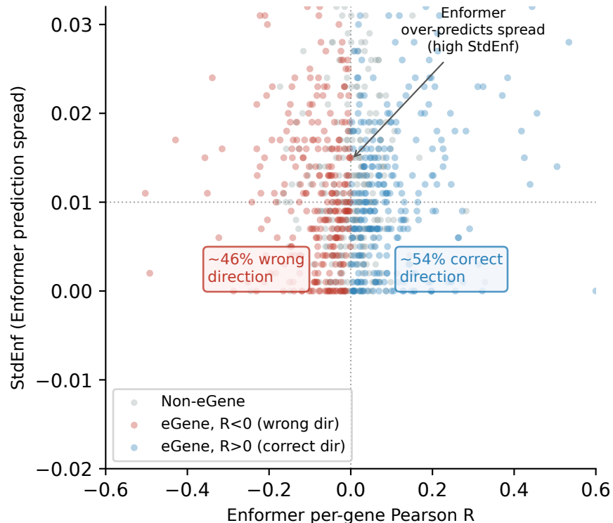
(B) eGenes span both R > 0 and R < 0 ; but have higher StdEnf (magnitude)
