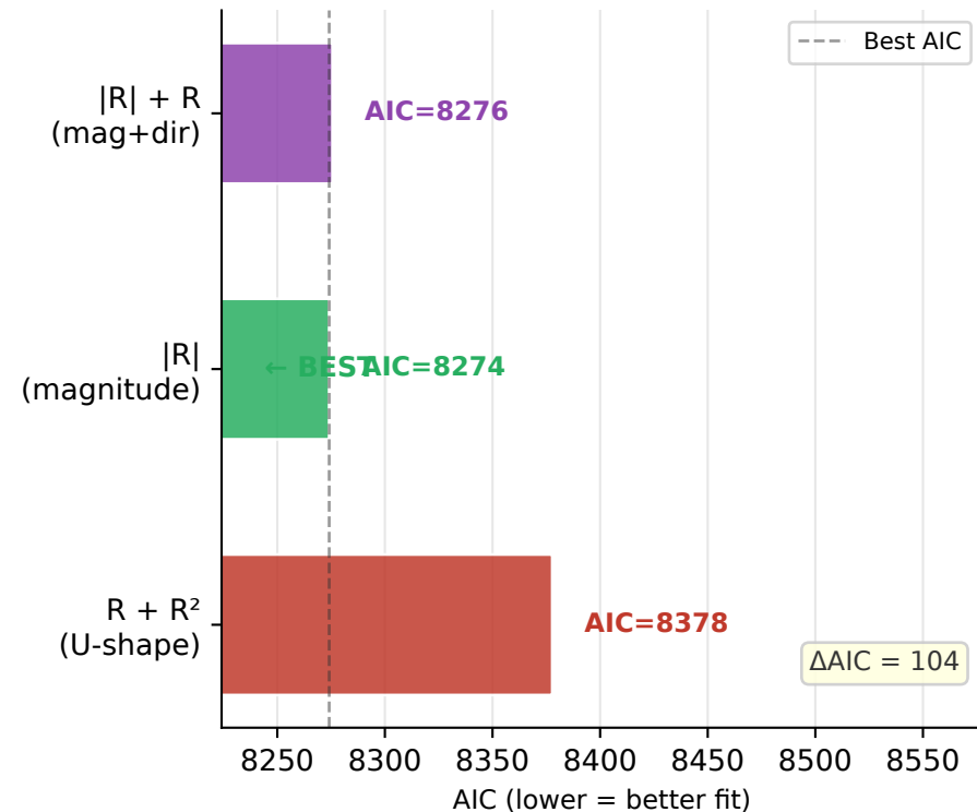
(A) |R| model fits significantly better than R + R^2 (U-shape)
