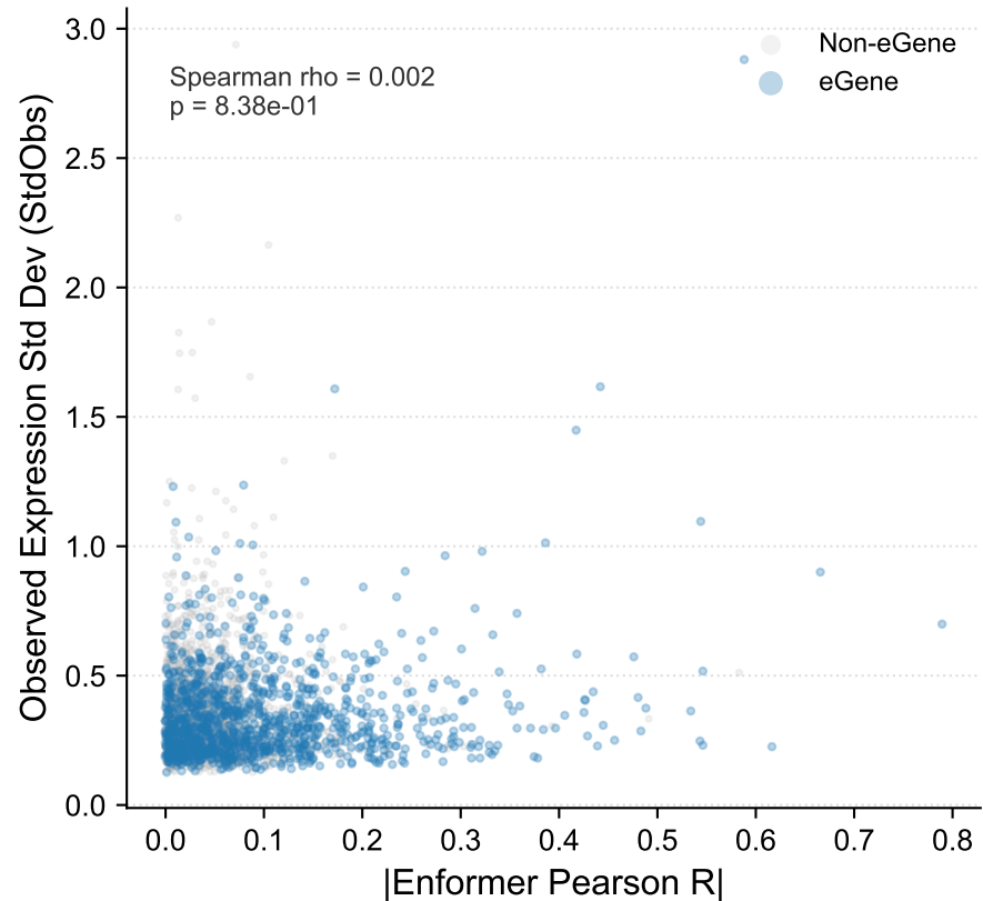
C Prediction magnitude vs. observed spread
