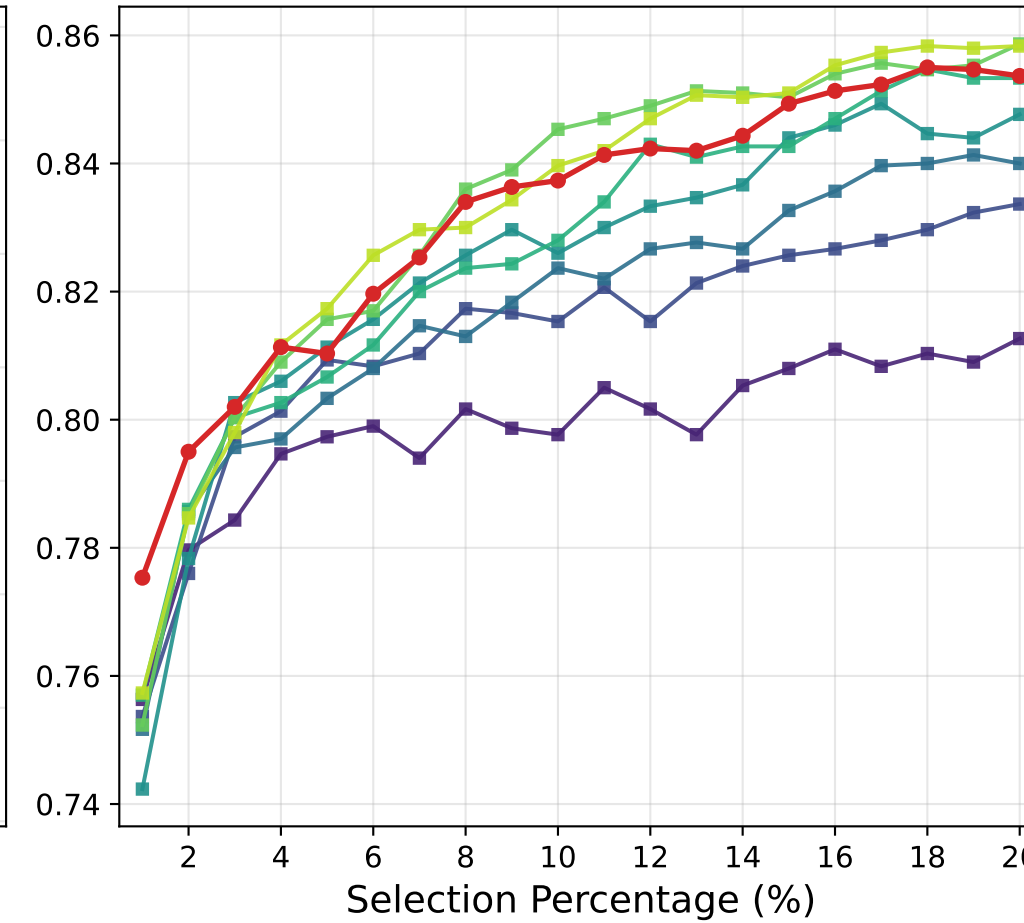
MR
