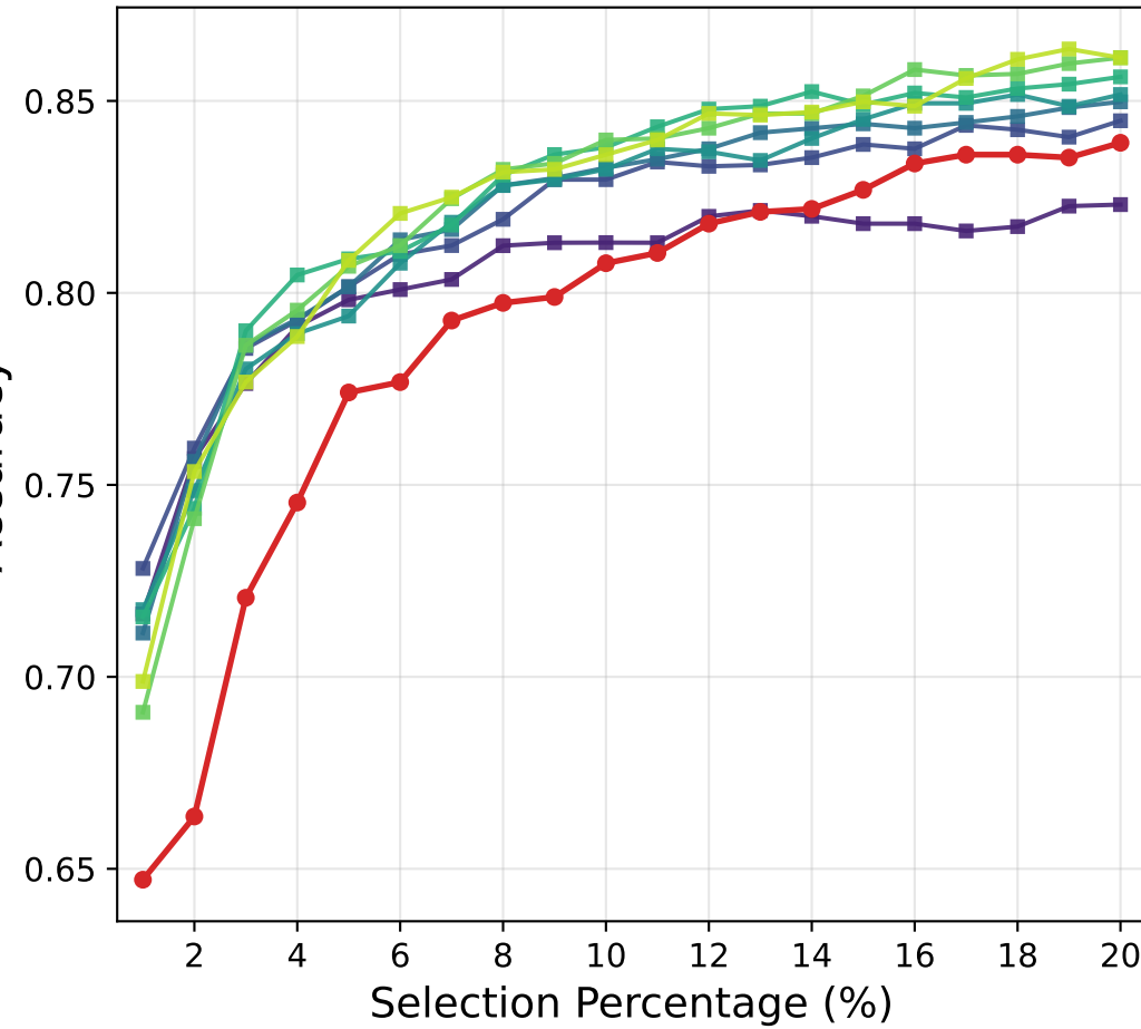
SST-2
