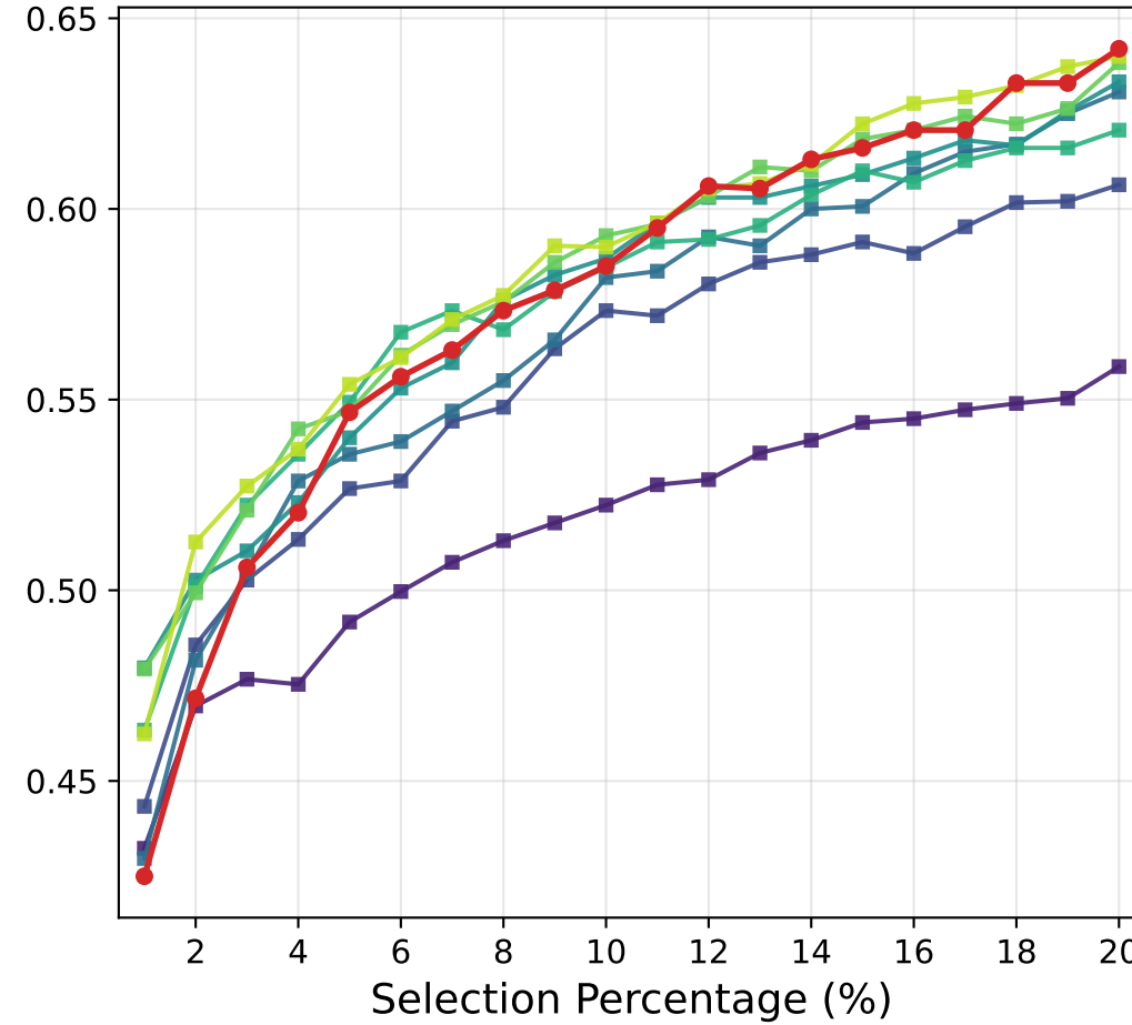
MNLI
