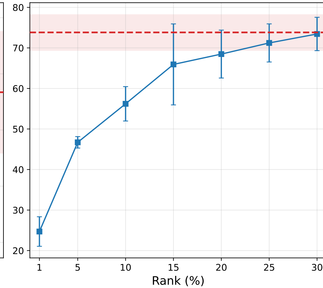
MNLI
