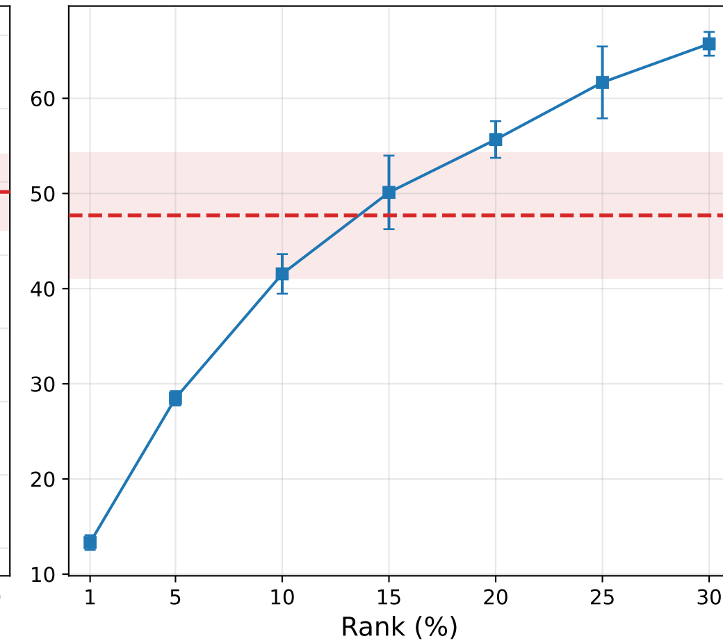
MR
