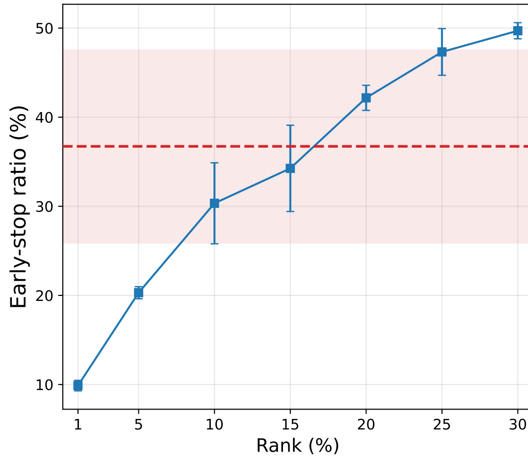
SST-2
