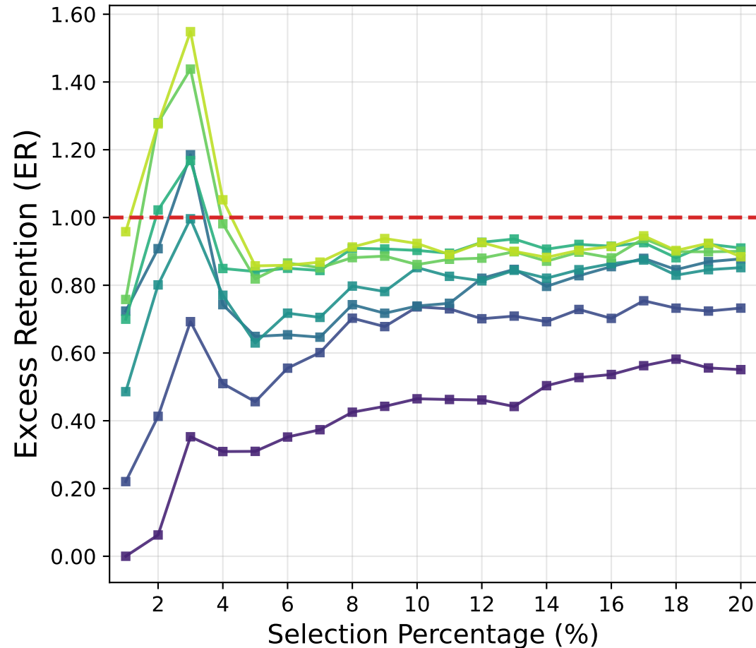
QQP ( n = 5000 )
