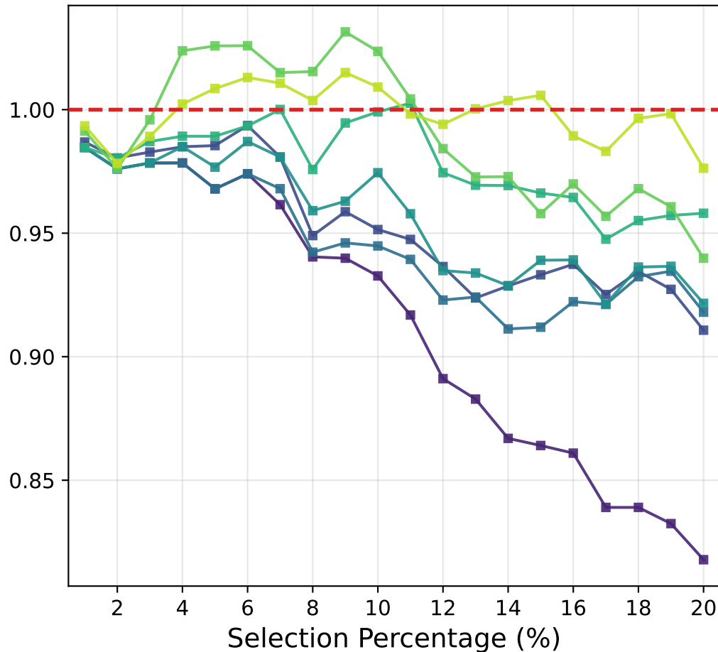
MRPC ( n = 3668 )
