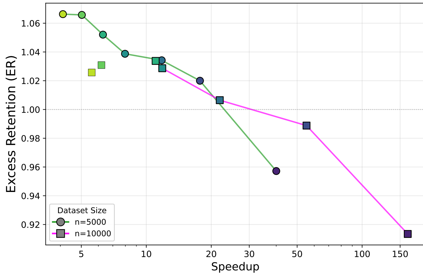
SST-2
