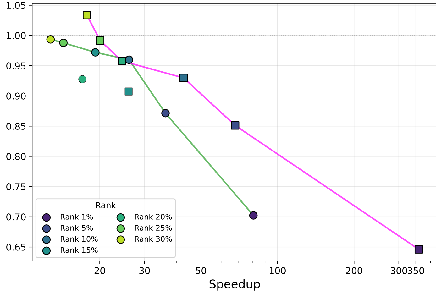
MNLI
