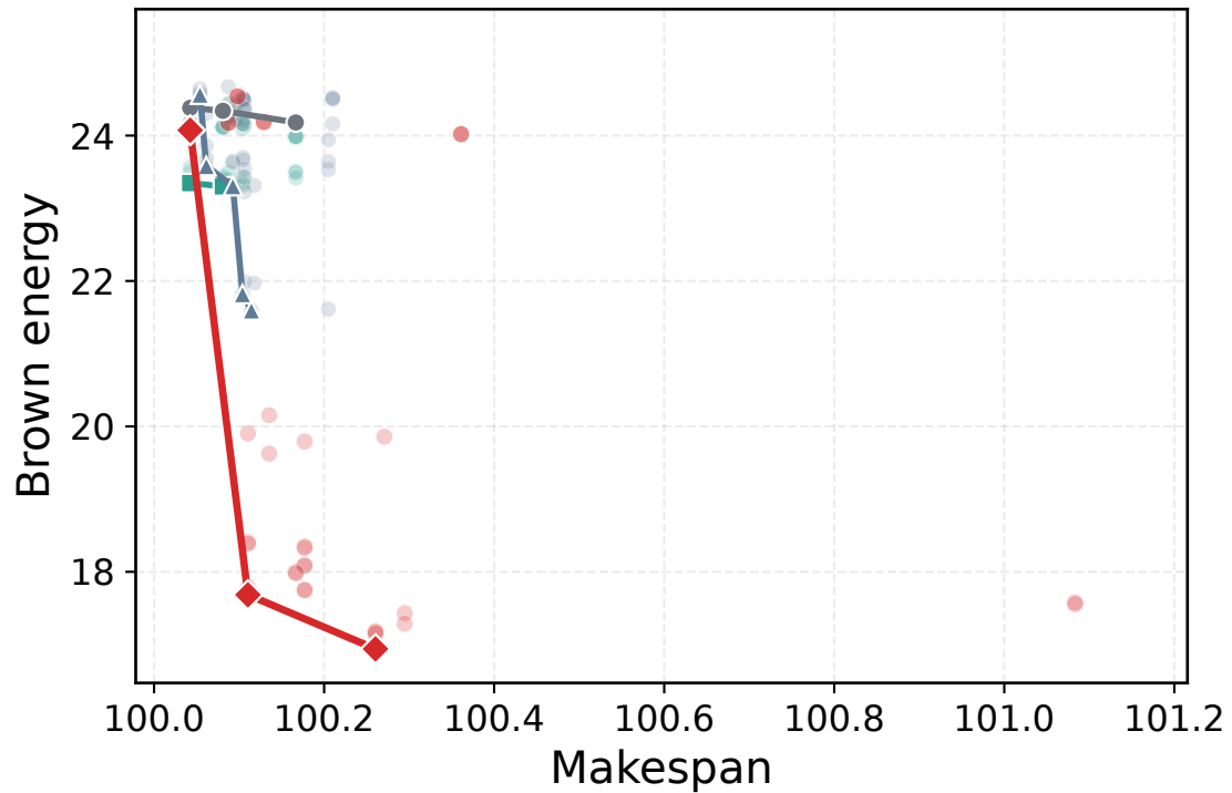
Seismology-200p
