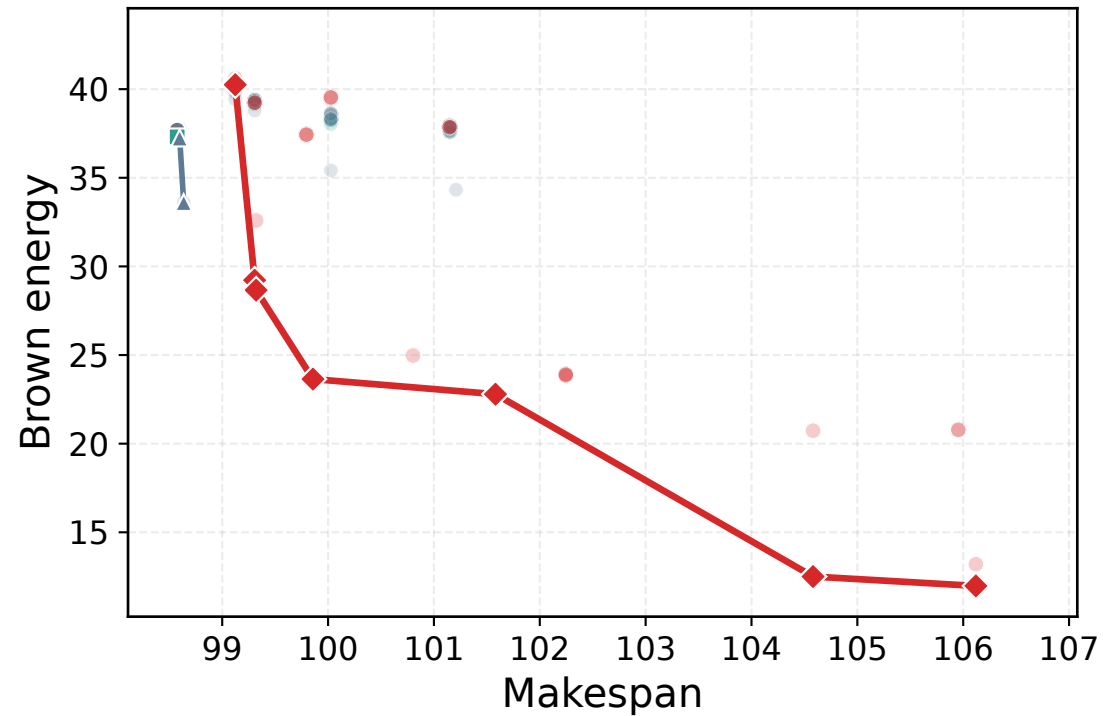
Epigenomics-100k
