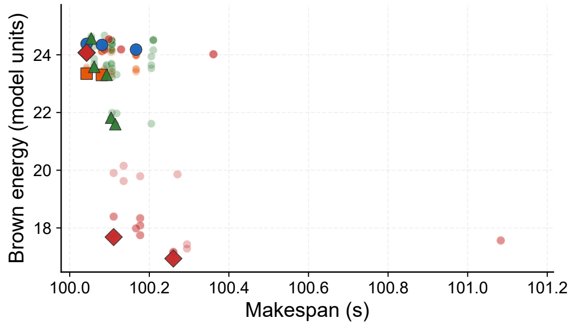
Seismology-200p
