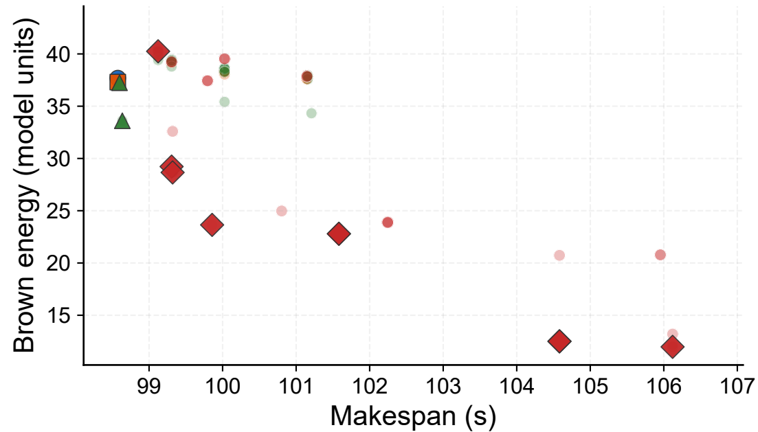
Epigenomics-100k
