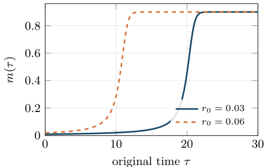
\rho = n = 3 : nonlinear escape
