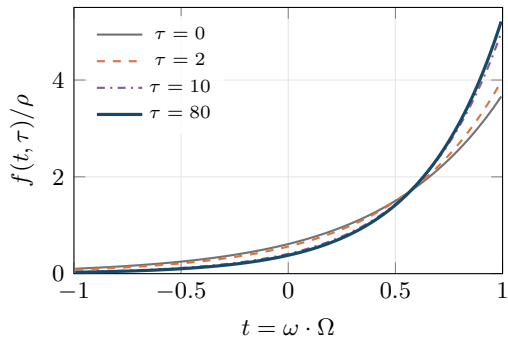
orientation profile, ordered basin
