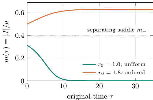
orientation profile, ordered basin
