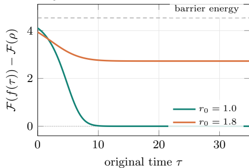
\rho = n = 3 : nonlinear escape
