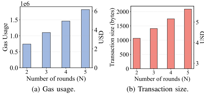
(a) Gas usage. (b) Transaction size. Fig. 14: On-chain costs of round-based HedgeSwap.
