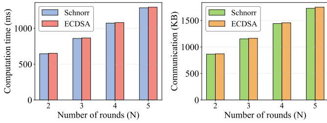
(a) Computation time. (b) Communication overhead. Fig. 13: Off-chain costs of round-based HedgeSwap.
