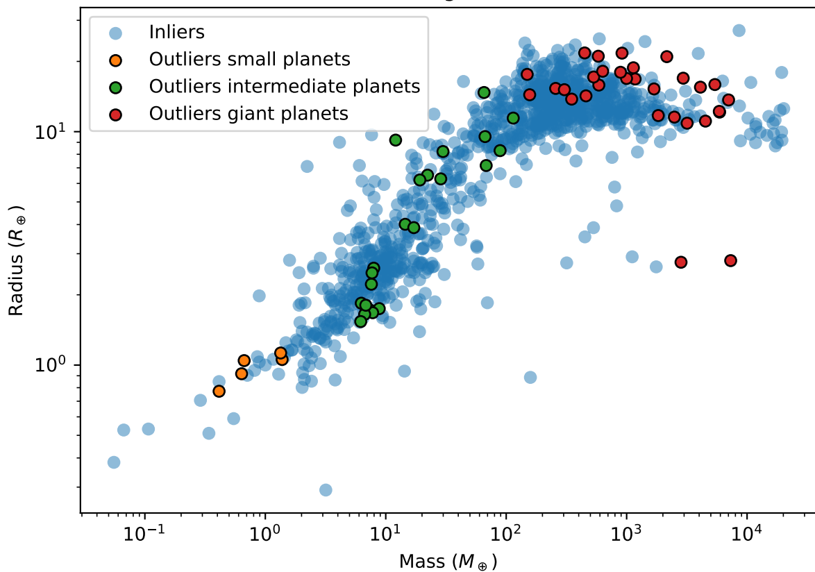
LOF Outlier Detection excluding uncertainties: Mass vs Radius
