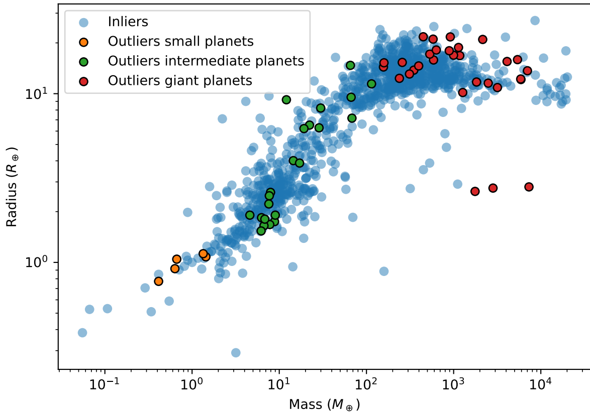
LOF Outlier Detection including uncertainties: Mass vs Radius
