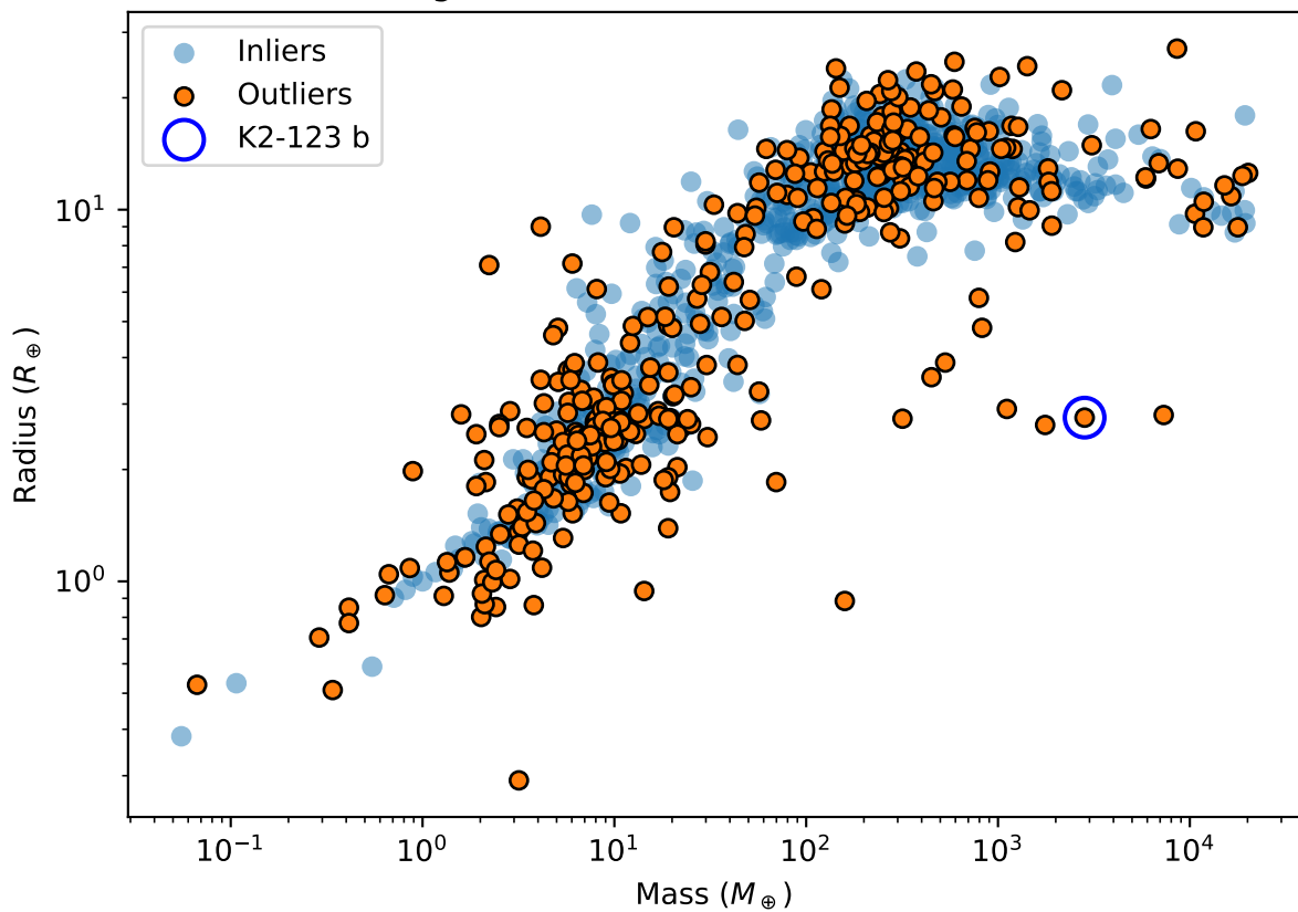
Otegi Outlier Selection: Mass vs Radius
