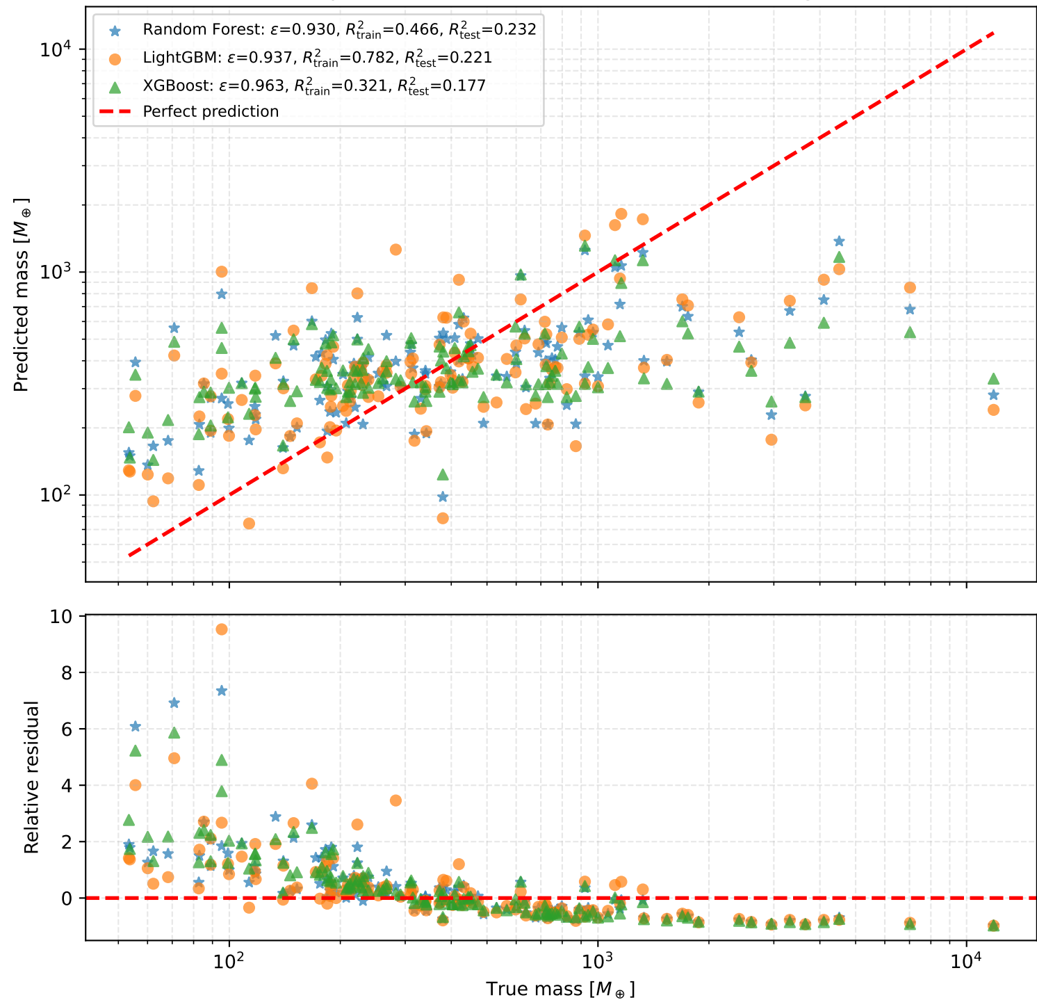
Mass Prediction Comparison on Mousavi Giant Planets; RF vs LightGBM vs XGBoost
