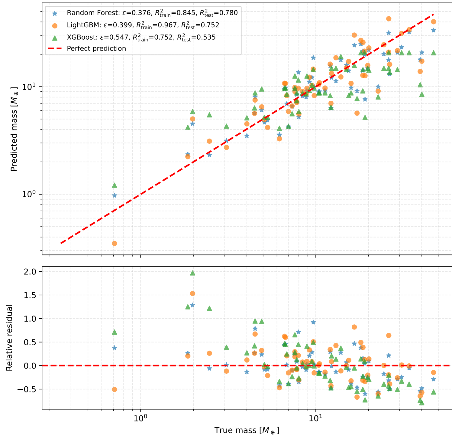
Mass Prediction Comparison on Mousavi Small Planets; RF vs LightGBM vs XGBoost
