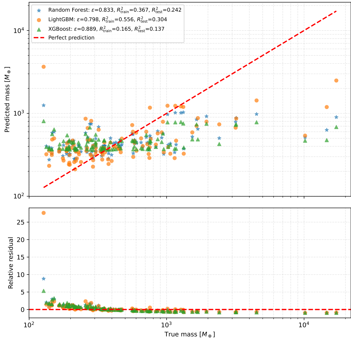
Mass Prediction Comparison on Otegi Giant Planets; RF vs LightGBM vs XGBoost
