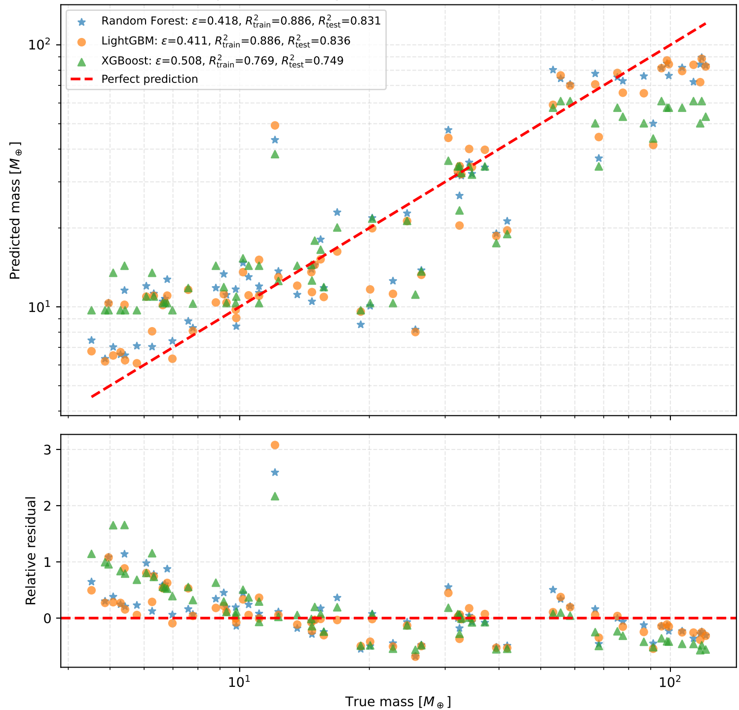
Mass Prediction Comparison on Otegi Intermediate Planets; RF vs LightGBM vs XGBoost
