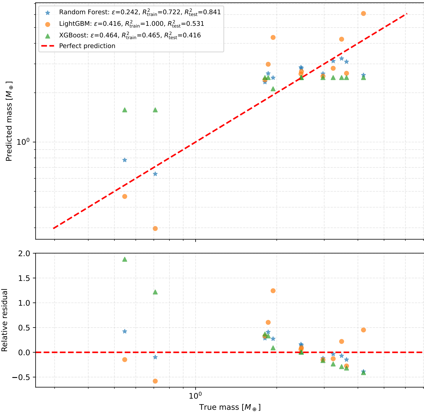
Mass Prediction Comparison on Otegi Small Planets; RF vs LightGBM vs XGBoost
