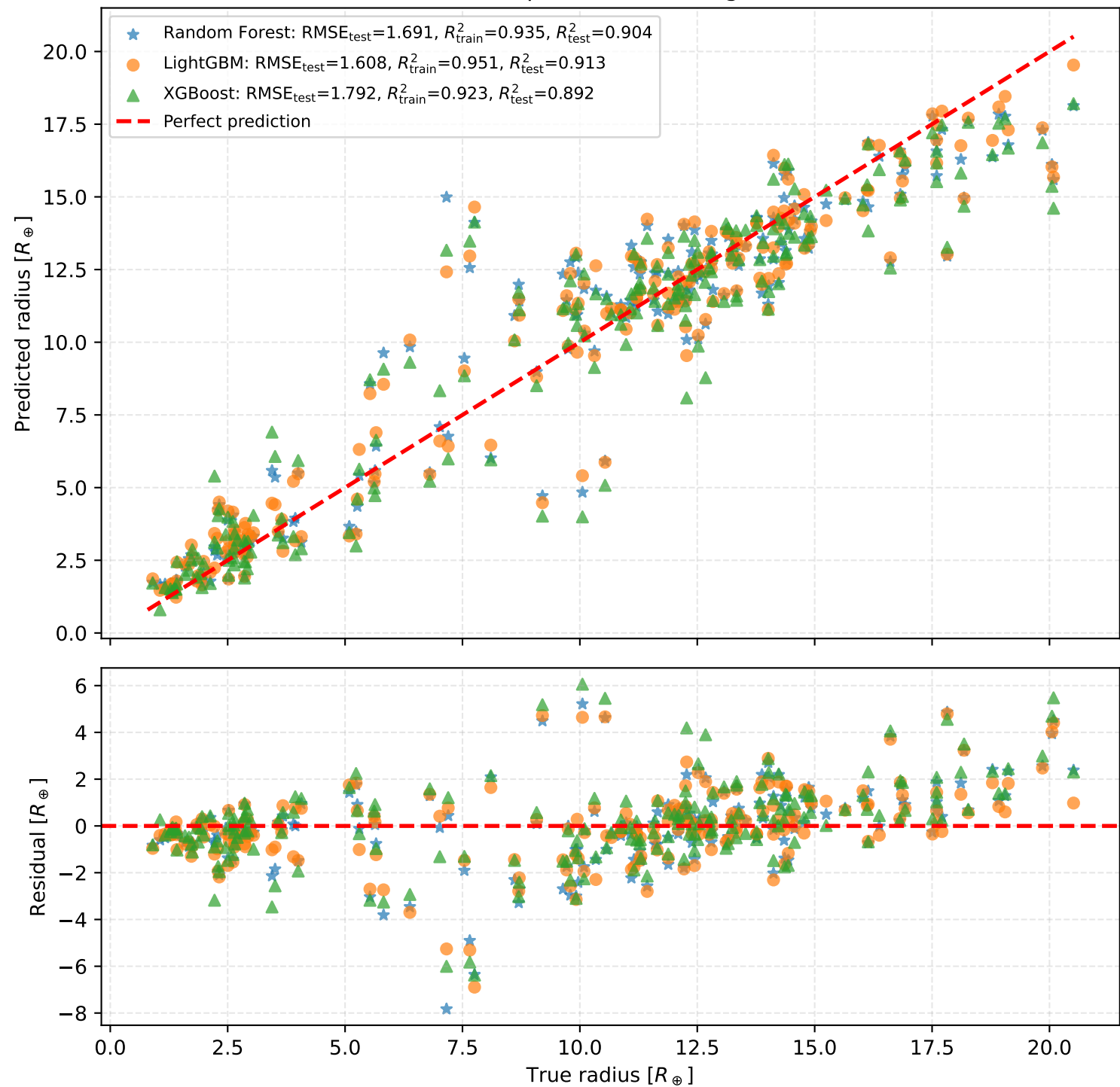
Radius Prediction Comparison: RF vs LightGBM vs XGBoost
