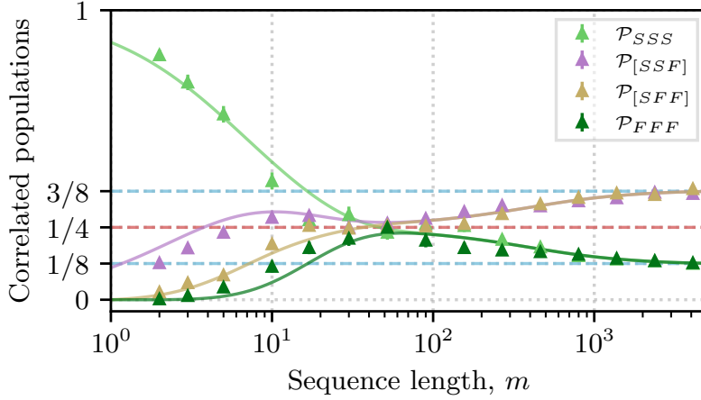
Figure 1.14: Experimental data and analytic fit for 3-qubits subject to correlated random-unitary single-qubit noise injected via random phase jitter ( \sigma_\phi = 0.06 turns).
