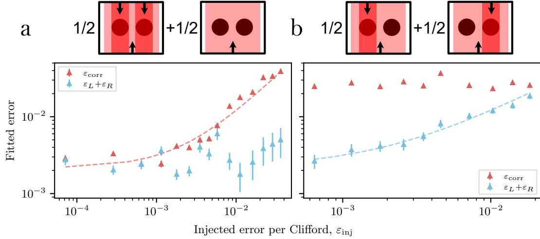
Figure 1.13: Correlated and uncorrelated errors are injected via a single-addressed Stark-shift beam, and quantified through fitting the correlated success populations. The four addressing configurations are depicted visually above the plot. The wide beam signifies the on-resonance global drive which executes the parallel single-qubit rotations, while the narrow beams represent the off-resonant Stark shift beams addressing single-qubits (black circles). In (a) the errors are correlated between qubits, while panel (b) shows the extracted errors after independent errors are injected. Error bars are the extracted standard deviations from a non-linear Levenberg–Marquardt fit of the underlying correlated populations.
