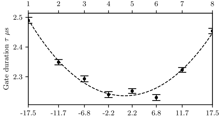
Figure 1.15: Variation of \pi -pulse gate duration along eight ion chain due to global beam Gaussian profile.
