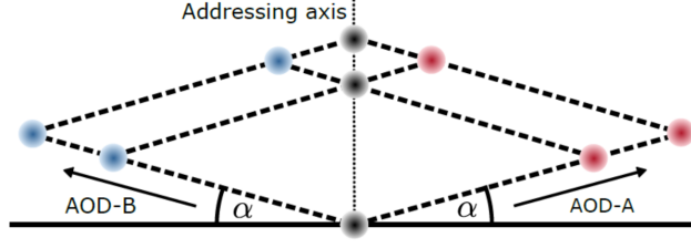
Figure 3.13: Spots generated by cAOD with wedge angle \alpha , when supplying two frequencies to each AOD. The black points have no over-all frequency shift, and are aligned to the ion-chain. This schematic is reproduced with permission from I. R. Overgaard transfer of status [58].
